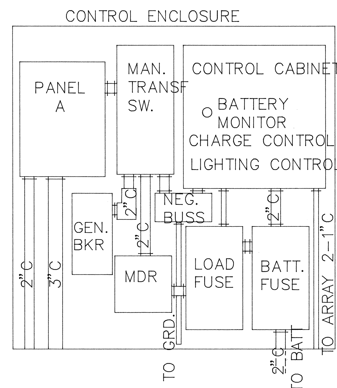
CONTROL ENCLOSURE ELEVATION SCALE: 1" = 1'-0"
