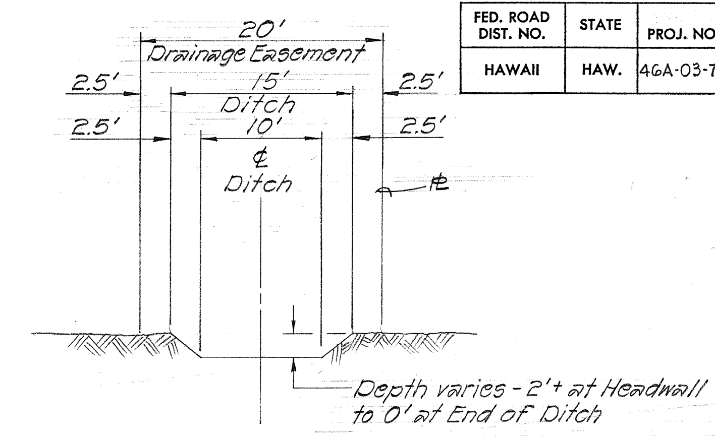
TYPICAL SECTION OF DITCH Scale: 1/8"=1'-0"
