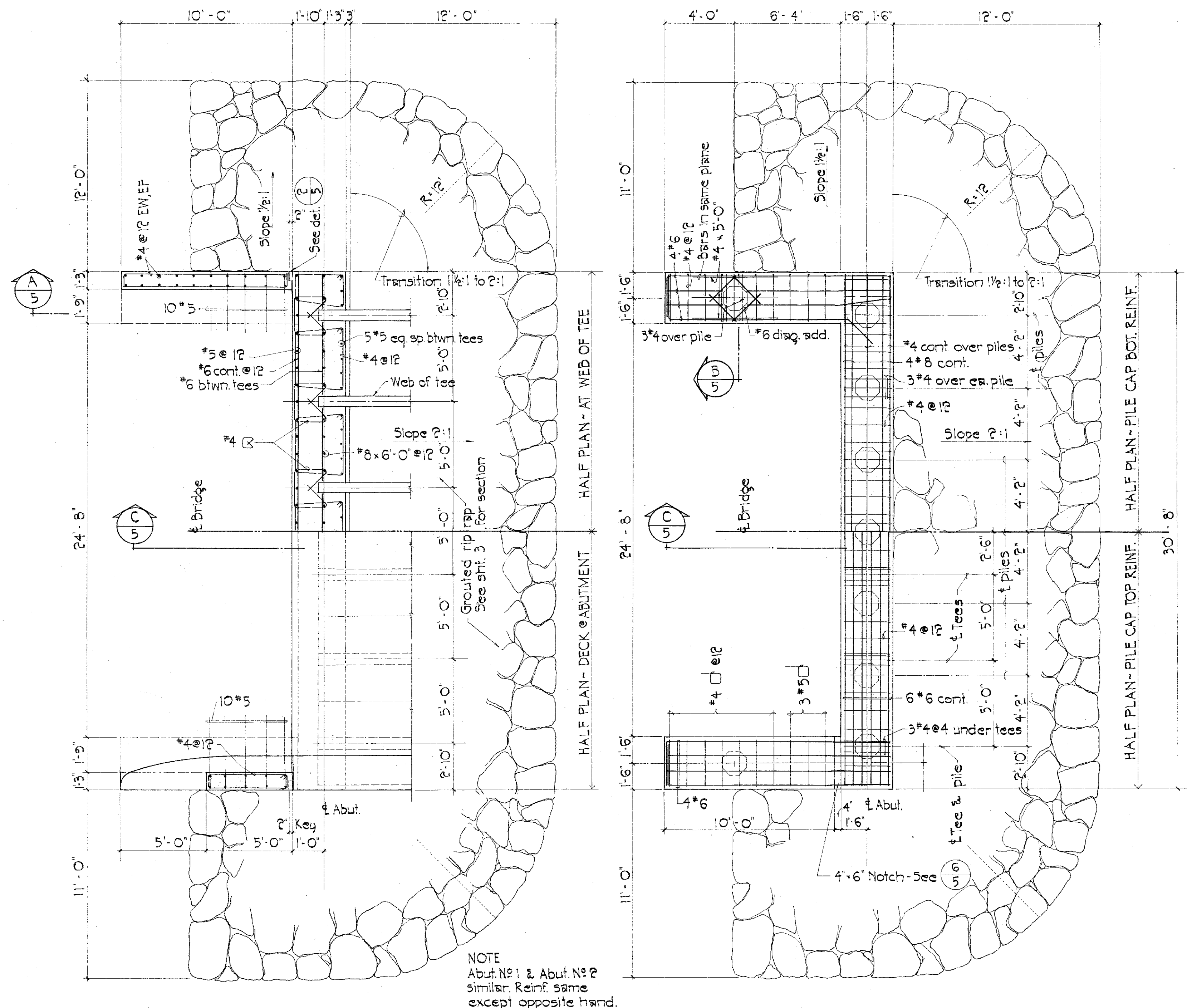
PARTIAL PLAN SECTIONS OF ABUTMENT Scale: 1/4" = 1'-0"
