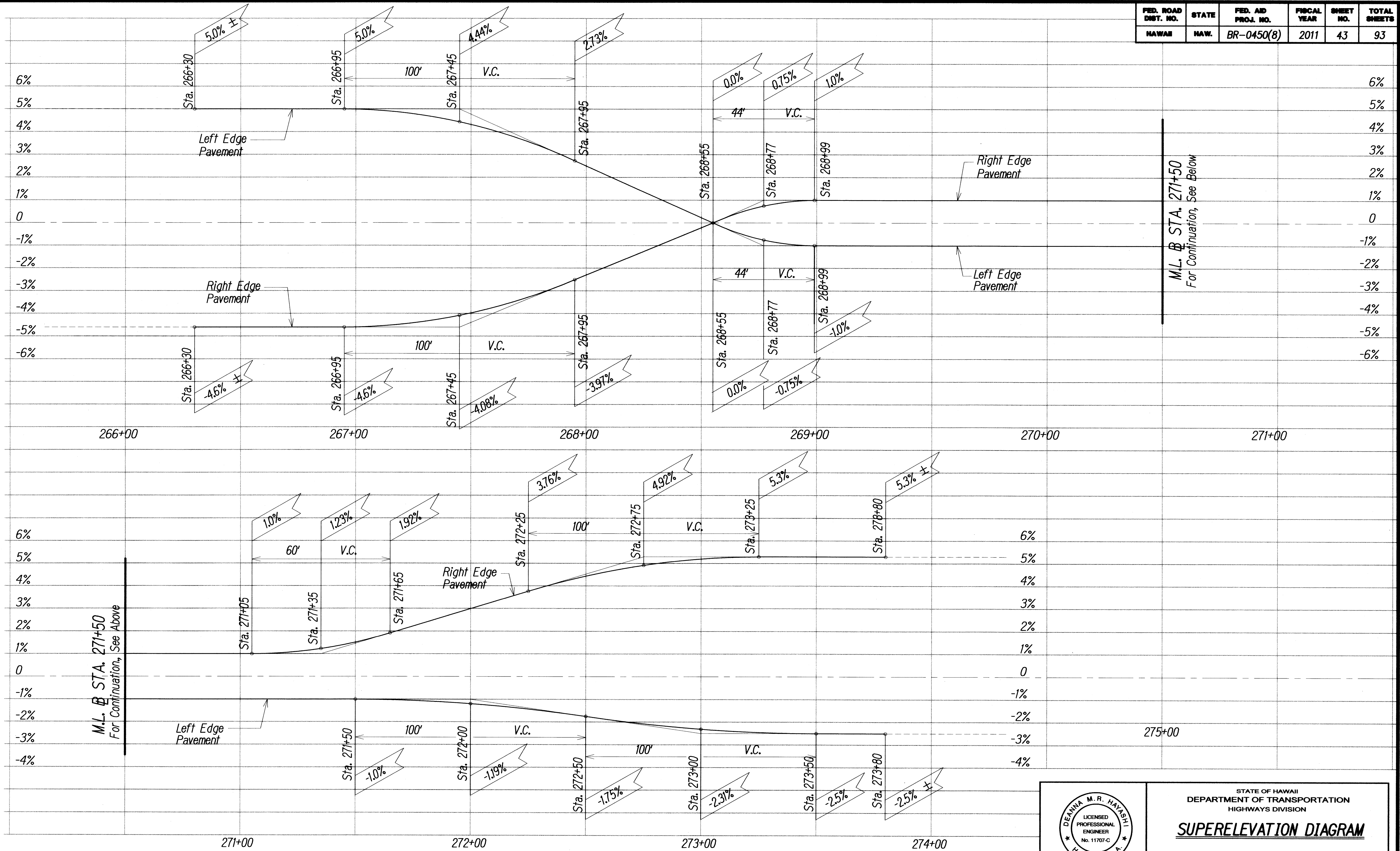
SUPERELEVATION DIAGRAM-KAM. V HWY. SCALE: HORIZ. 1" = 20' VERT. 1" = 2'
