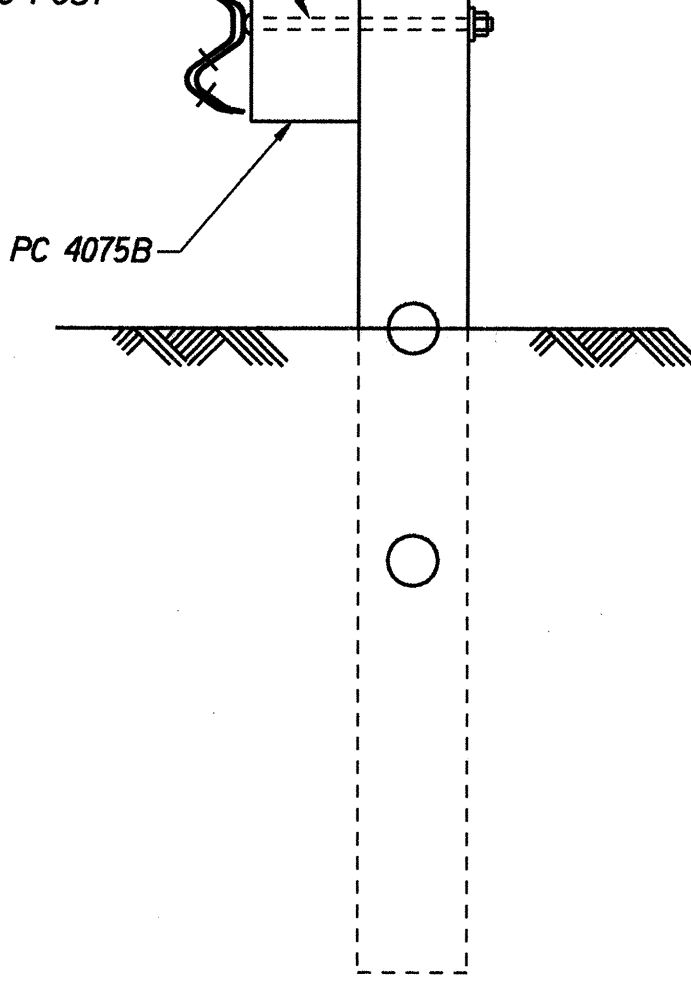
SECTION "B-B" (at POSTS #3 & #7)
