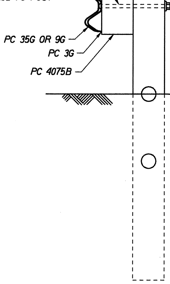
SECTION "C-C" (at POSTS #4, #6, #8, #9 & #10)
