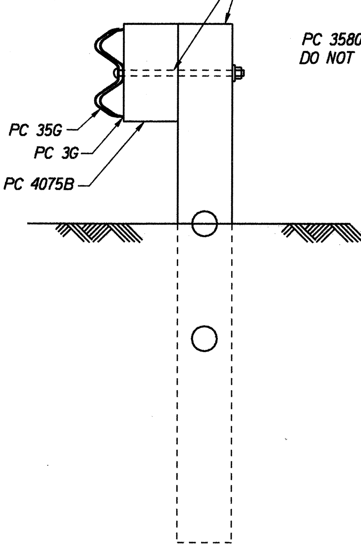
SECTION "D-D" (at POST #5)
