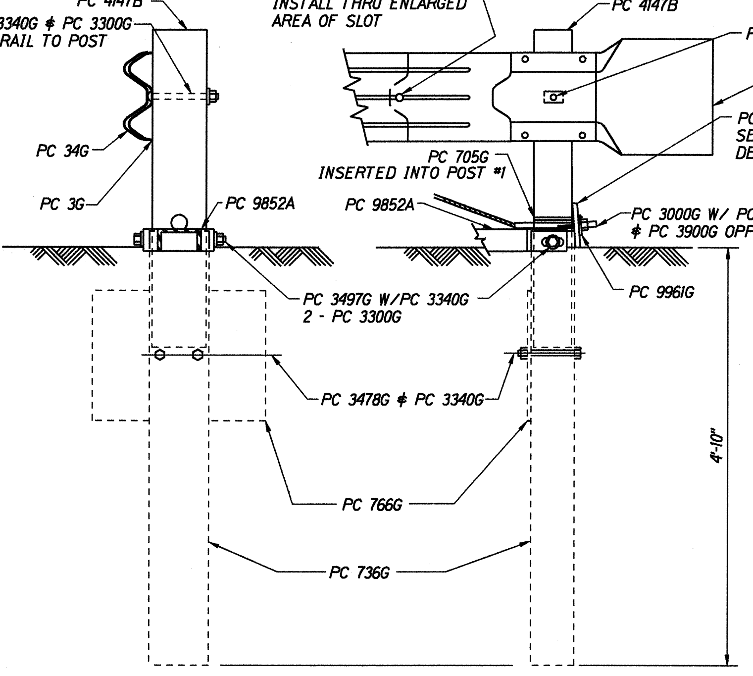
SECTION "A-A" (at POST #2)
