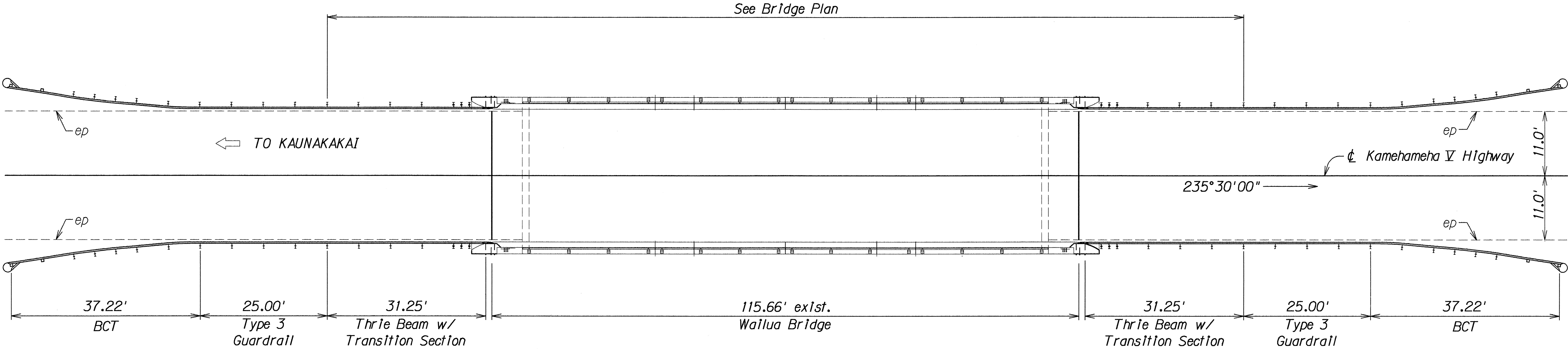
PLAN GUARDRAIL LAYOUT WAILUA BRIDGE Scale: 1"=10'
