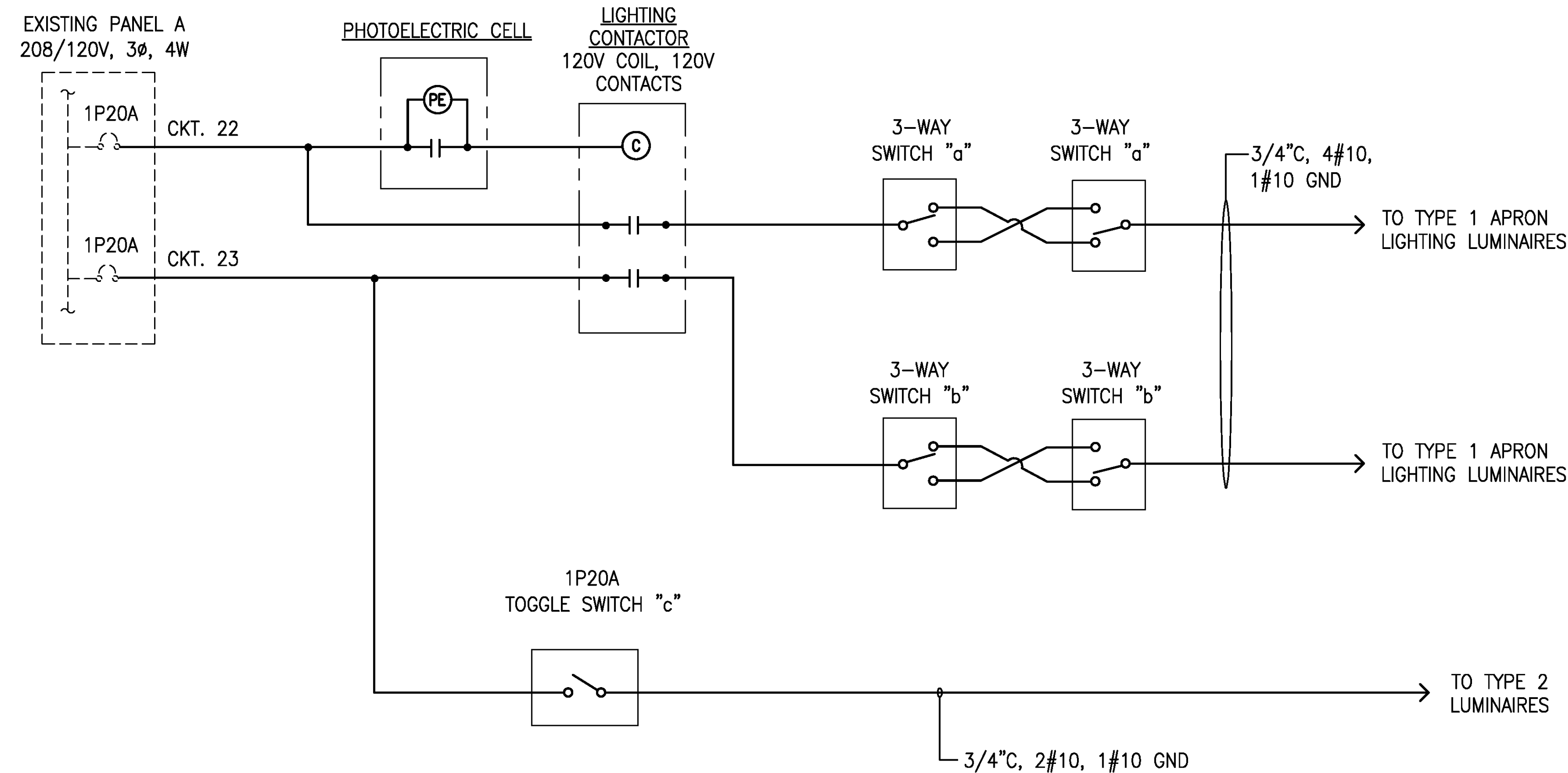
1 APRON LIGHTING CONTROL DIAGRAM E-7 NOT TO SCALE
