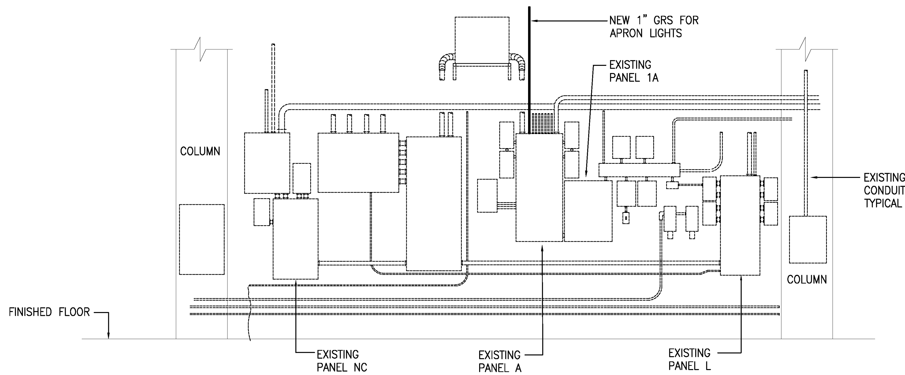
3 EQUIPMENT ELEVATION E-7 NOT TO SCALE
