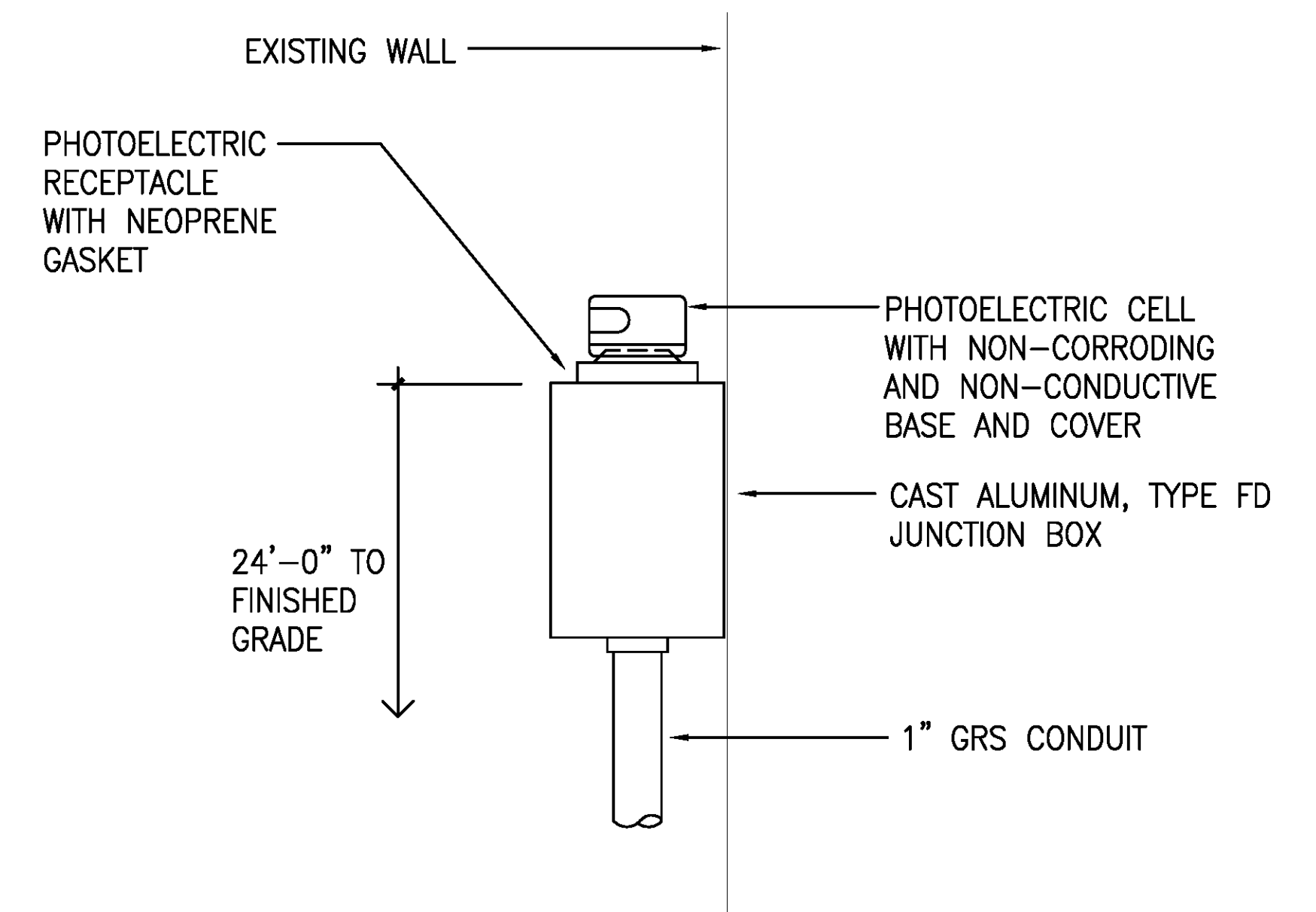
2 PHOTOELECTRIC CELL DETAIL E-7 NOT TO SCALE
