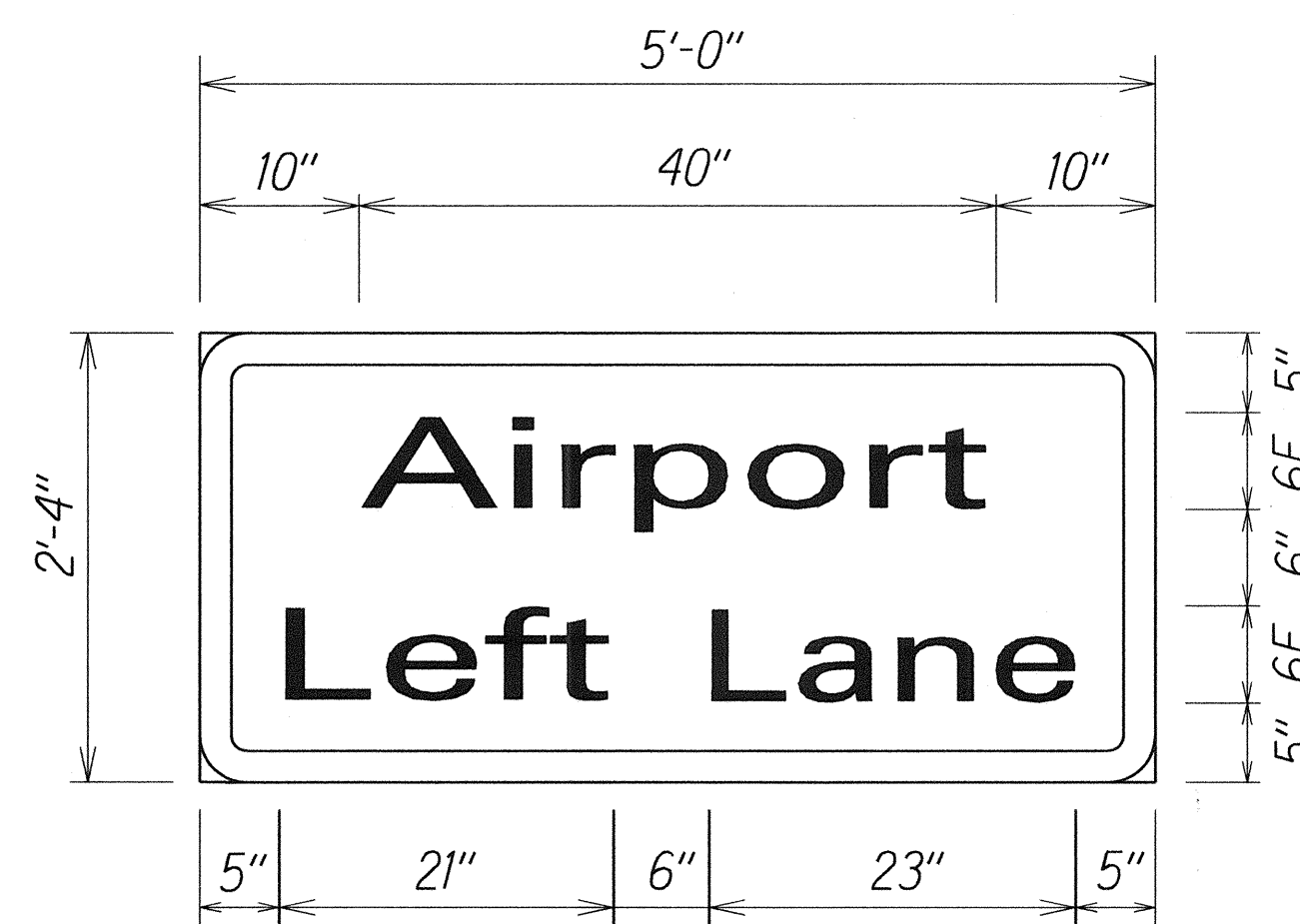
DESTINATION SIGN (D-2) Scale: 1" = 1'-0"
