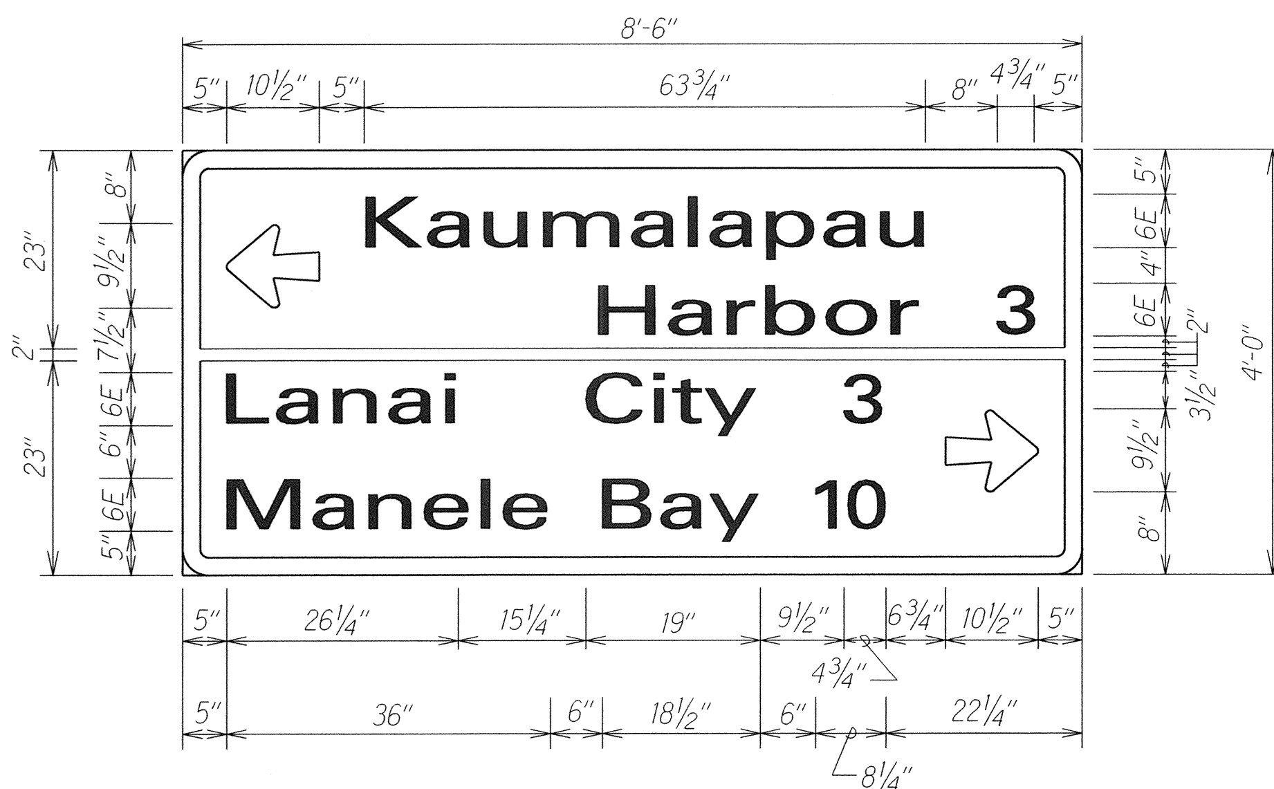
DESTINATION SIGN (D-1) Not to Scale
