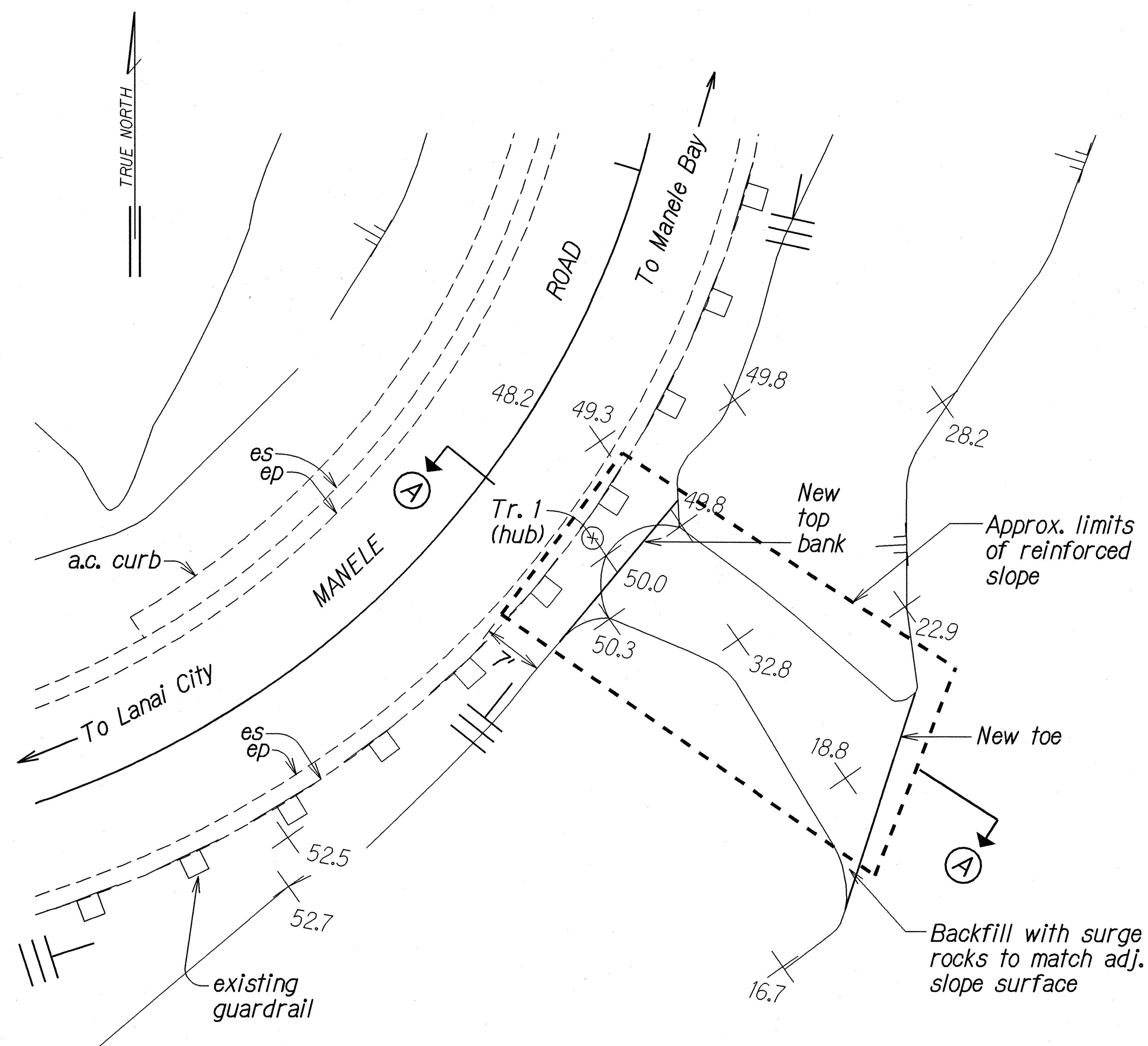
PLAN @ REINFORCED SLOPE Scale: 1" = 10'
