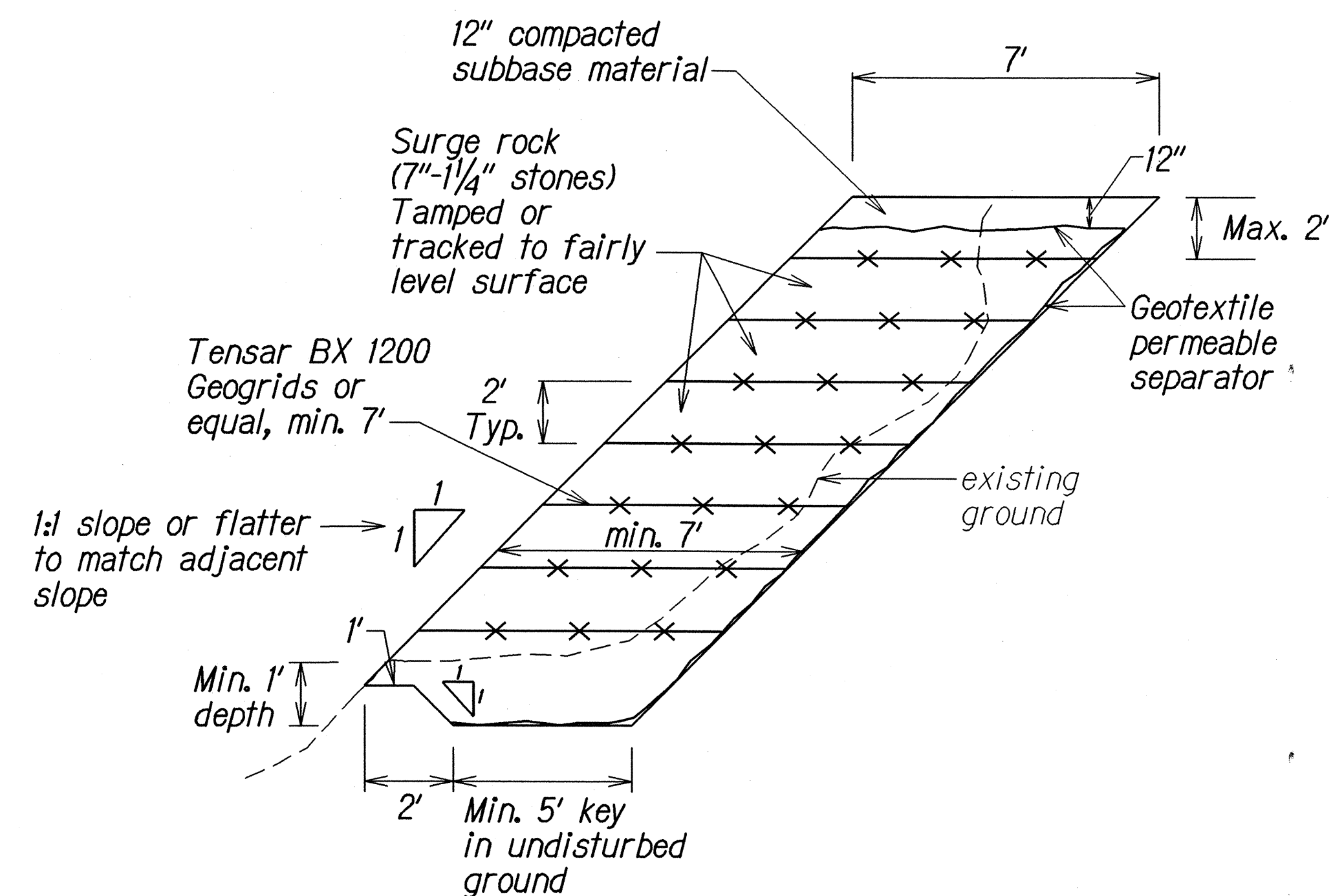
SECTION A-A TYPICAL DETAILS - REINFORCED SLOPE Not To Scale
