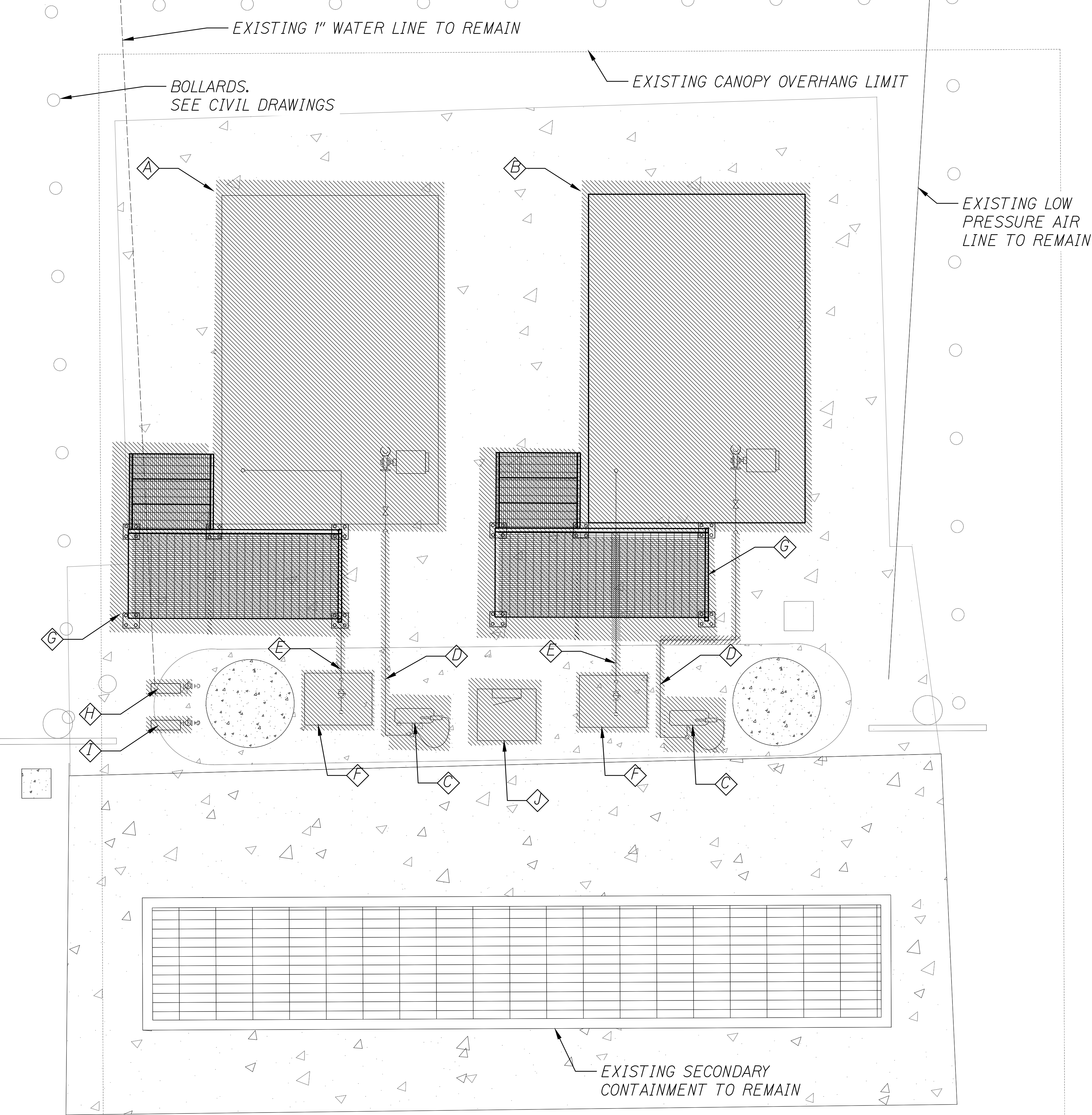
MECHANICAL DEMOLITION PLAN SCALE: 1/2" = 1'
