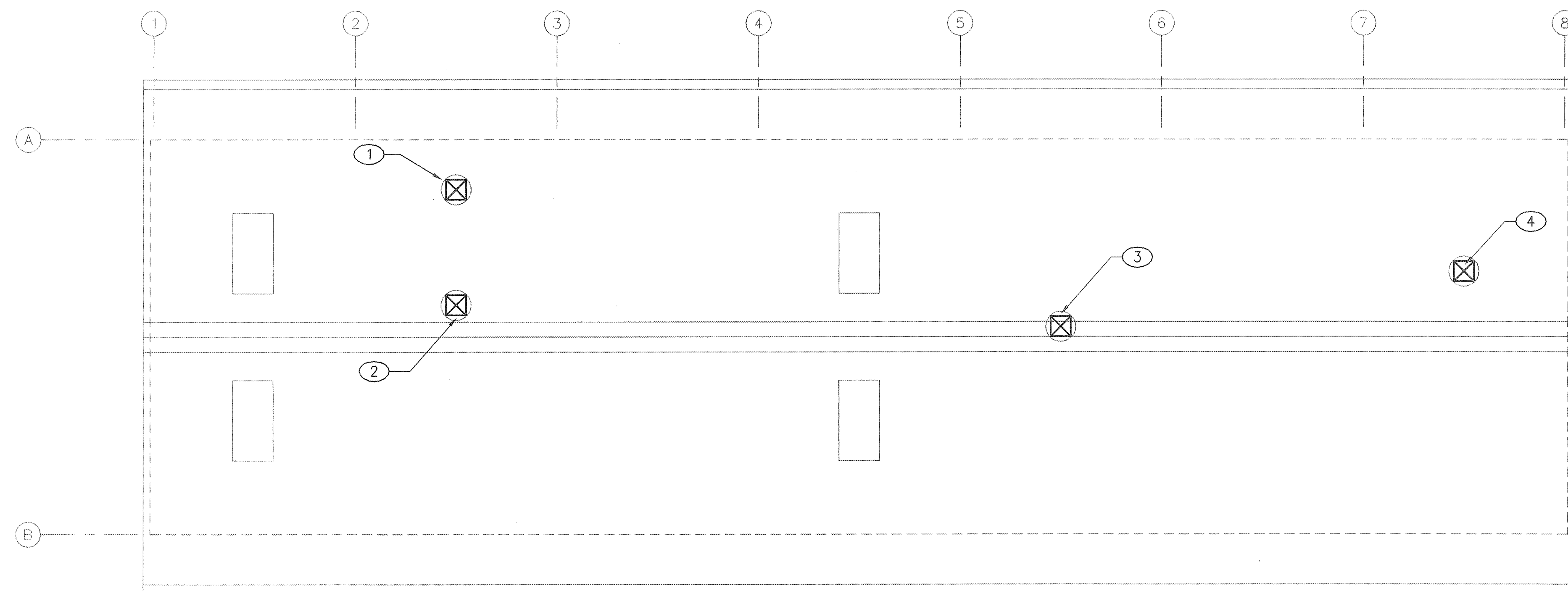
1 EXISTING MAINTENANCE OFFICE AND SHOP BLDG MECHANICAL FLOOR PLAN 8' 4' 0' 4' 8' 16' 32' SCALE: 1/8"=1'-0"
