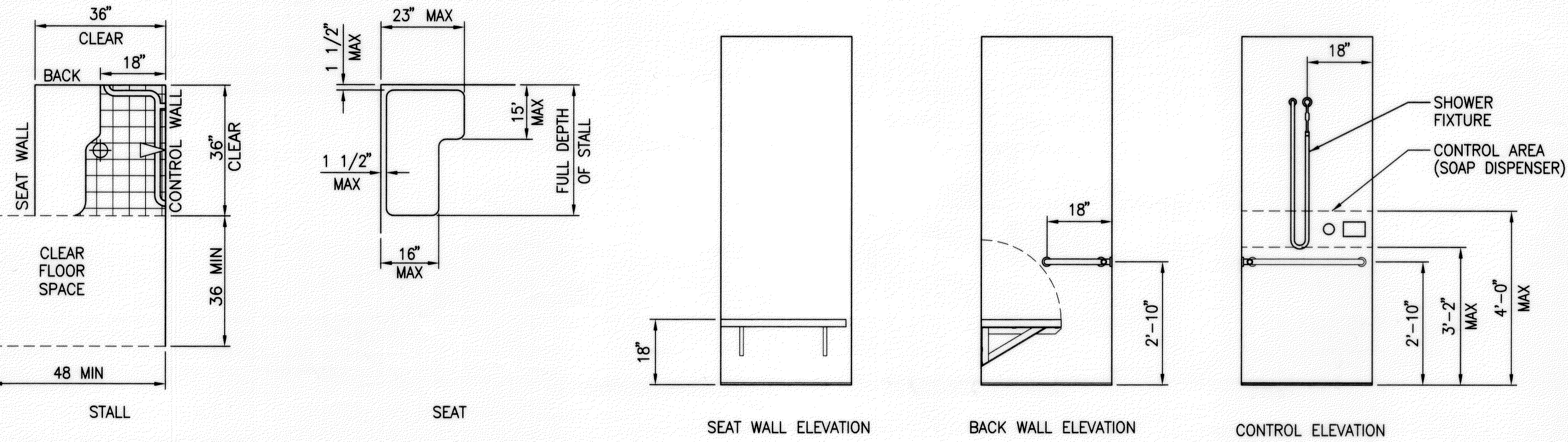
ADA SHOWER STALL SCALE: 1/2"=1'-0"
