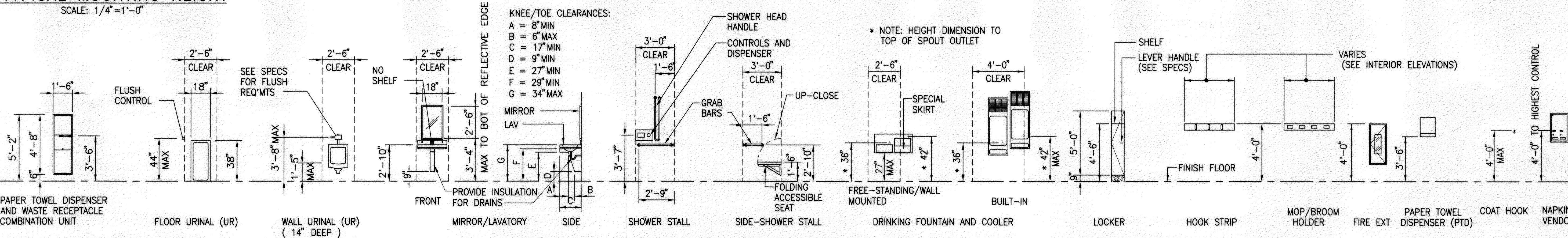
ADA FIXTURES AND EQUIPMENT MOUNTING HEIGHT SCALE: 1/4"=1'-0"
