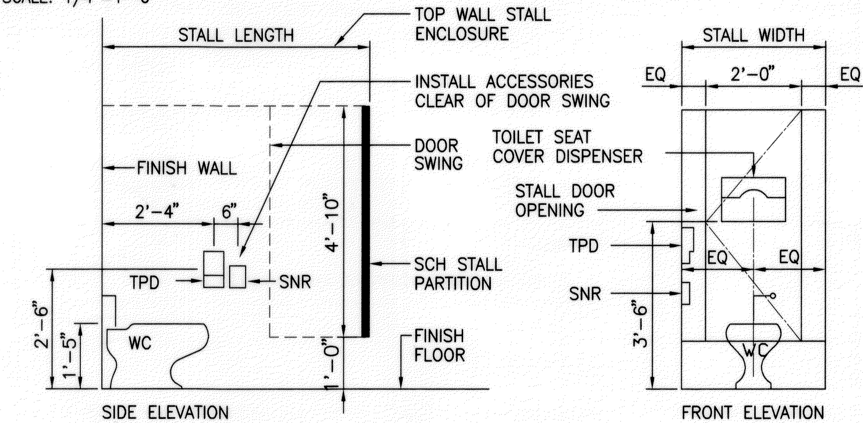
TYPICAL WATER CLOSET SCALE: 1/2"=1'-0"
