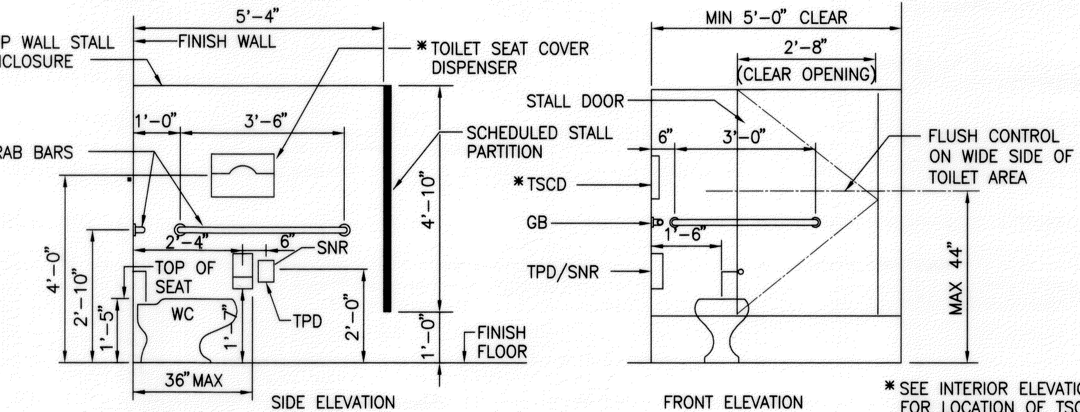
ADA WATER CLOSET SCALE: 1/2"=1'-0"
