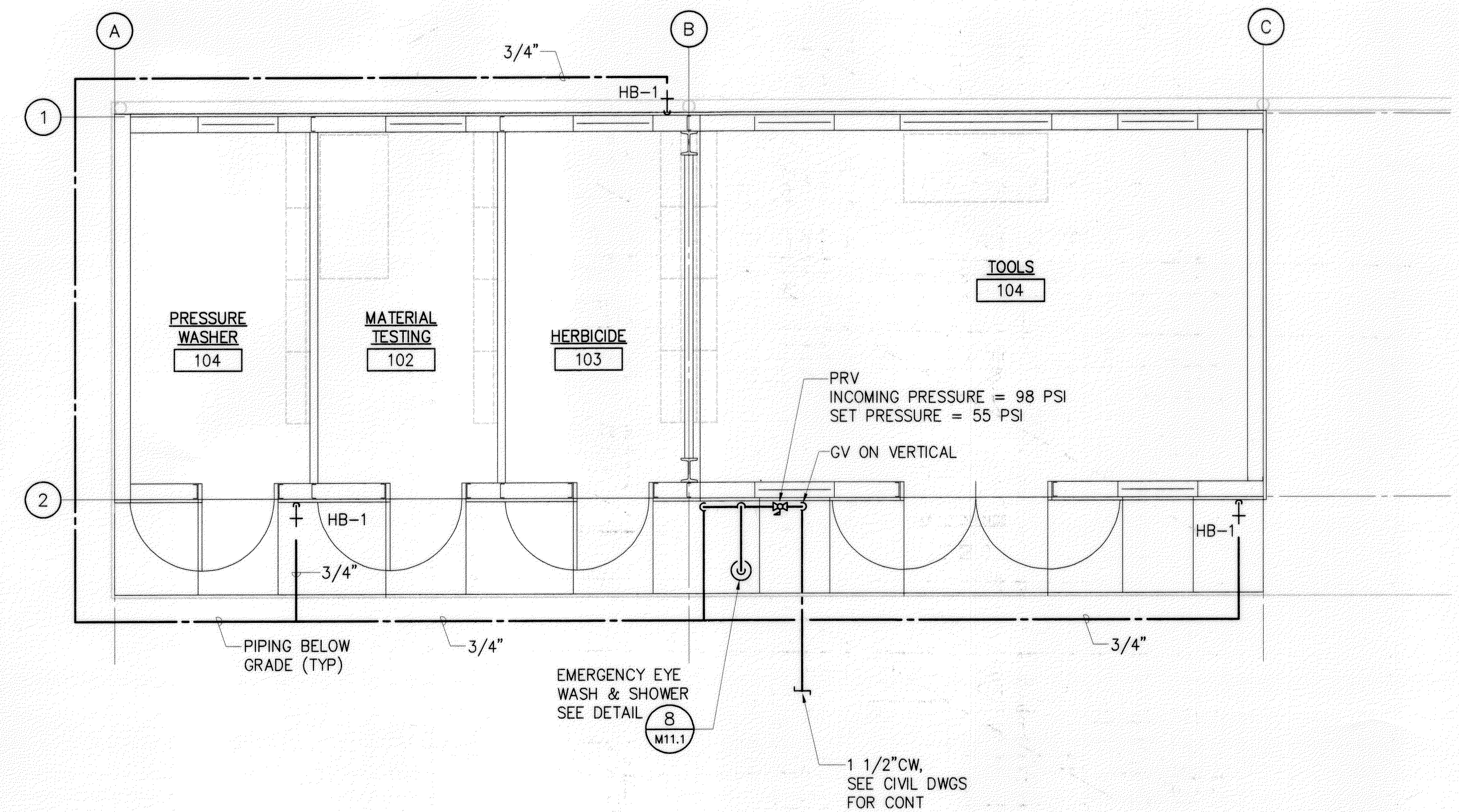
STORAGE BUILDING PLUMBING FLOOR PLAN (DEDUCTIVE NO. 1) SCALE: 1/4" = 1'-0"
