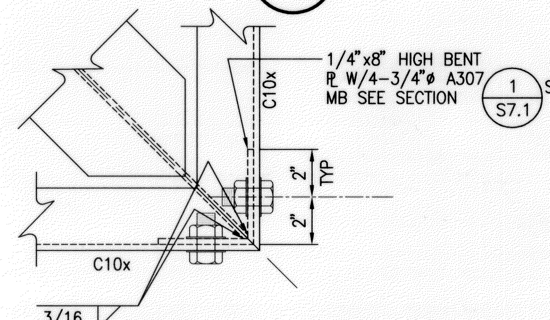
6A DETAIL S7.1 SCALE: 1"=1'-0"
