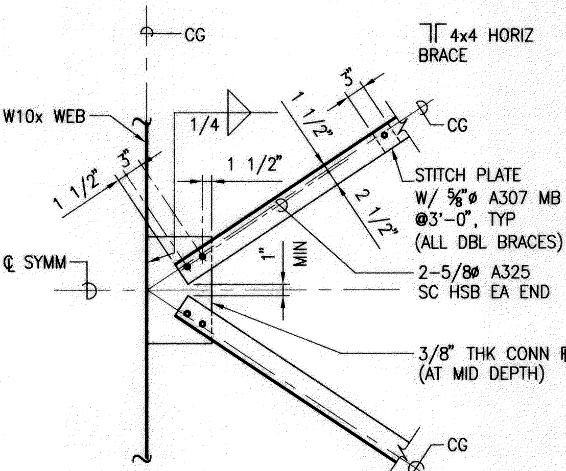
8 DETAIL - PLAN S7.1 SCALE: 3/4"=1'-0"
