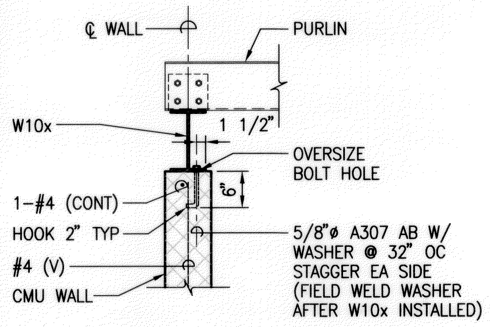
7 SECTION S7.1 SCALE: 3/4"=1'-0"
