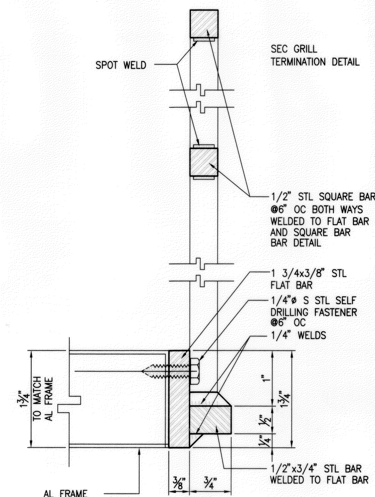
GRILL FRAME DETAILS
