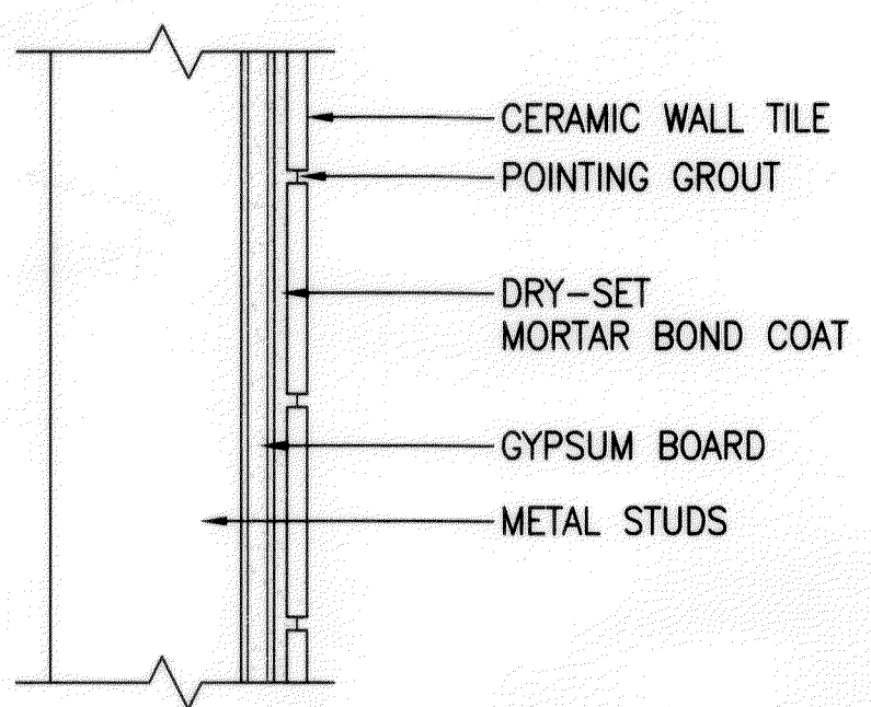
TCA DESIGN W243
