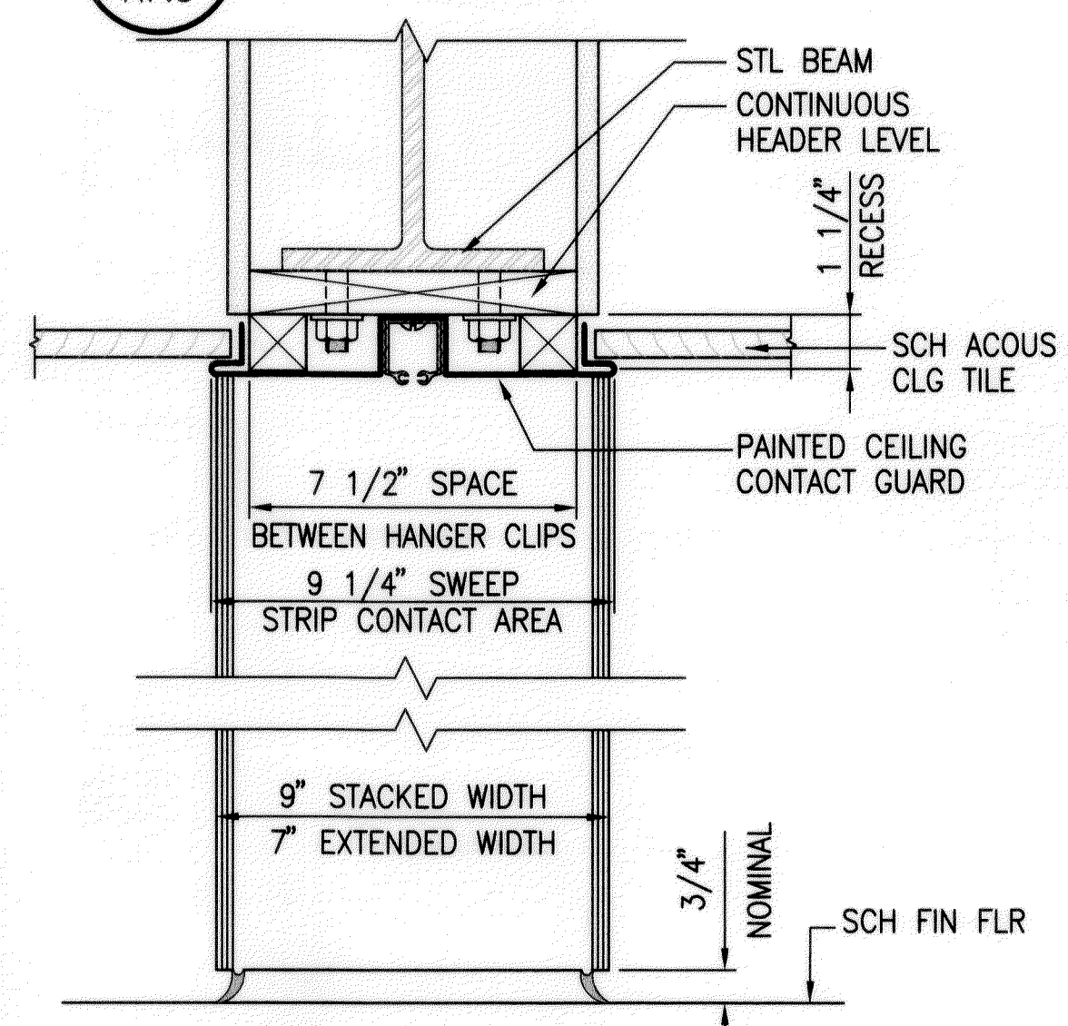
TYPICAL PANEL SECTION
