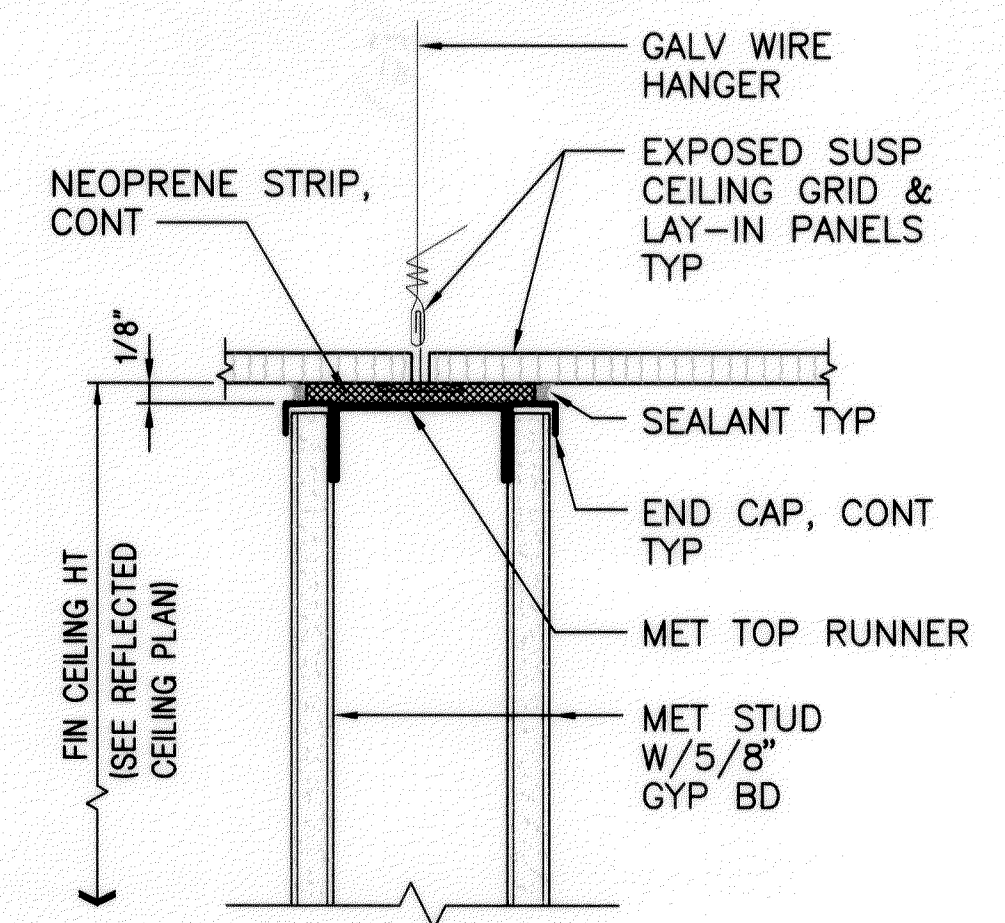
8 GYPSUM BOARD WALL @ TOP A7.3 SCALE: 1 1/2"=1'-0"
