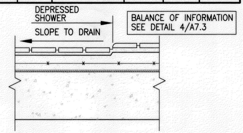
TCA DESIGN F121 MODIFIED FOR SHOWER CONFORMING TO ADA
