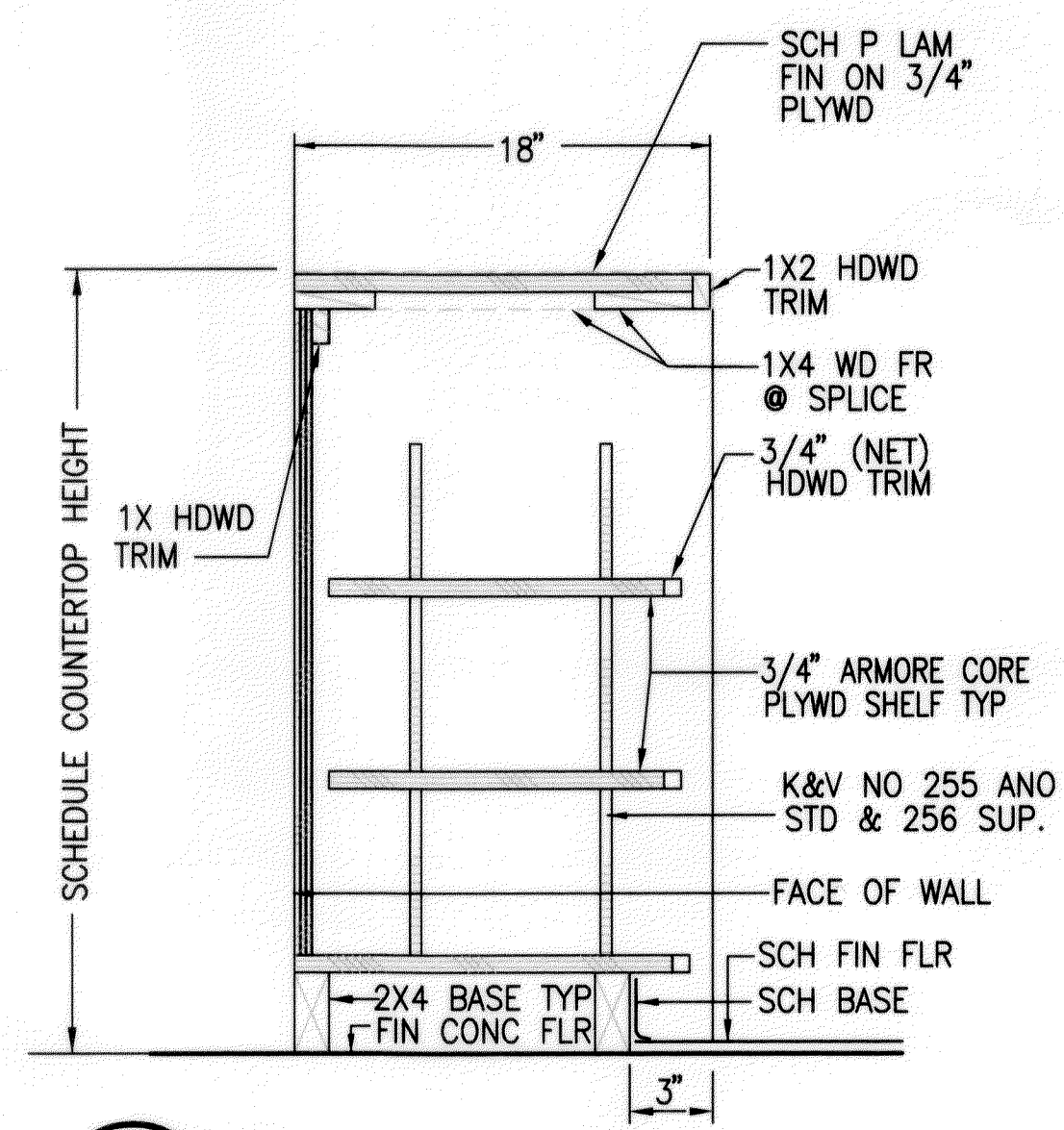
1 BASE COUNTER A7.4 SCALE: 1 1/2"=1'-0"
