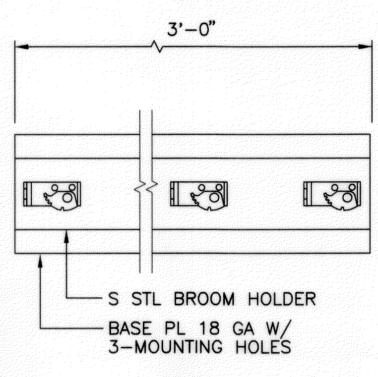
11 MOP/BROOM HOLDER A7.4 SCALE: 1 1/2"=1'-0"
