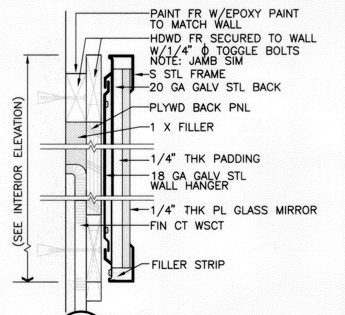
5 MIRROR DETAIL A7.4 SCALE: NTS
