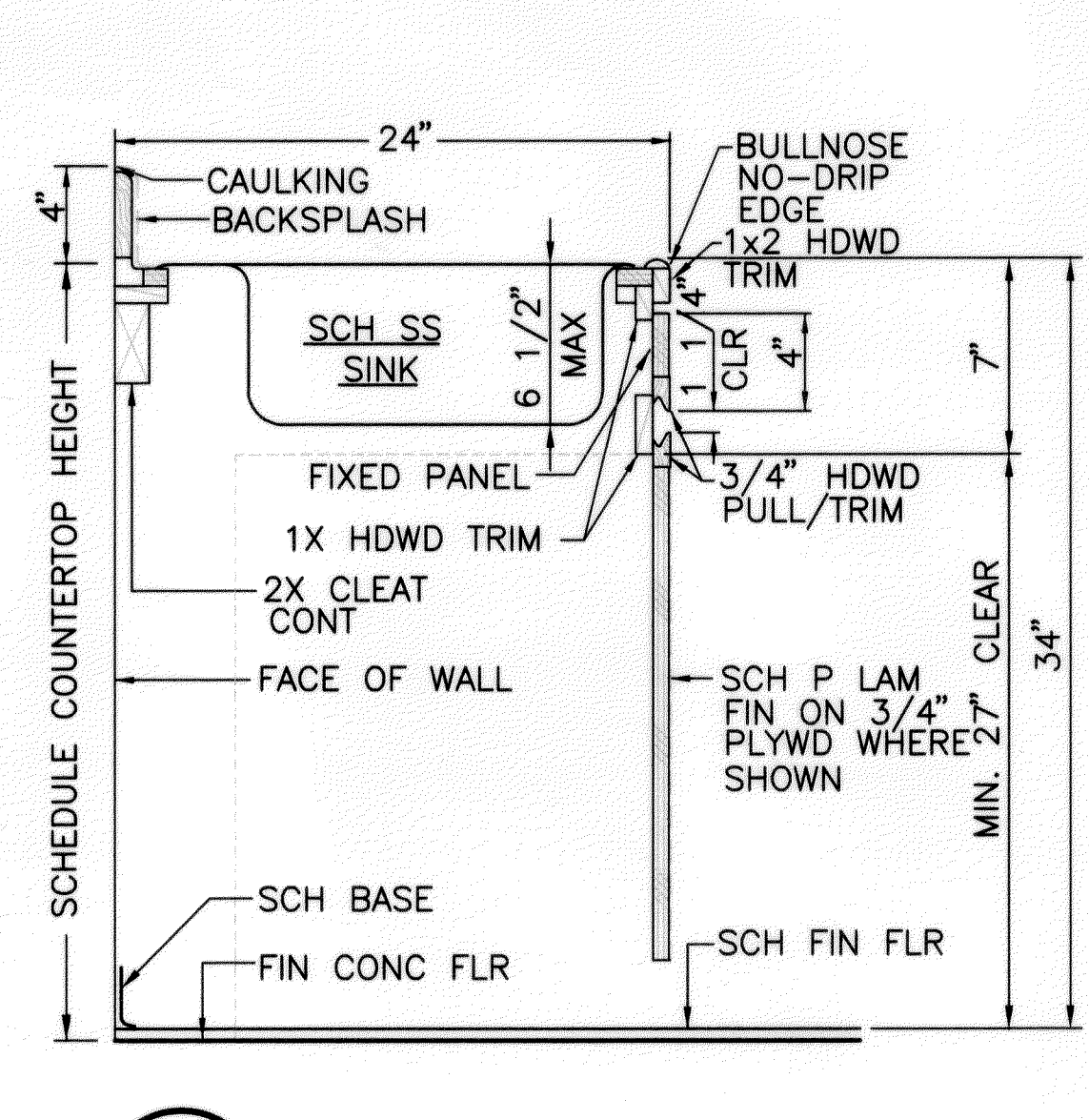
4 ADA COUNTER W/ SINK A7.4 SCALE: 1 1/2"=1'-0"
