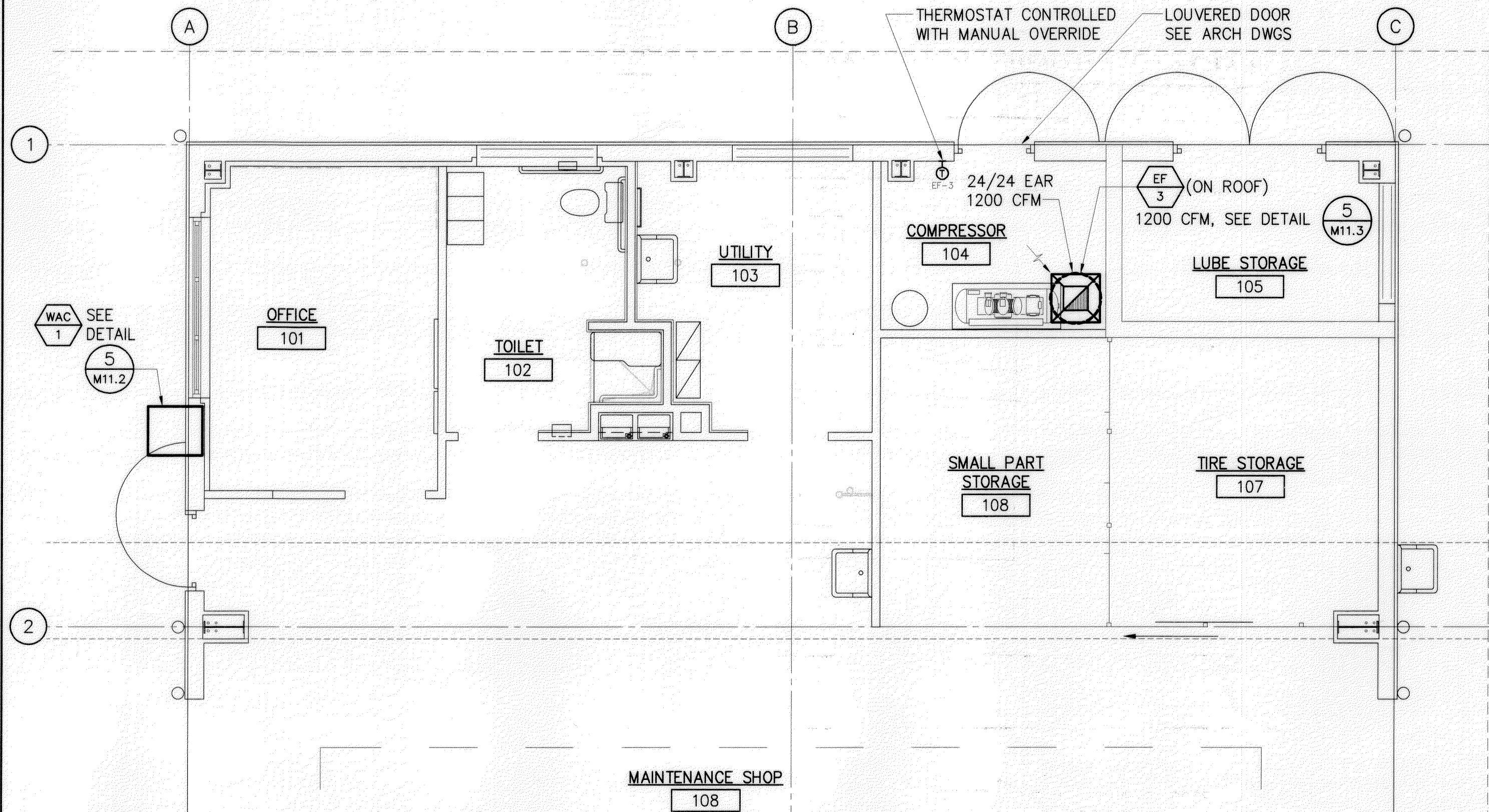
B DETAILED AIR CONDITIONING & VENTILATION FLOOR PLAN SCALE: 1/4" = 1'-0"
