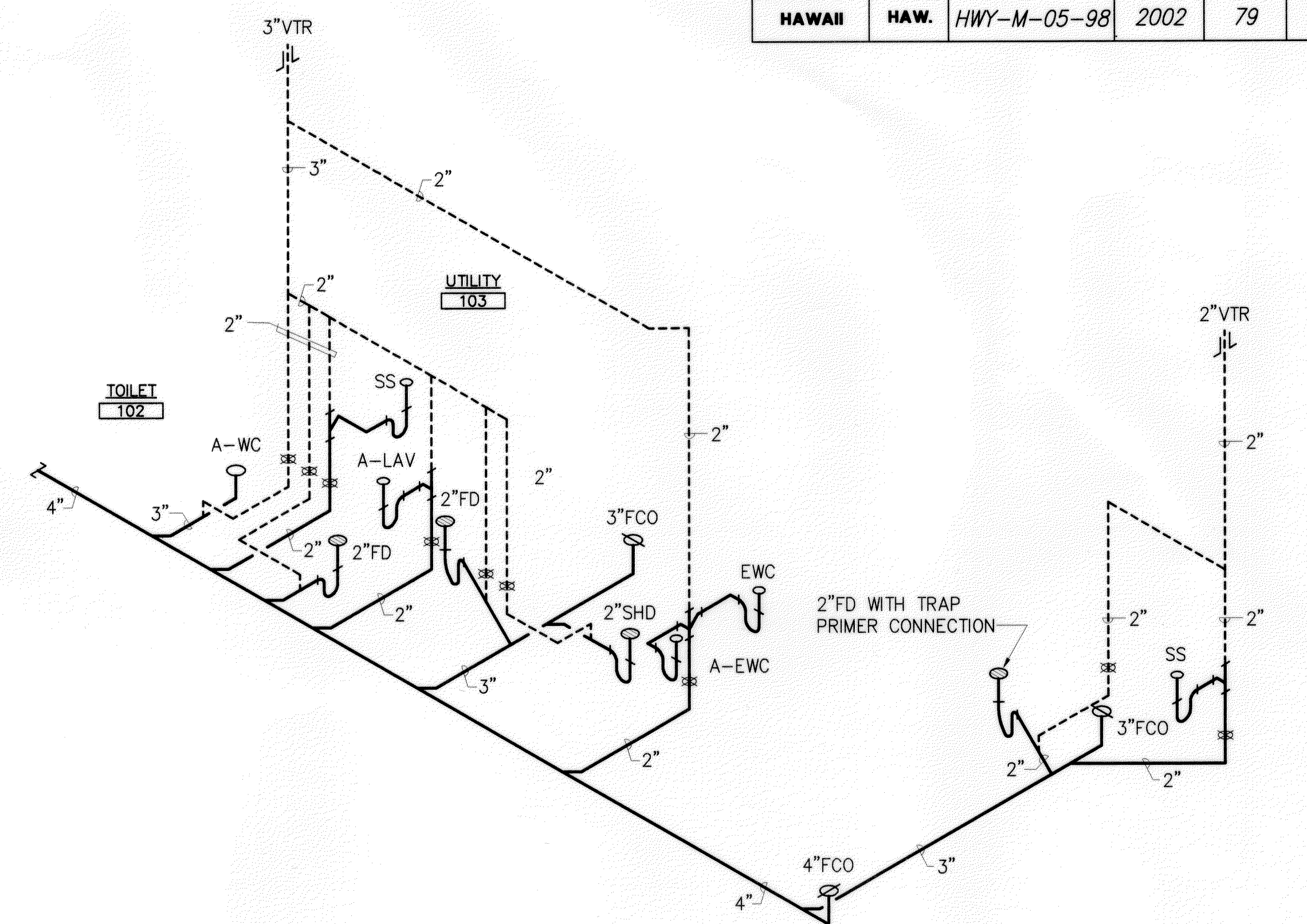
MAINTENANCE BUILDING – SANITARY PIPING DIAGRAM SCALE: NONE
