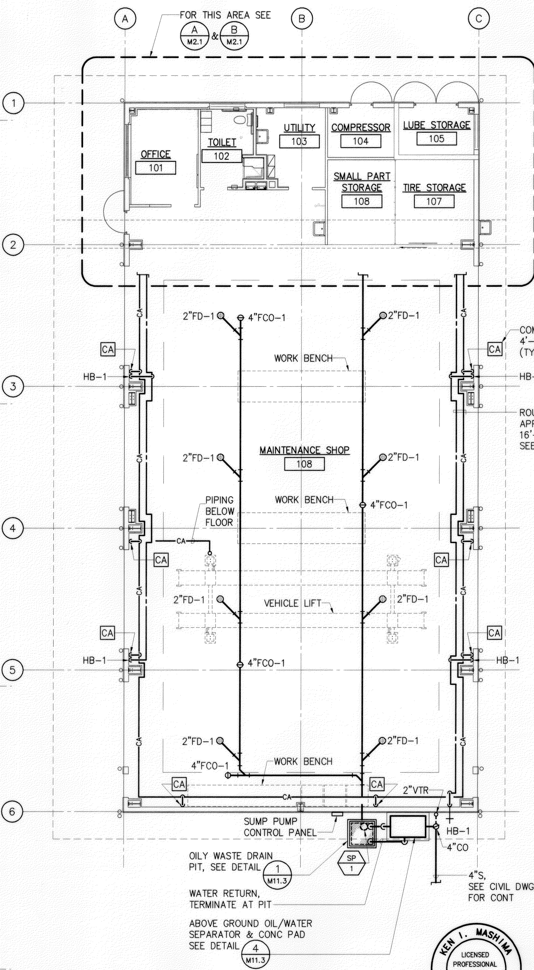
MAINTENANCE BUILDING PLUMBING FLOOR PLAN SCALE: 1/8" = 1'-0"
