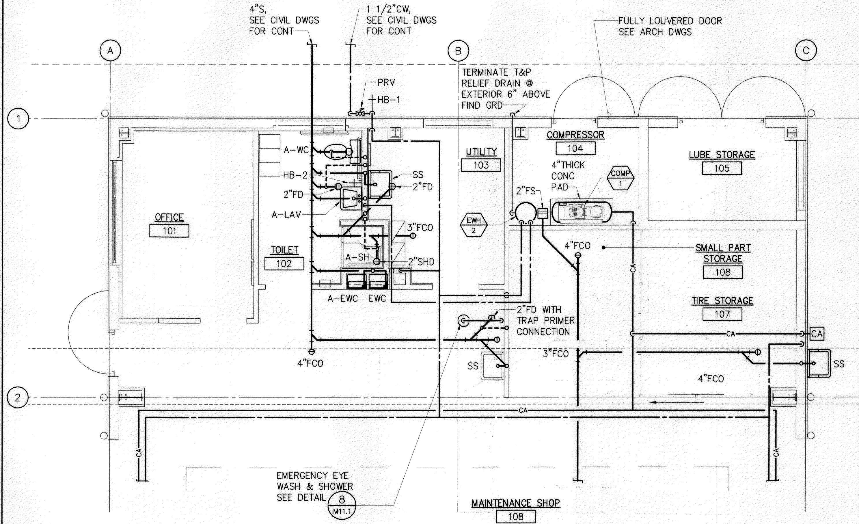
A DETAILED PLUMBING FLOOR PLAN SCALE: 1/4" = 1'-0"
