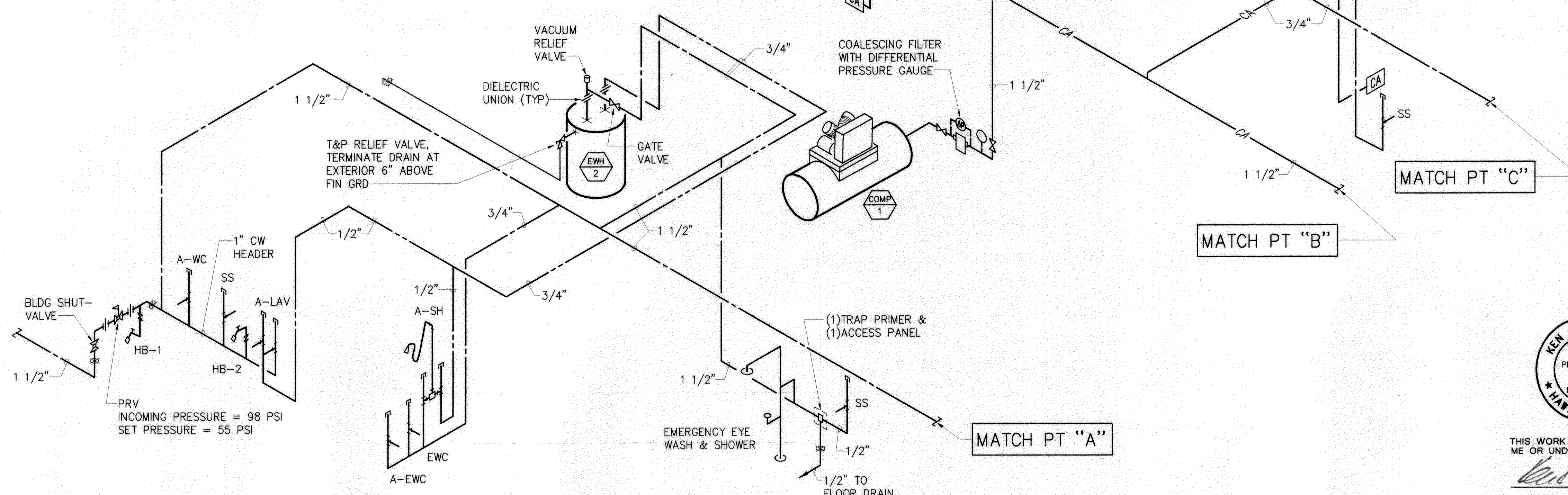
MAINTENANCE BUILDING – WATER & COMPRESSED AIR PIPING DIAGRAM SCALE: NONE
