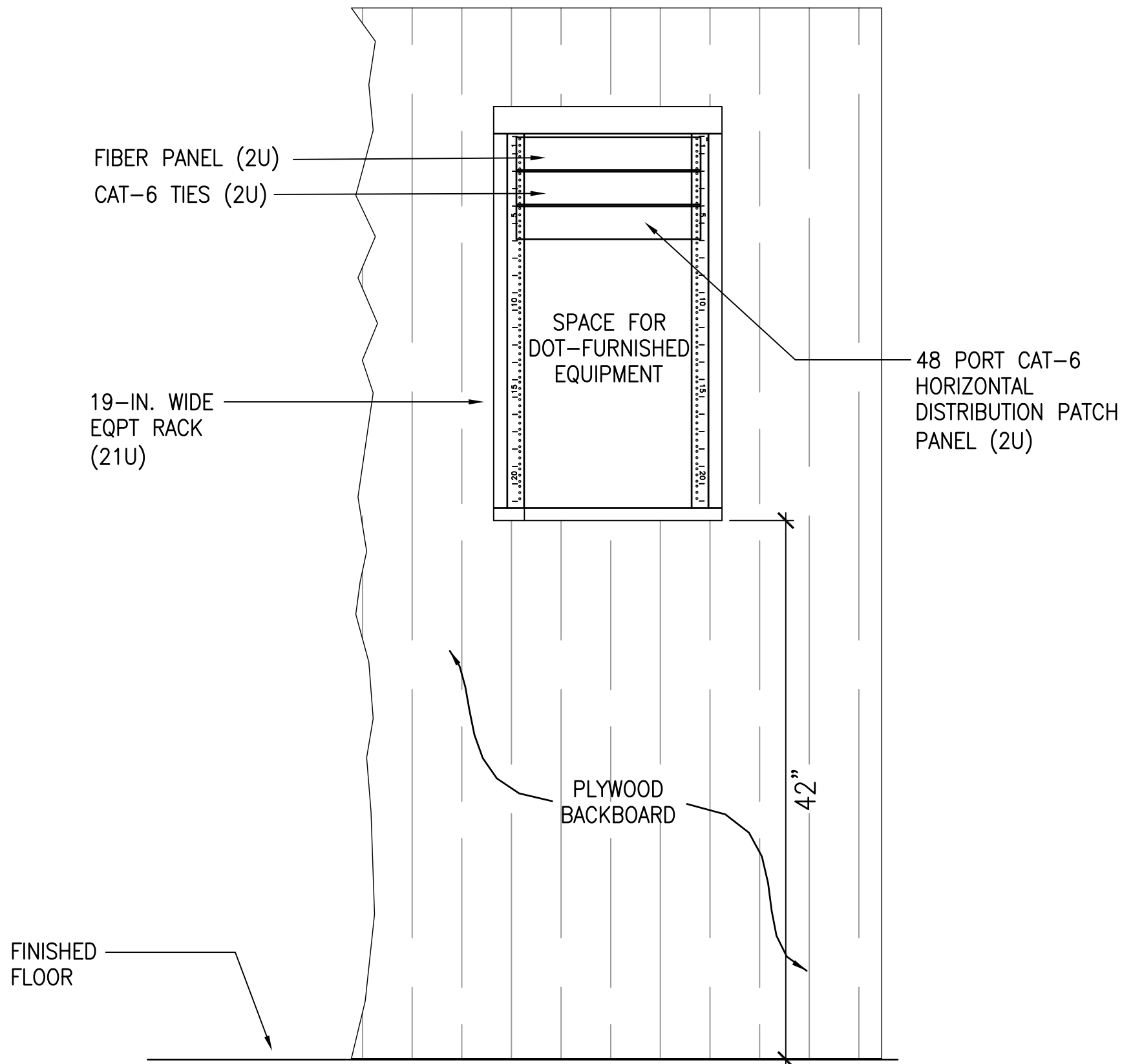
2 WALL MOUNTED TELECOM EQUIPMENT RACK ELEVATION - NEW BUILDING E14 NOT TO SCALE
