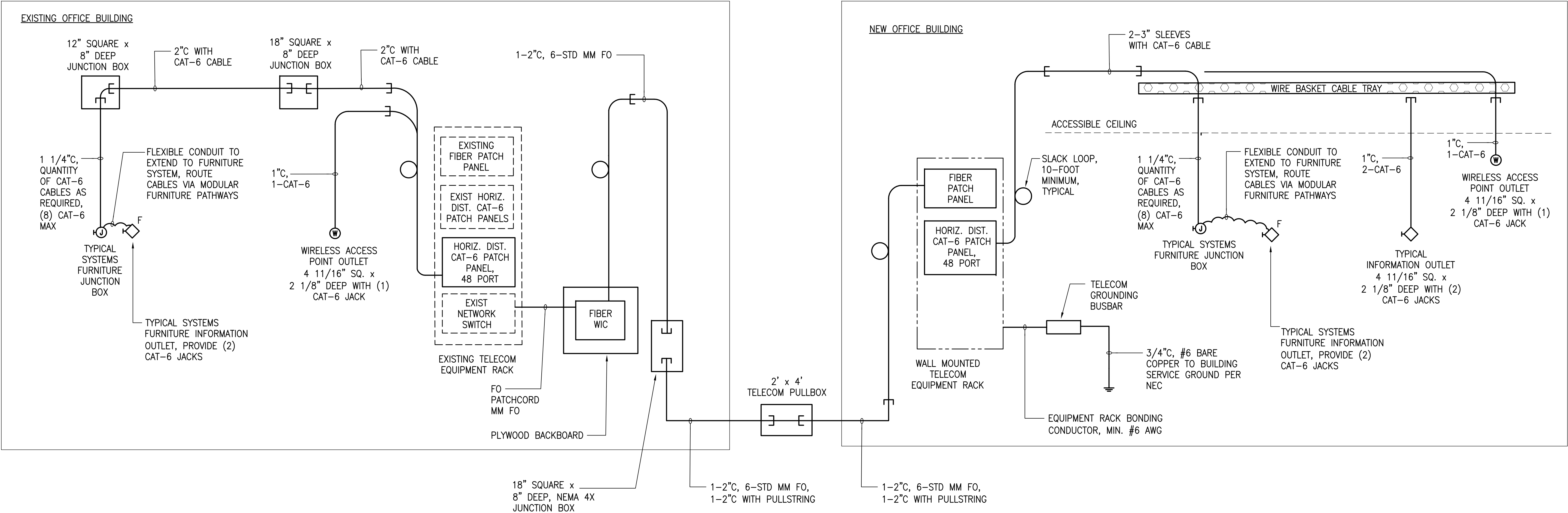
1 TELECOMMUNICATIONS RISER DIAGRAM E14 NO SCALE
