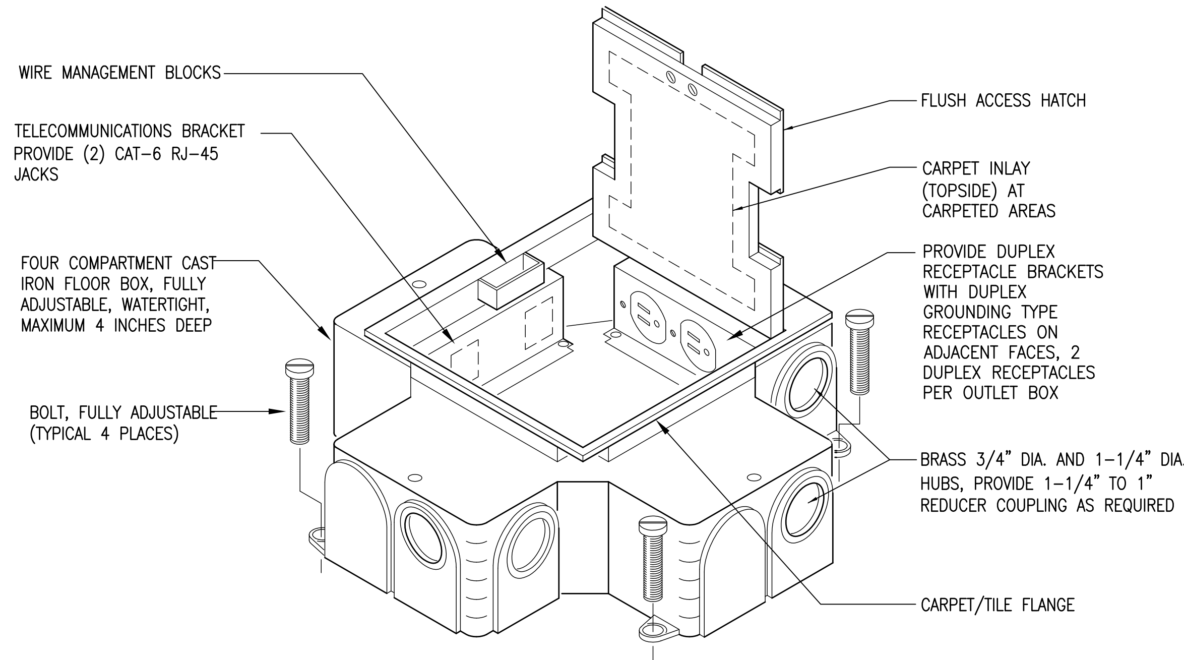
2 FLOOR OUTLET E20 NO SCALE
