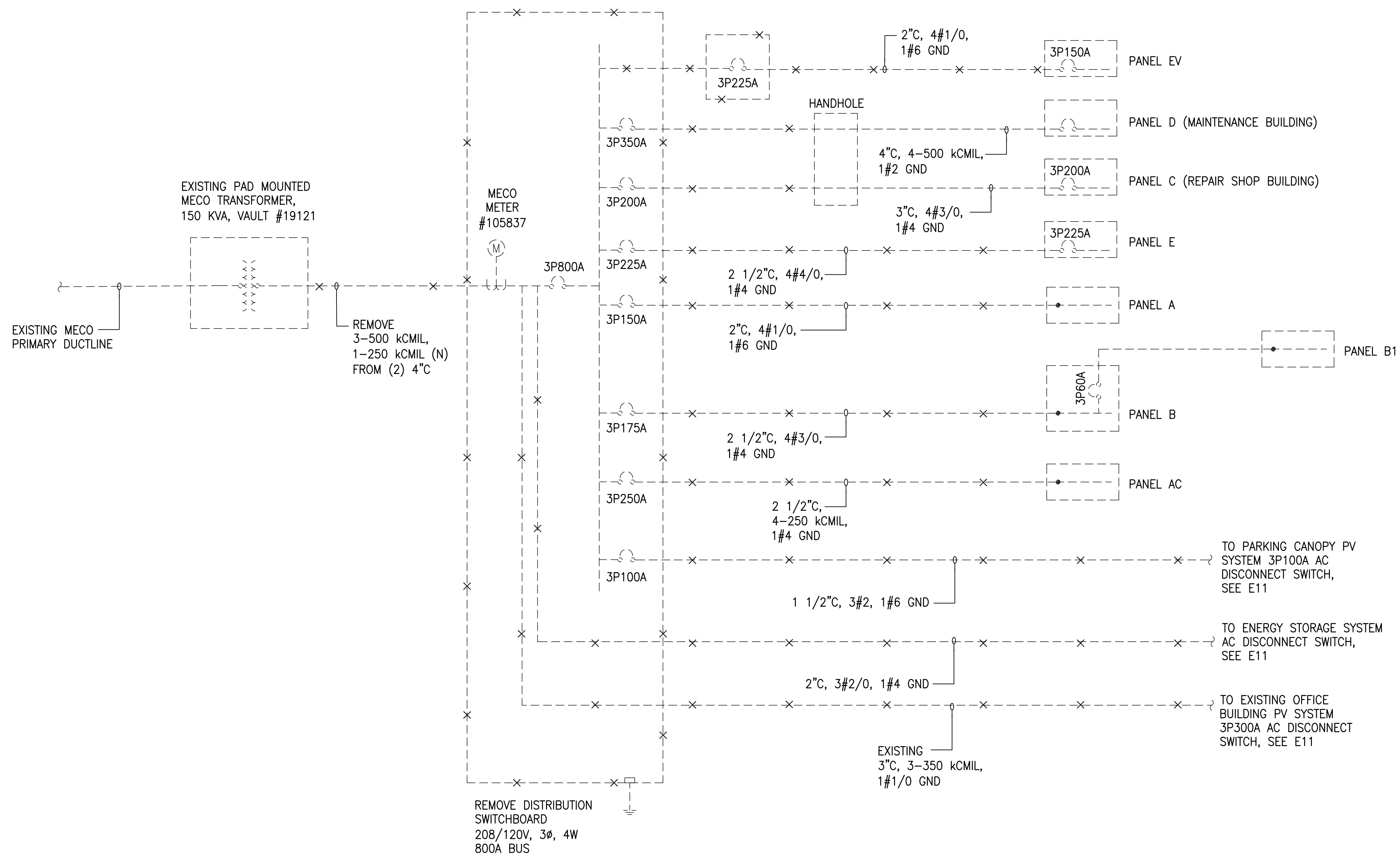
DEMOLITION/EXISTING ONE LINE DIAGRAM - 1 NO SCALE
