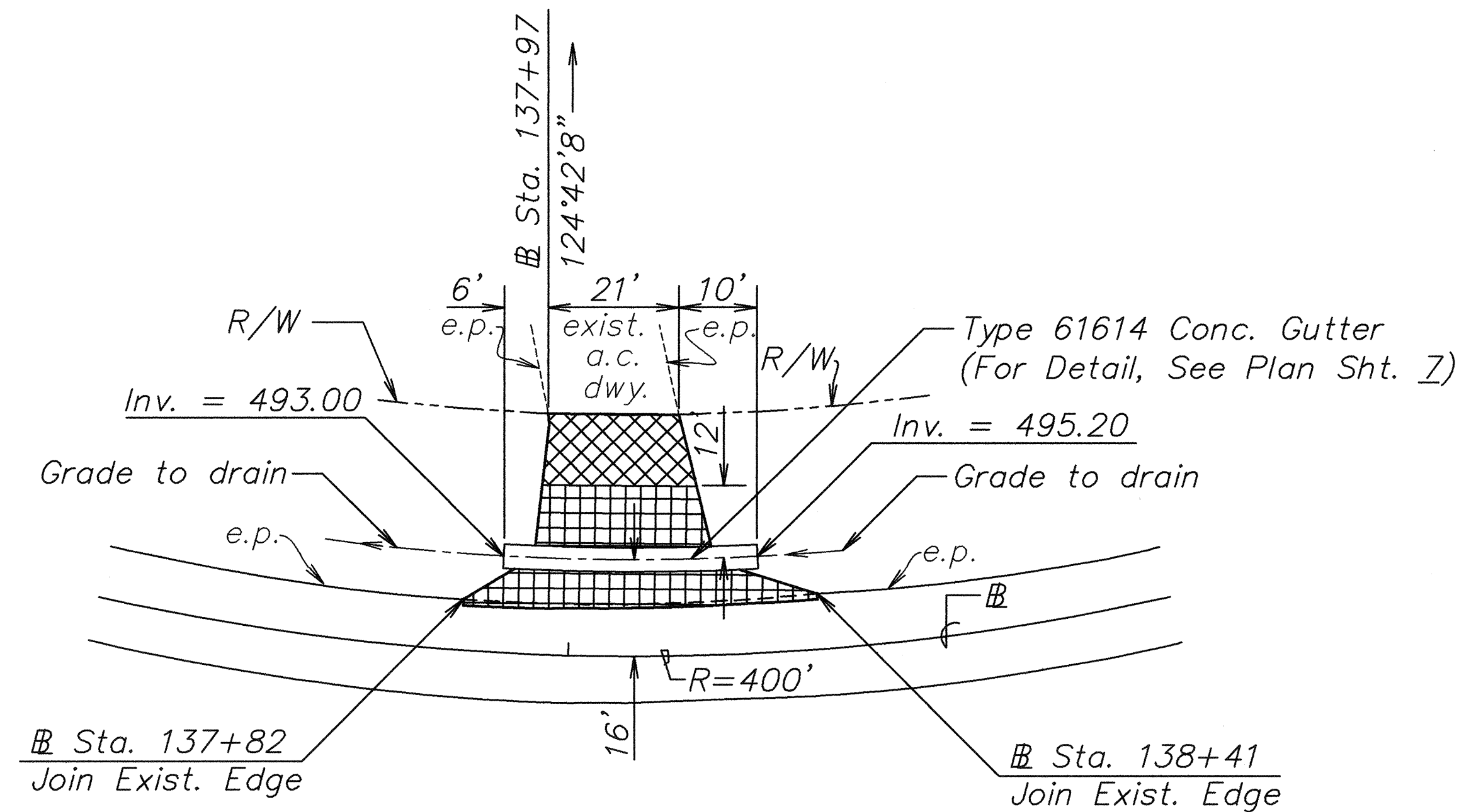
DETAIL PLAN – EXISTING DRIVEWAY STA. 137+82 TO STA. 138+41 Scale: 1"=20'
