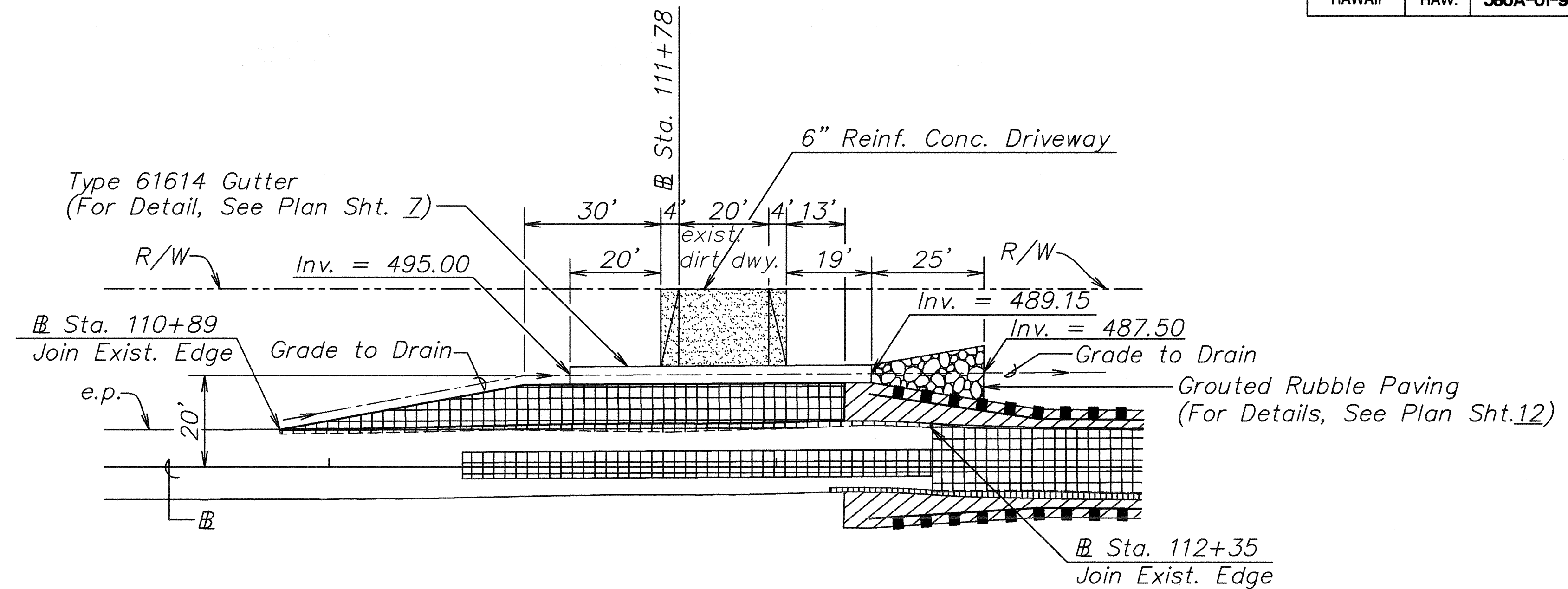
DETAIL PLAN – EXISTING DRIVEWAY STA. 110+89 TO STA. 112+35 Scale: 1"=20'
