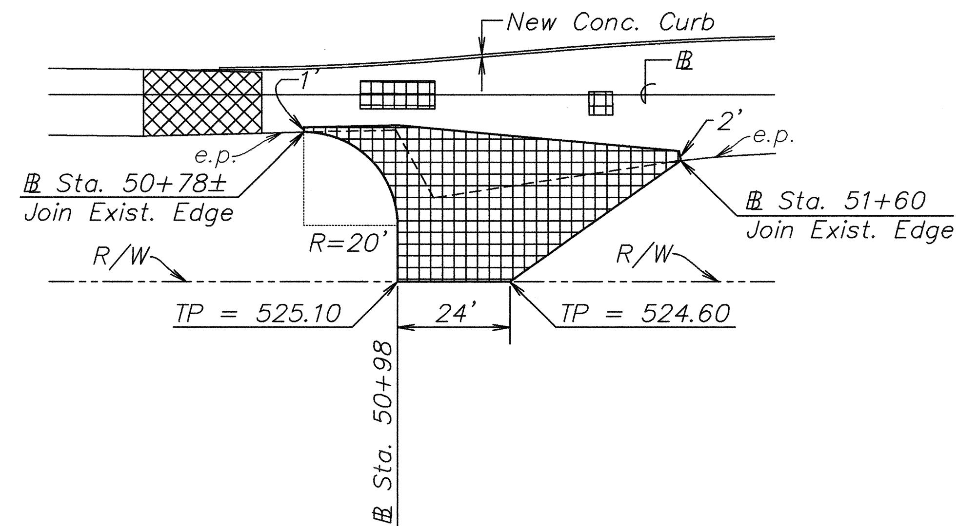
DETAIL PLAN – EXISTING DRIVEWAY STA. 50+78 TO STA. 51+60 Scale: 1"=20'
