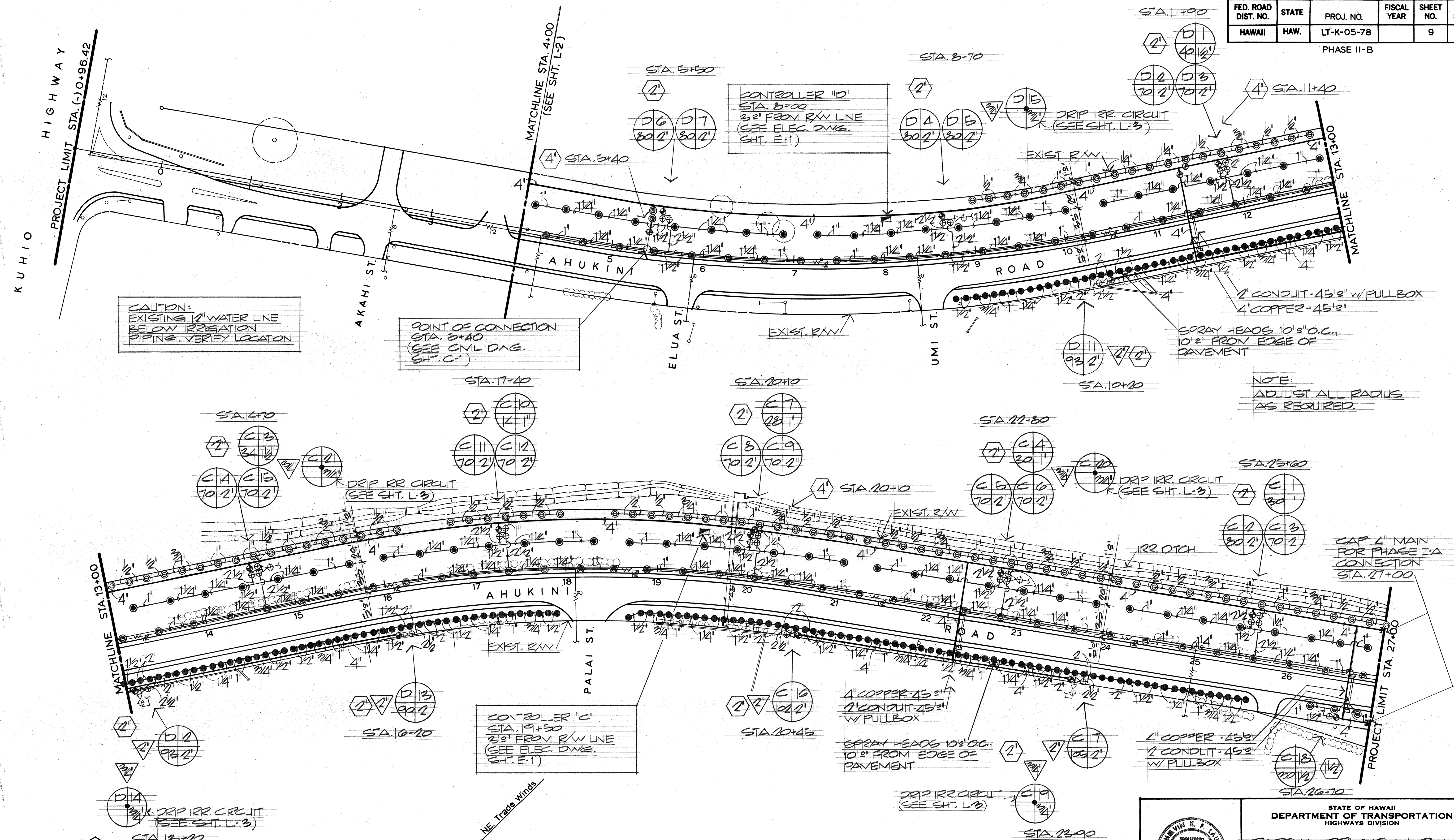
PARTIAL IRRIGATION PLAN SCALE = 1" = 50'
