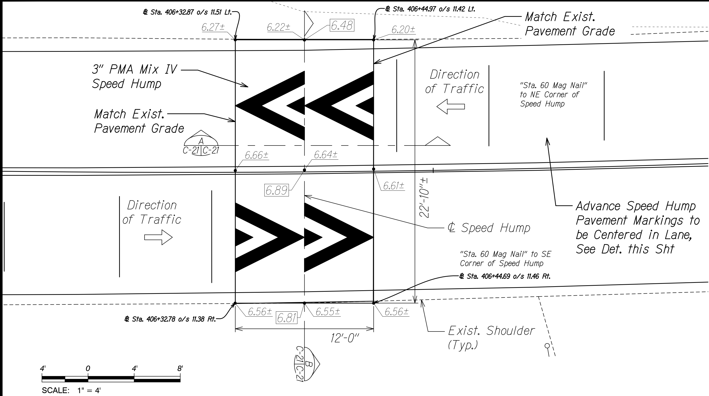
ENLARGED PLAN @ STA. 406+38.83 Scale: 1"=4'
