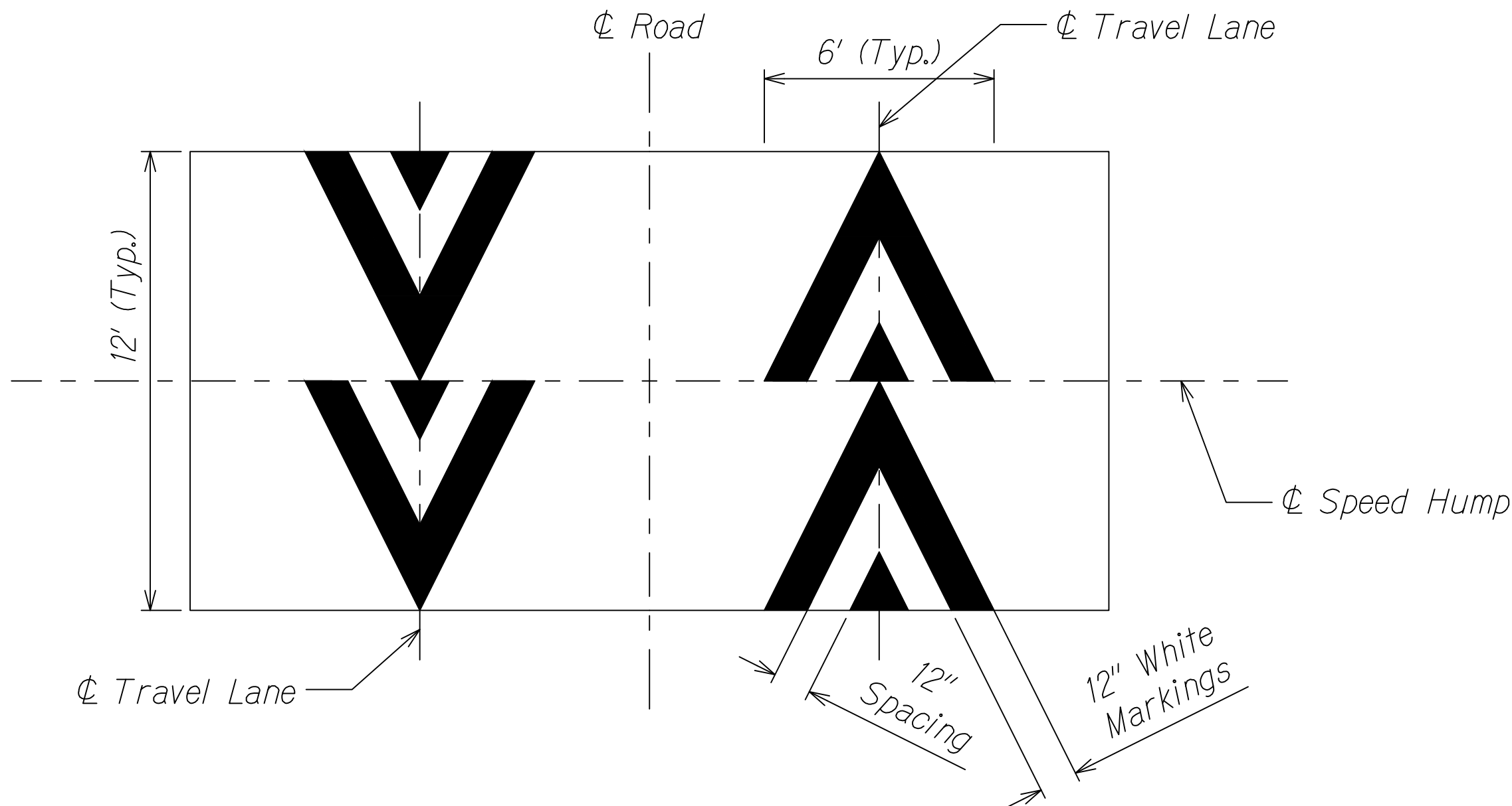
Typical Speed Hump Pavement Marking Detail
