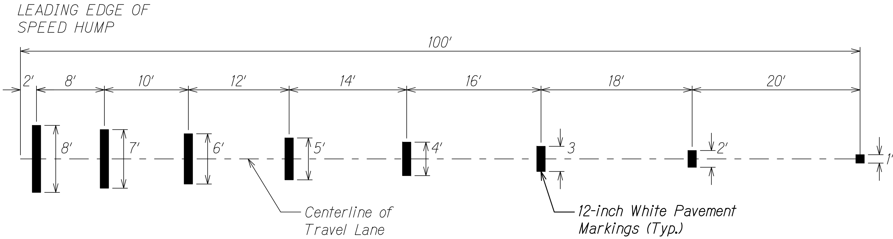
Typical Advance Speed Hump Pavement Marking Detail
