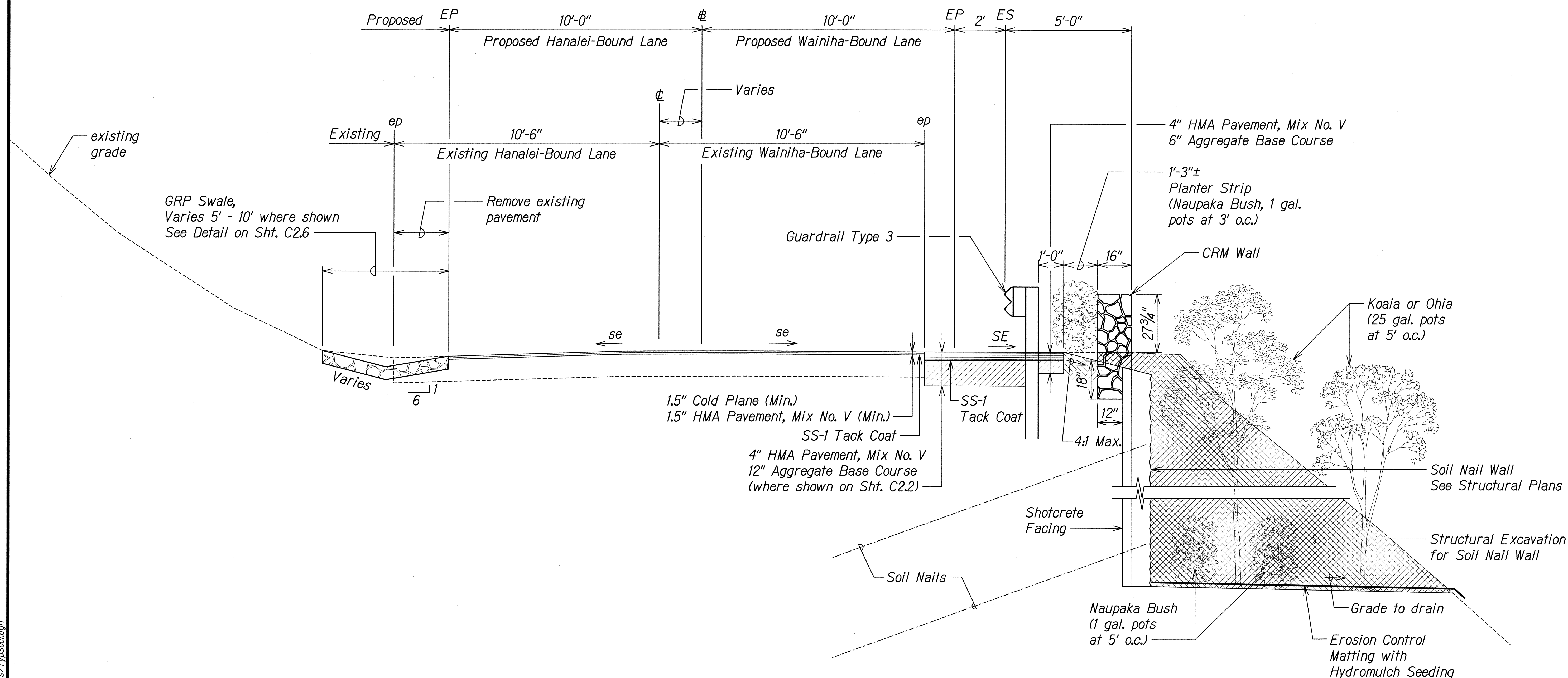
TYPICAL SECTION - SOIL NAIL WALL (LOOKING DOWNSTATION) Scale: 1/2" = 1'-0"
