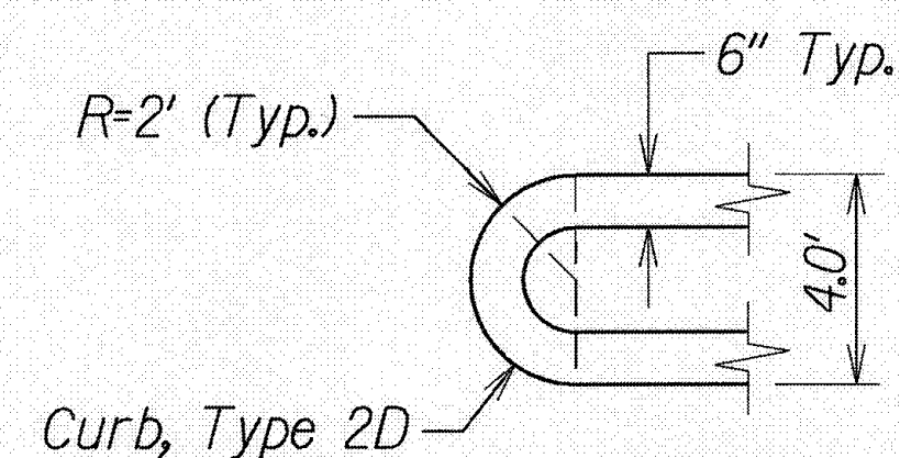
TYPICAL NOSING DETAIL Not to Scale
