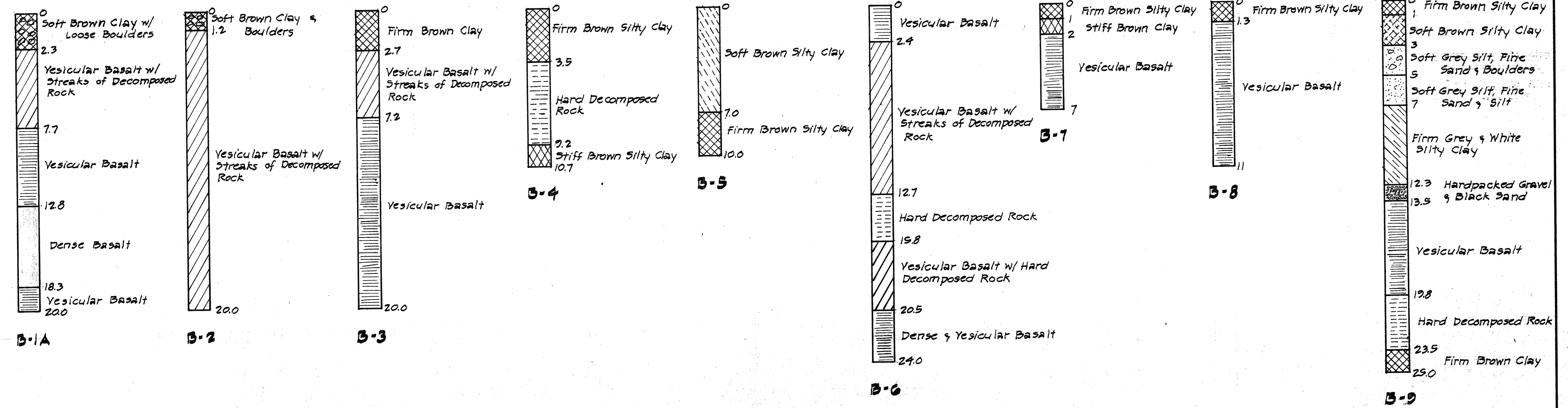
BORING LOGS Not to Scale
