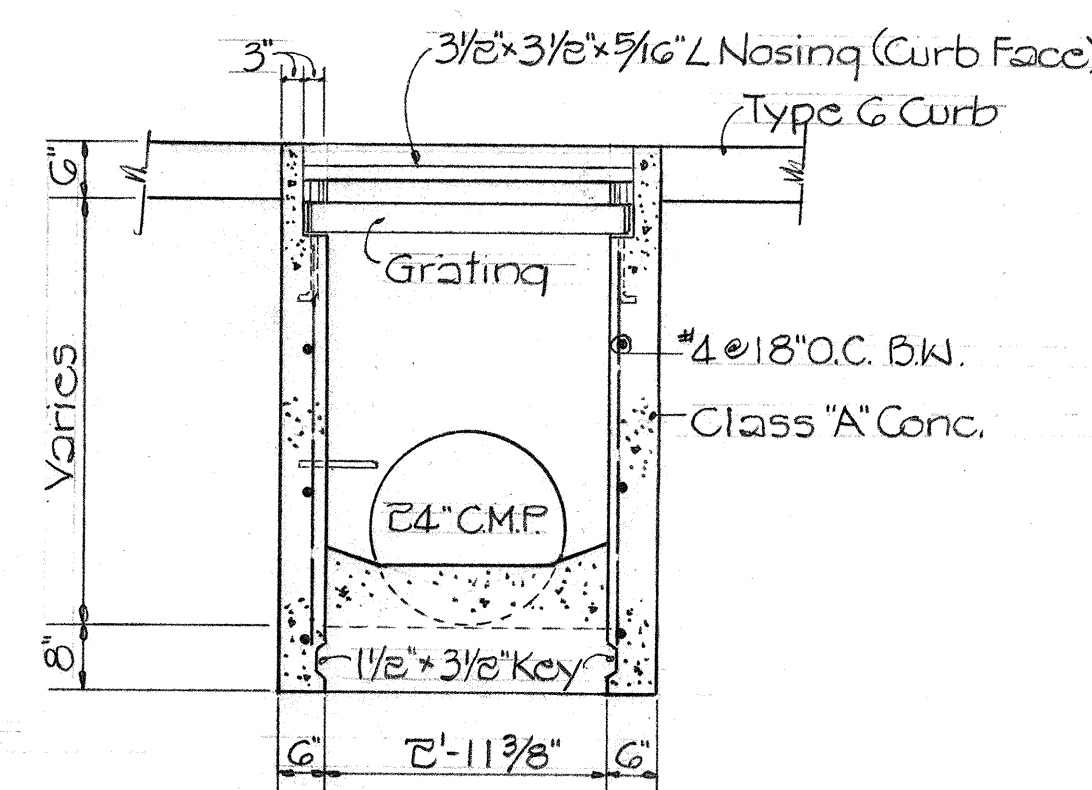
SECTION "B"-B"
