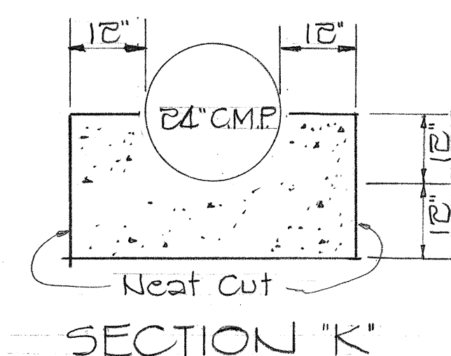
SECTION "K"
