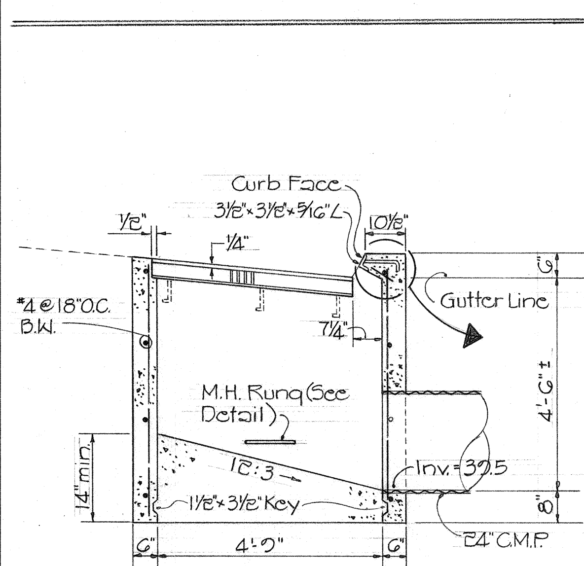
SECTION "A"-A"
