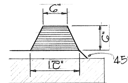
TYPE G CURBING (A.C.)
