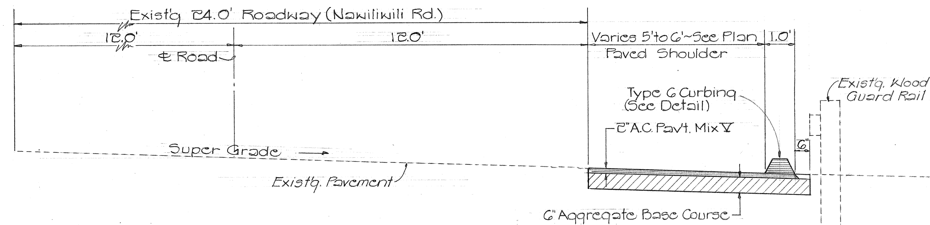
TYPICAL ROAD SECTION SHOWING NEW PAVED SHOULDER Scale: 1/8"=1'-0"
