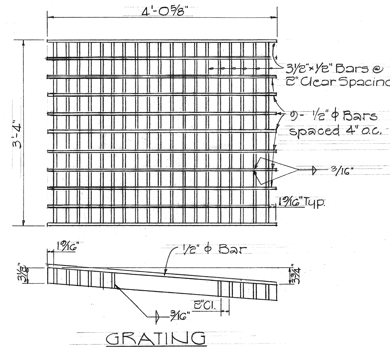
DETAIL ~ TYPE "K" STEEL FRAME & GRATE Scale: 1"=1'-0"
