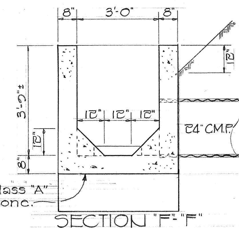
DETAIL ~ CONIC. OUTLET BOX Scale: 1/2"=1'-0"
