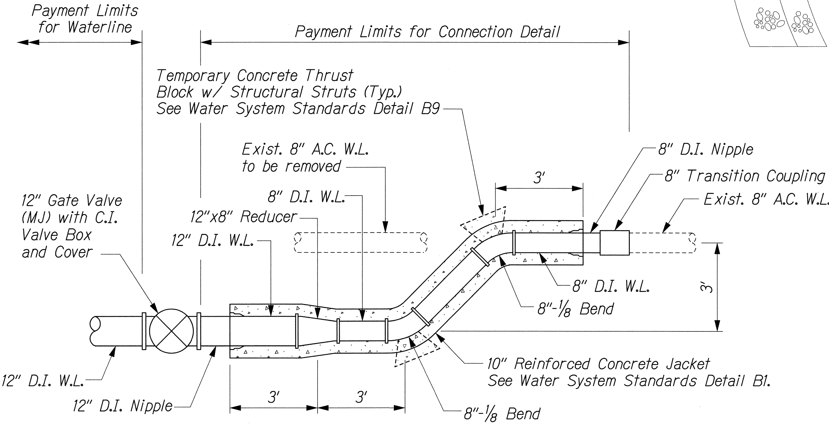
CONNECTION DETAIL - PLAN VIEW Scale: 1/2"=1'-0"
