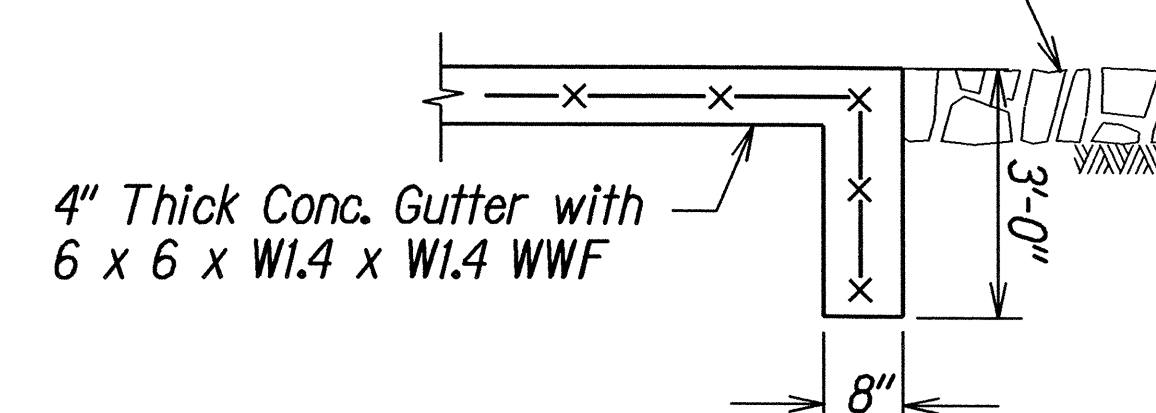
CUT-OFF WALL DETAIL Not to Scale
