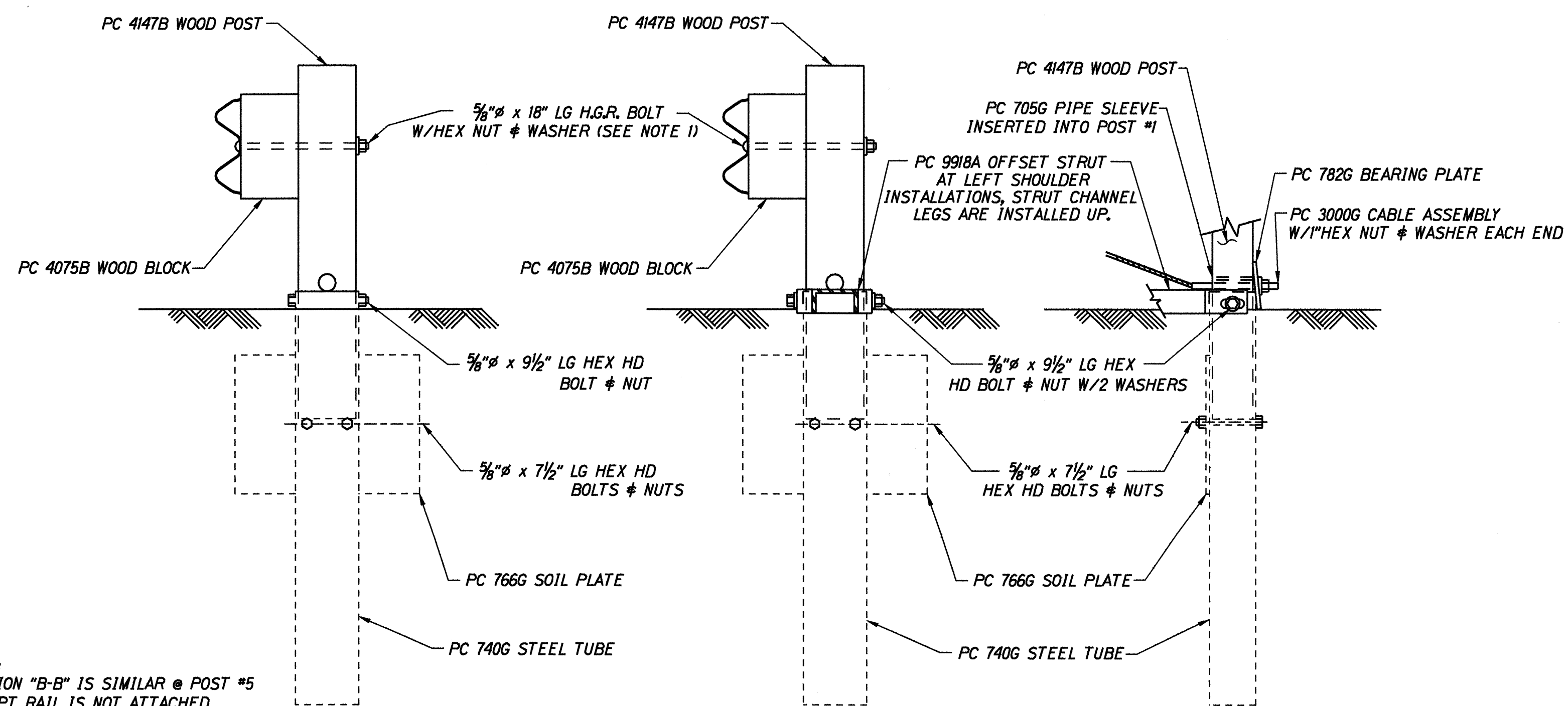
SECTION "B-B" (TYP @ POSTS #3, 4, 6, 7 & 8)
