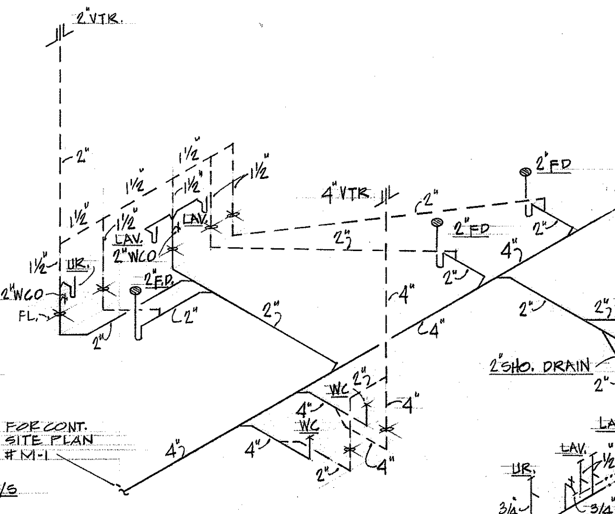
ALTERNATE #4 SANITARY DIAGRAM (BUILDING "C") NOT TO SCALE
