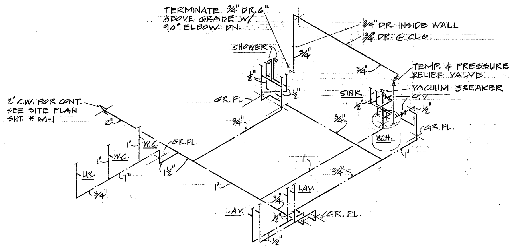
HOT & COLD WATER DIAGRAM (N.I.C.) (BUILDING "A") NOT TO SCALE
