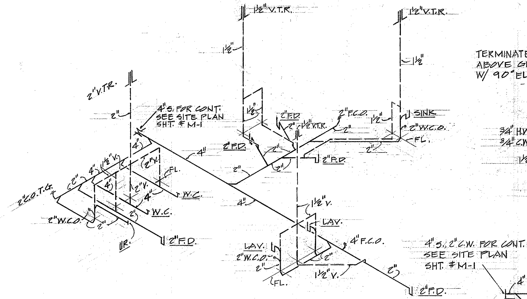
SANITARY DIAGRAM (N.I.C.) (BUILDING "A") NOT TO SCALE
