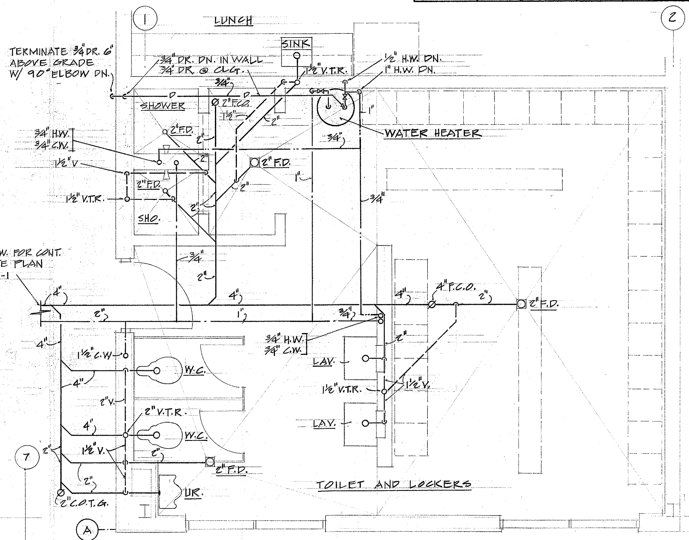
TOILET & LOCKER ROOM FLOOR PLAN (BUILDING "A") N.I.C. SCALE: 3/8"=1'-0" M-2
