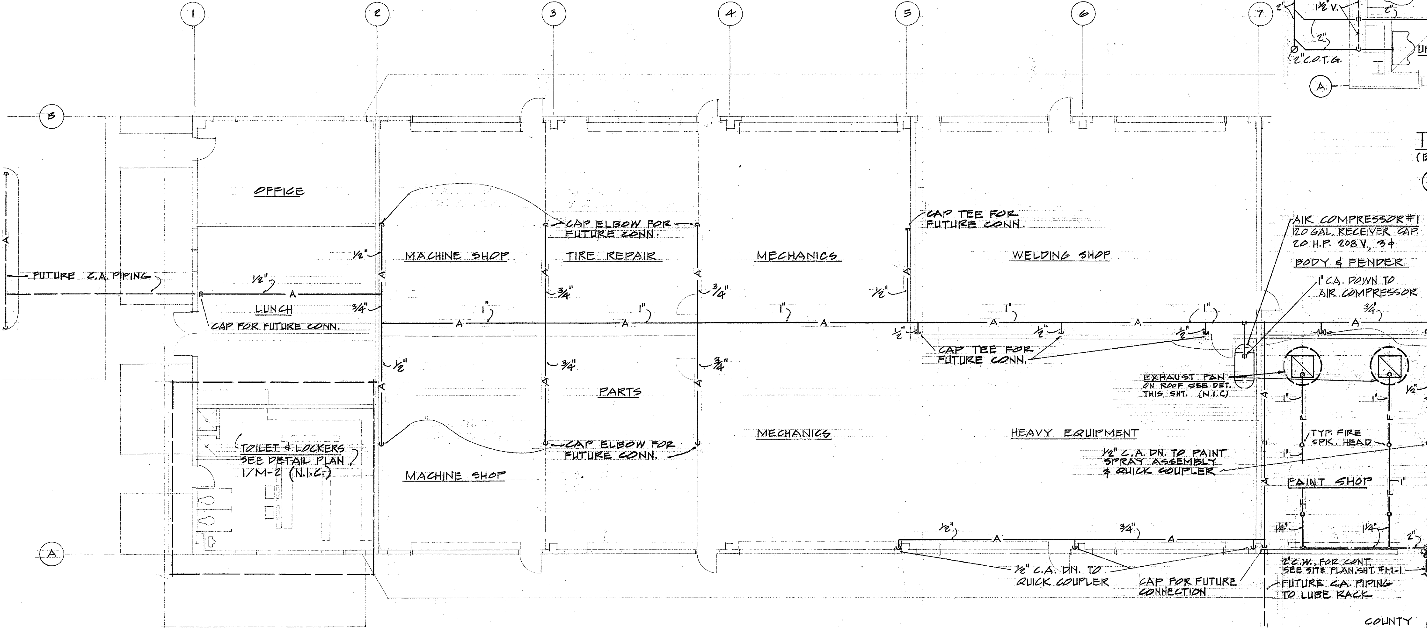
PARTIAL BLDG. "A" FLOOR PLAN (COUNTY) SCALE: 1/8"=1'-0"
