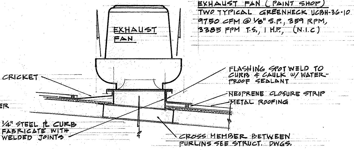
EXH. FAN SUPPORT DETAIL (N.I.C.) SCALE: 3/8"=1'-0"
