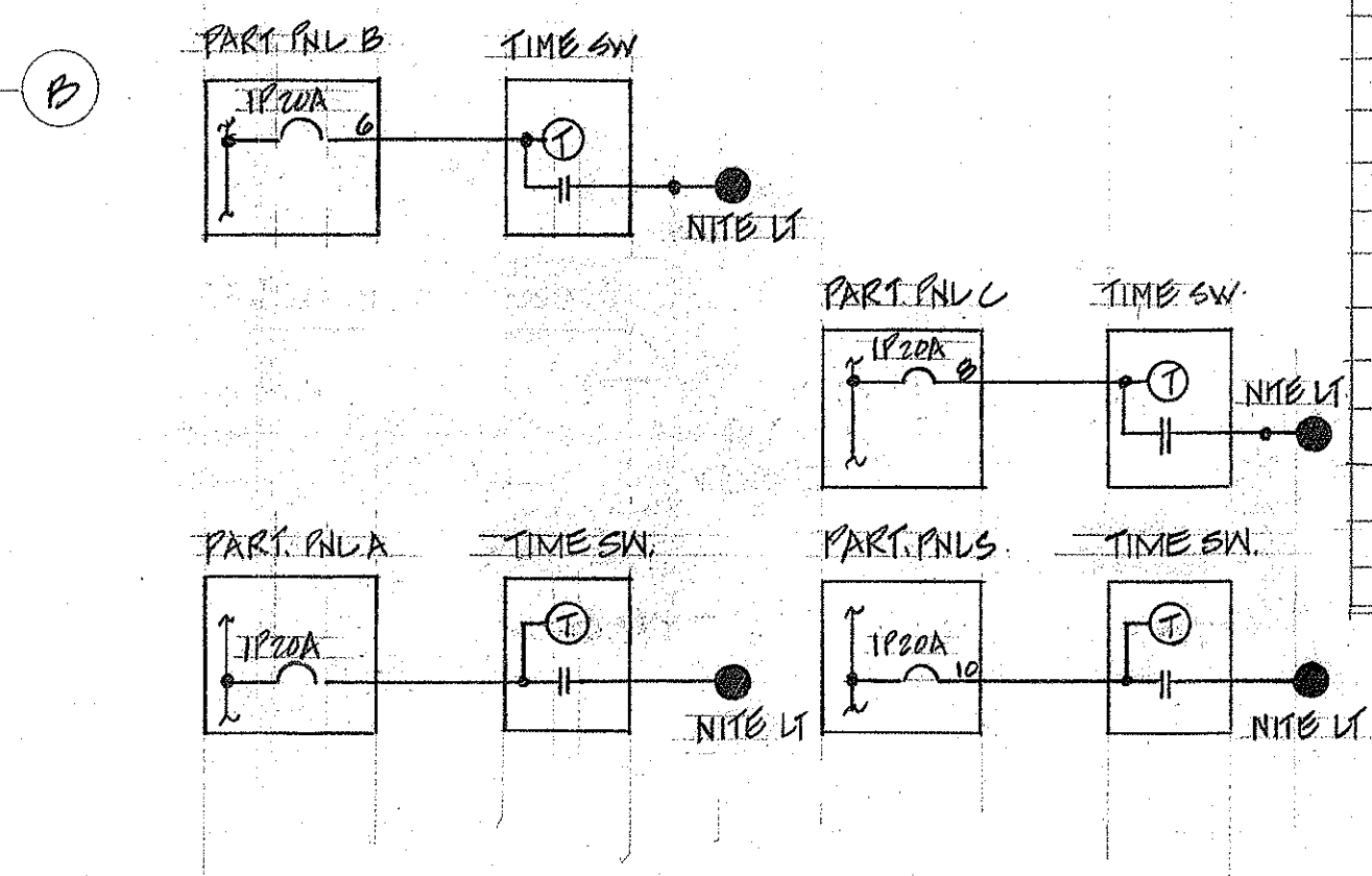
NITE NIGHT CONTROL DIAGRAM
