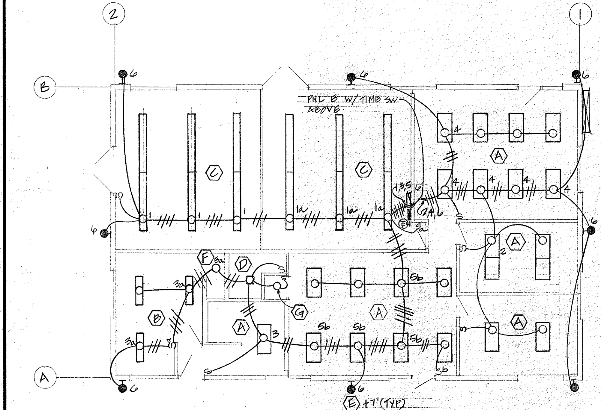
ALT. #1 - LIGHTING PLAN - BLDG. B (COUNTY) SCALE: 1/8"=1'-0"
