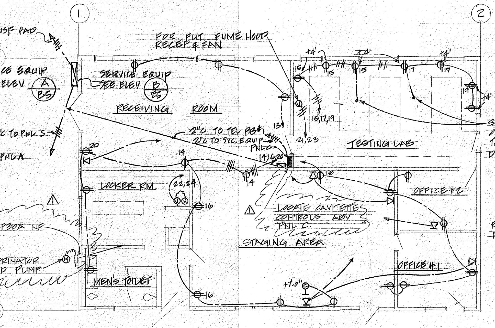
ALT. #4 - POWER & SIGNAL PLAN - BLDG. C (STATE) SCALE: 1/8"=1'-0"
