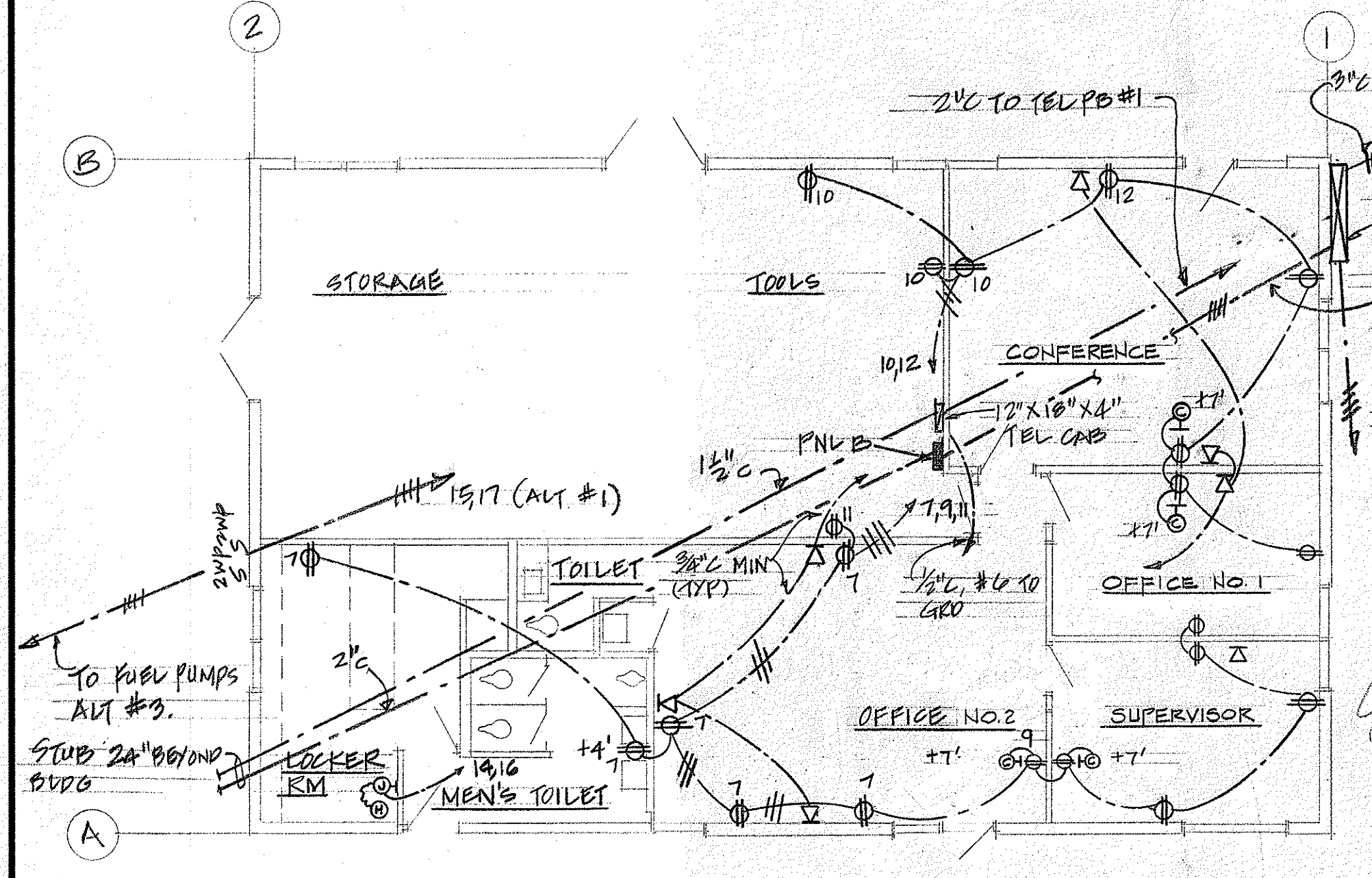
ALT. #1 - POWER & SIGNAL PLAN - BLDG. B (COUNTY) SCALE: 1/8"=1'-0"
