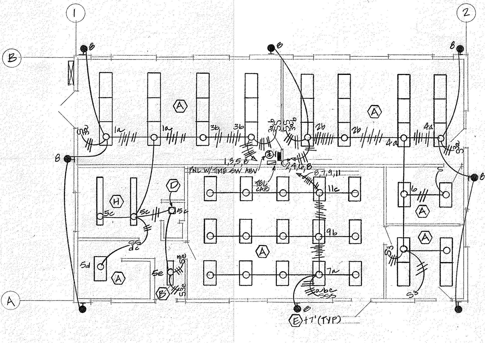
ALT. #4 - LIGHTING PLAN - BLDG. C (STATE) SCALE: 1/8"=1'-0"
