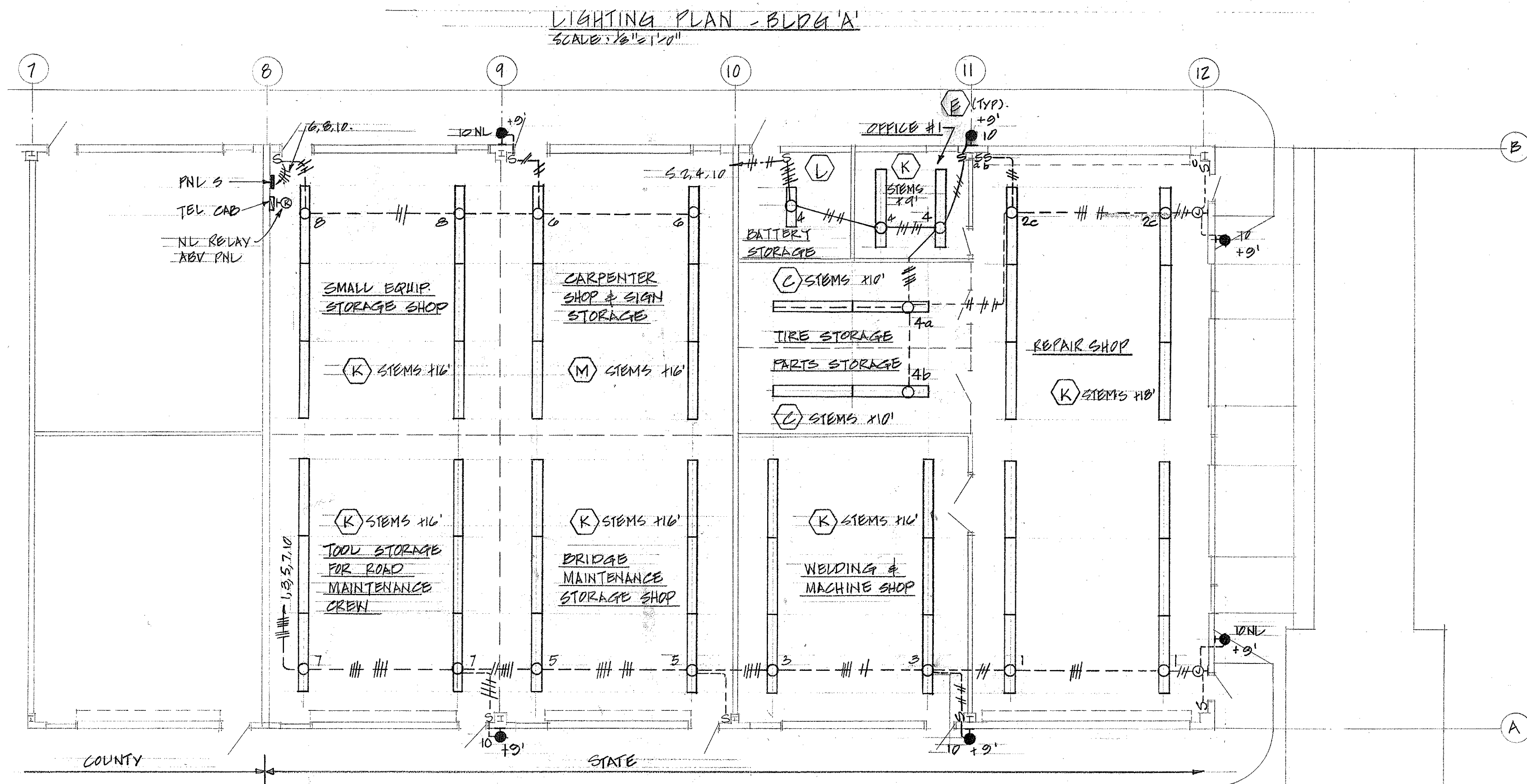
LIGHTING PLAN - BLDG 'A'
