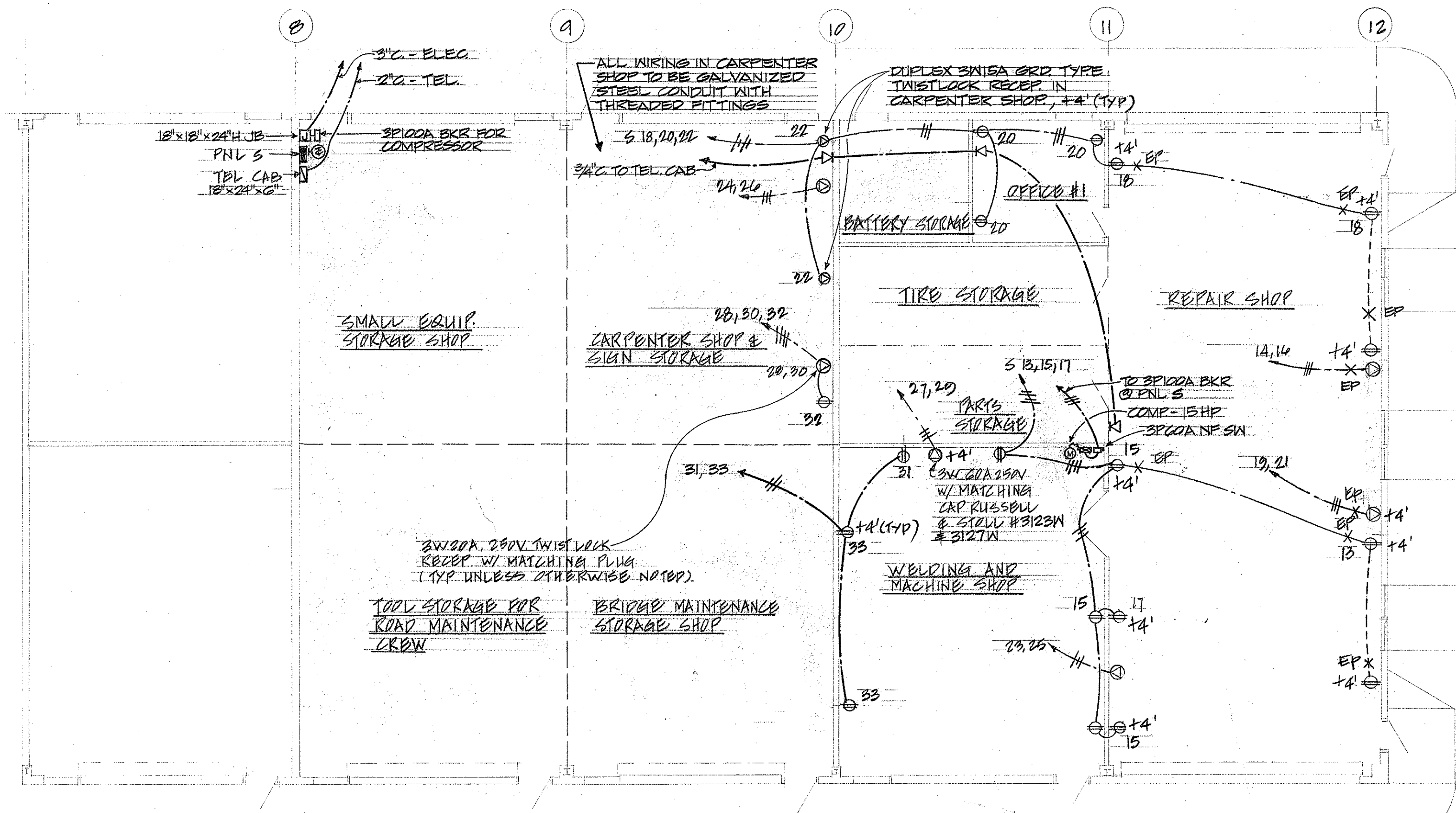
POWER & SIGNAL FLOOR PLAN - BLDG A' (STATE) SCALE: 1/8" = 1'-0"
