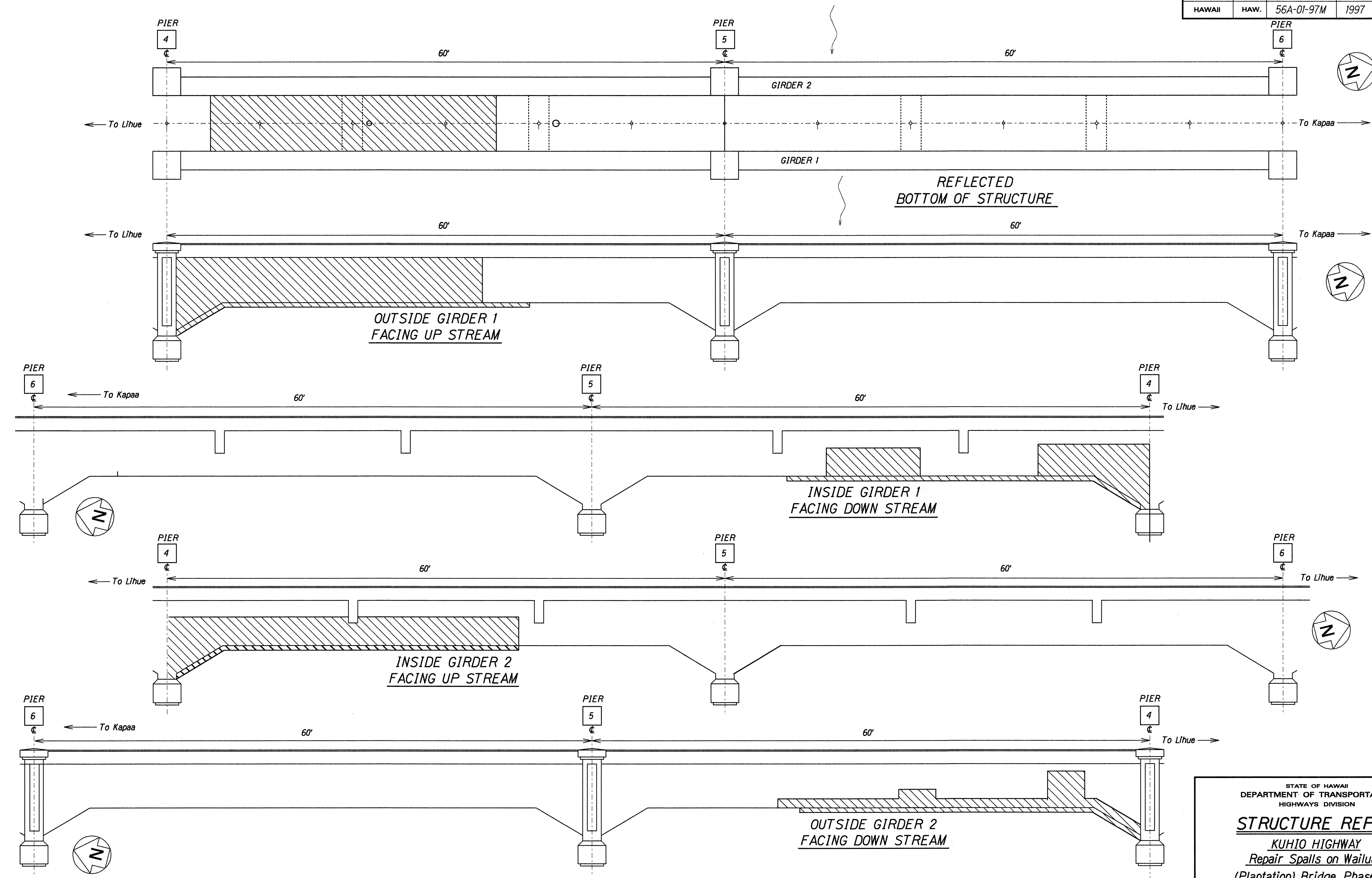
WAILUA (PLANTATION) BRIDGE REPAIR Scale: 1"=5'
