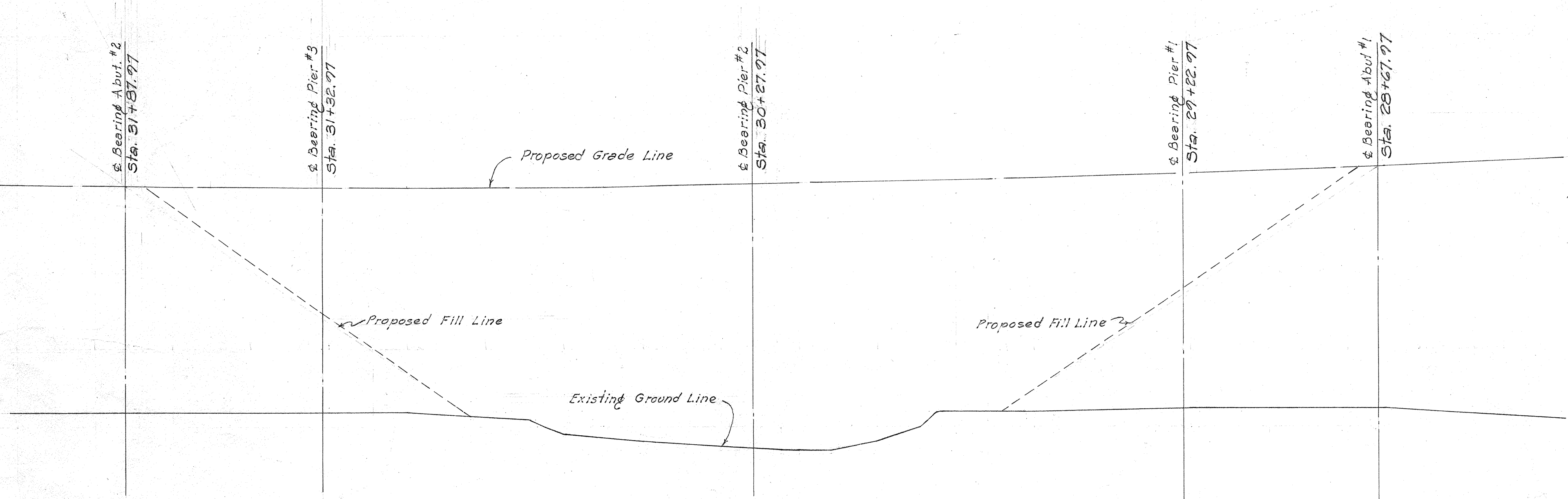
STREAM SECTION @ ROADWAY Scale: 1" = 20'-0"
