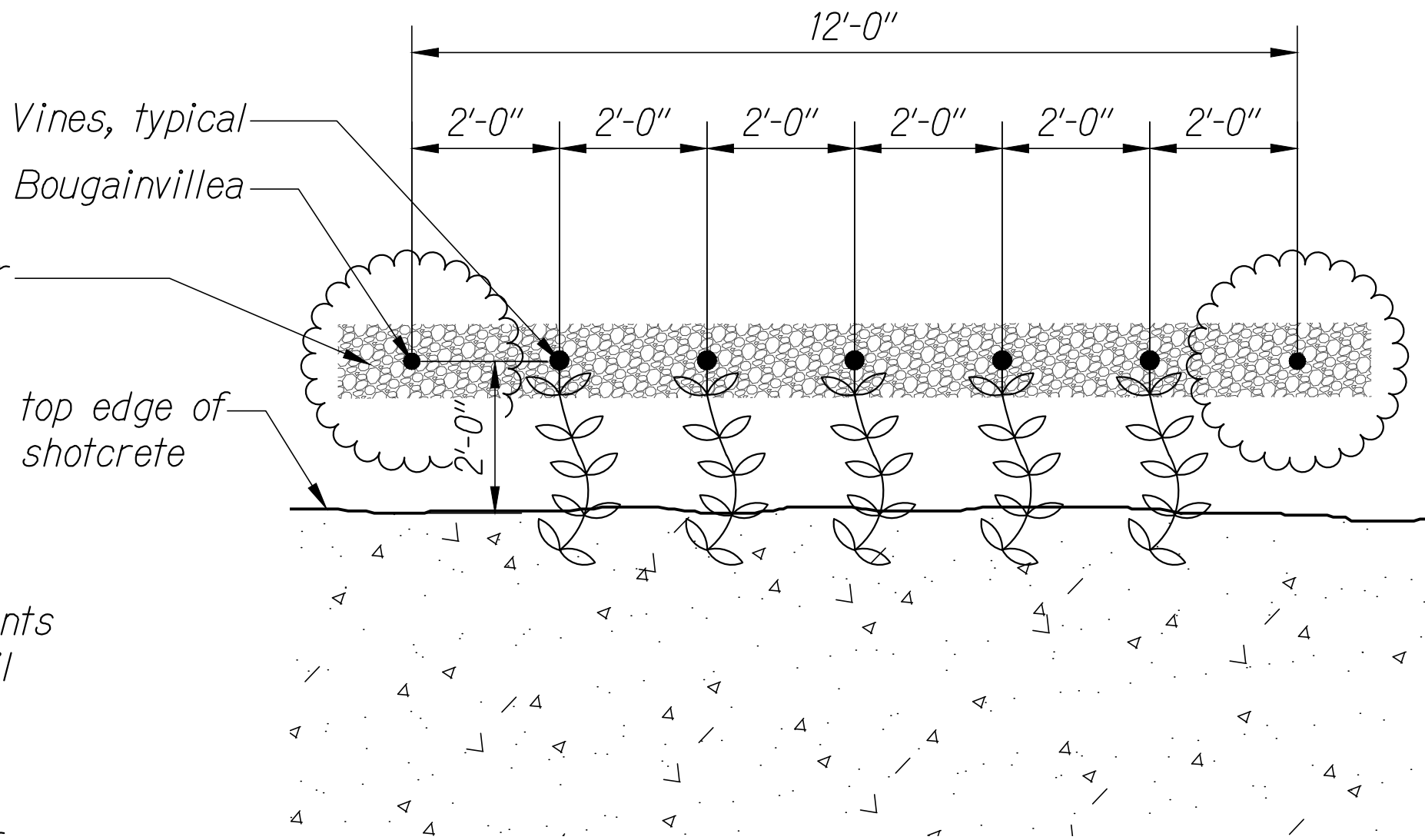
② VINE SPACING DETAIL SCALE: 1/2" = 1'-0"
