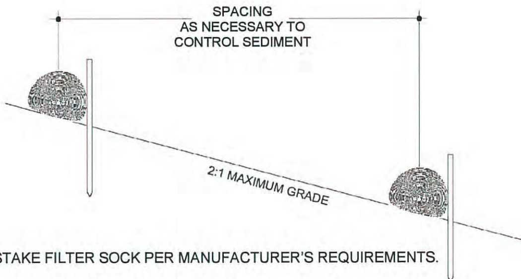
SECTION NTS
