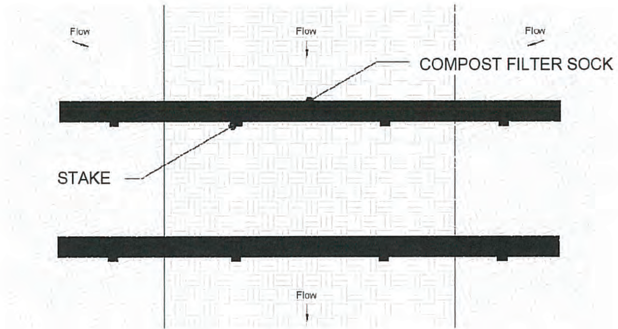
PLAN NTS
