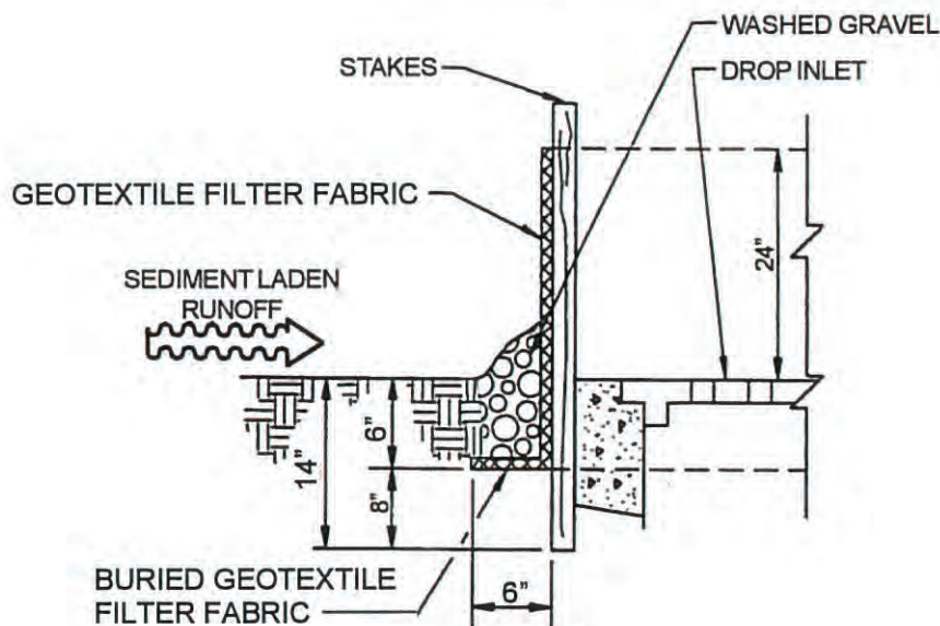
SECTION NTS
