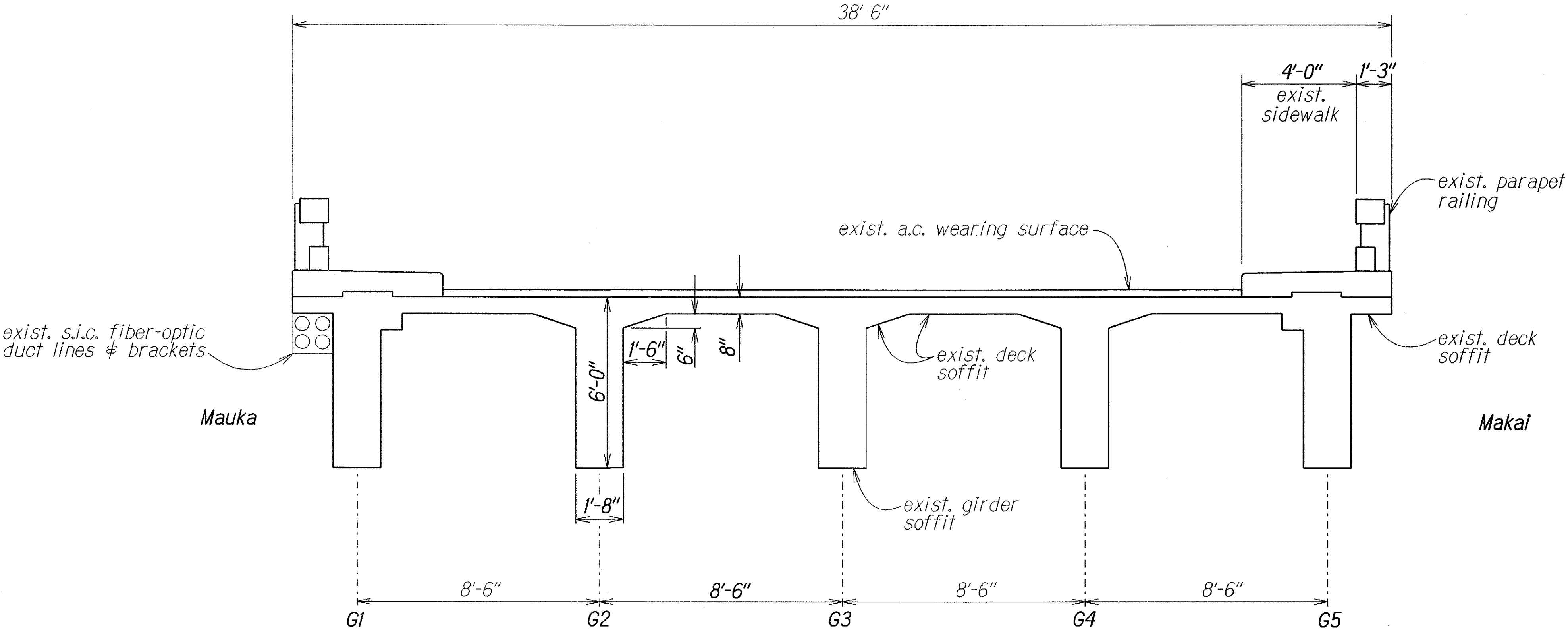
TYPICAL BRIDGE DECK SECTION - LOOKING TOWARD HANAIEI Scale: 3/8"=1'
