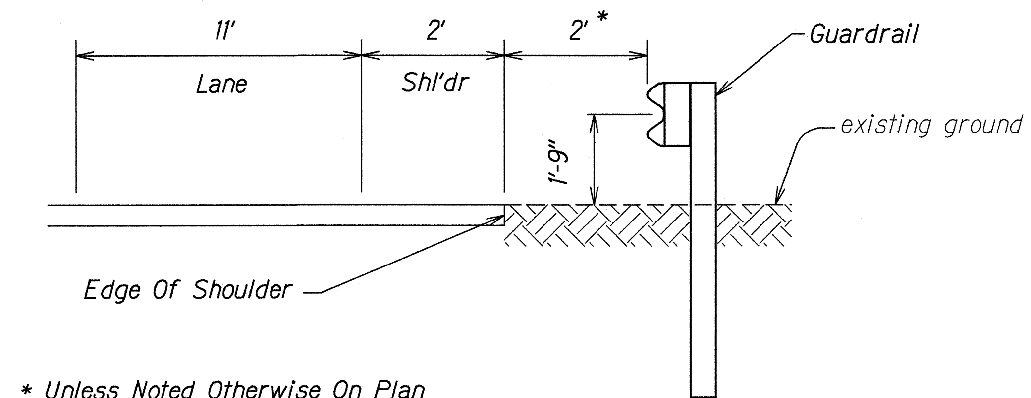
TYPICAL GUARDRAIL INSTALLATION Not To Scale
