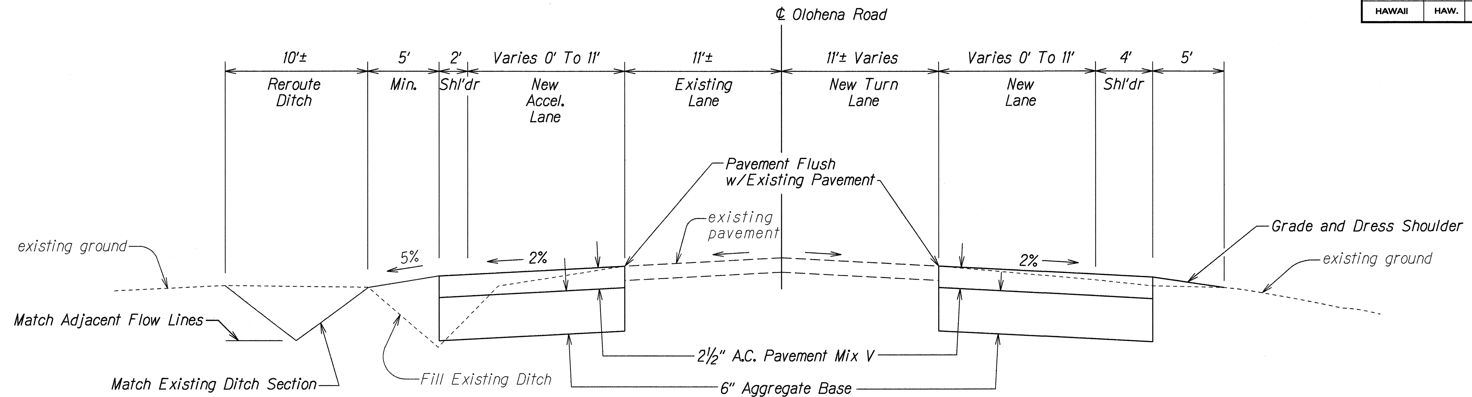
TYPICAL SECTION OLOHENA ROAD Sta. 6+00 To 10+00 Not To Scale
