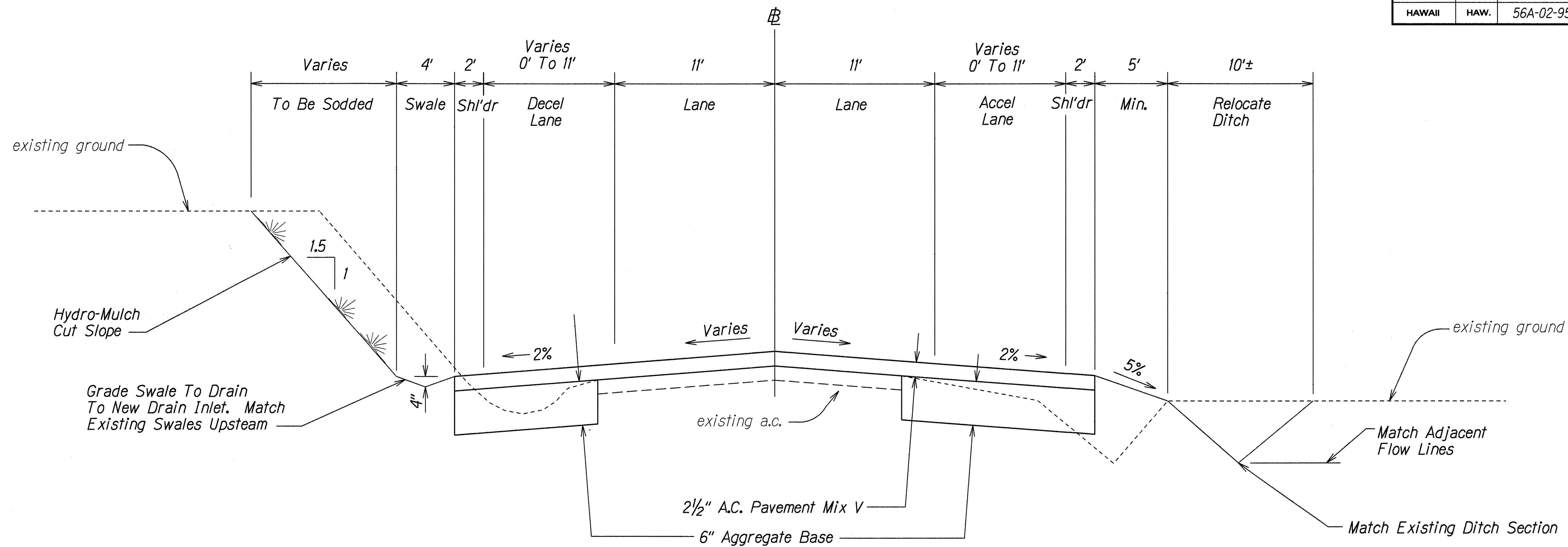
TYPICAL SECTION Sta. 121+70 To End Not To Scale
