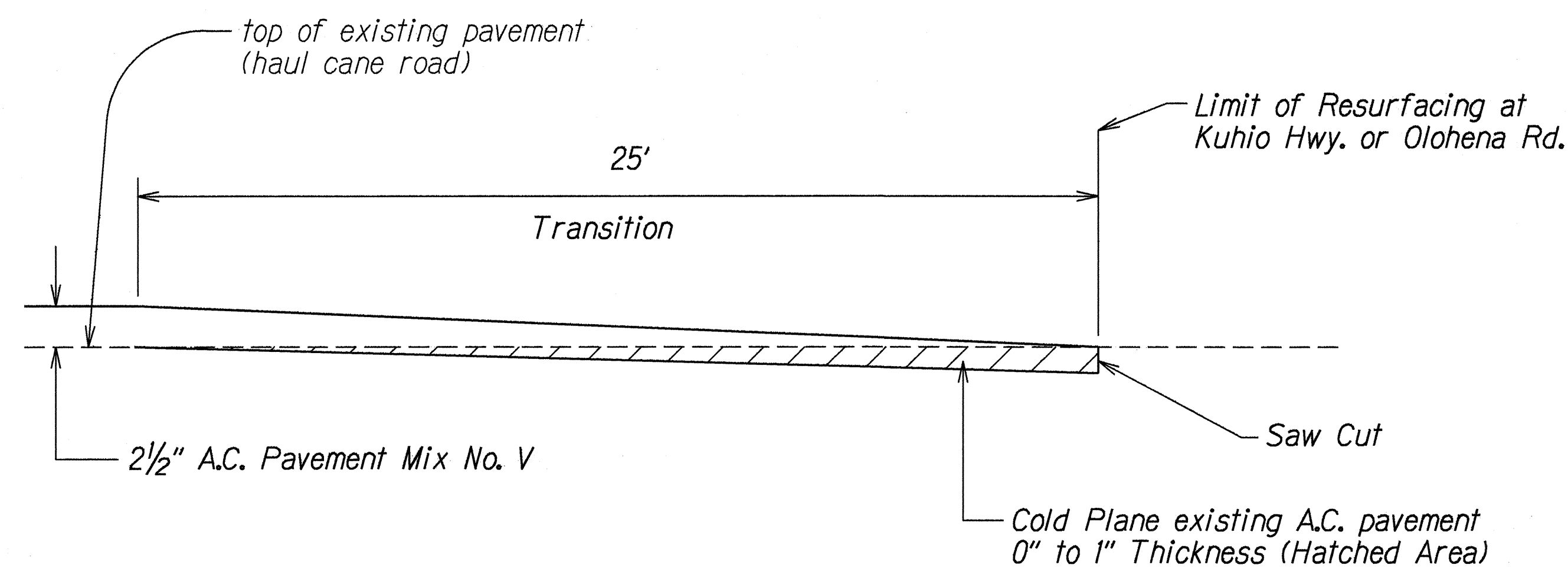
COLD PLANED TRANSITION TO EXISTING A.C. PAVEMENT Not To Scale
