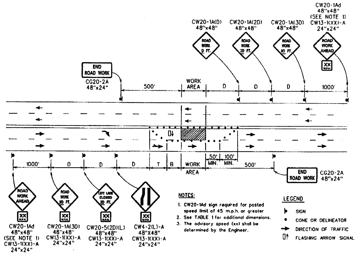
FIGURE 3 - TRAFFIC CONTROL PLAN
