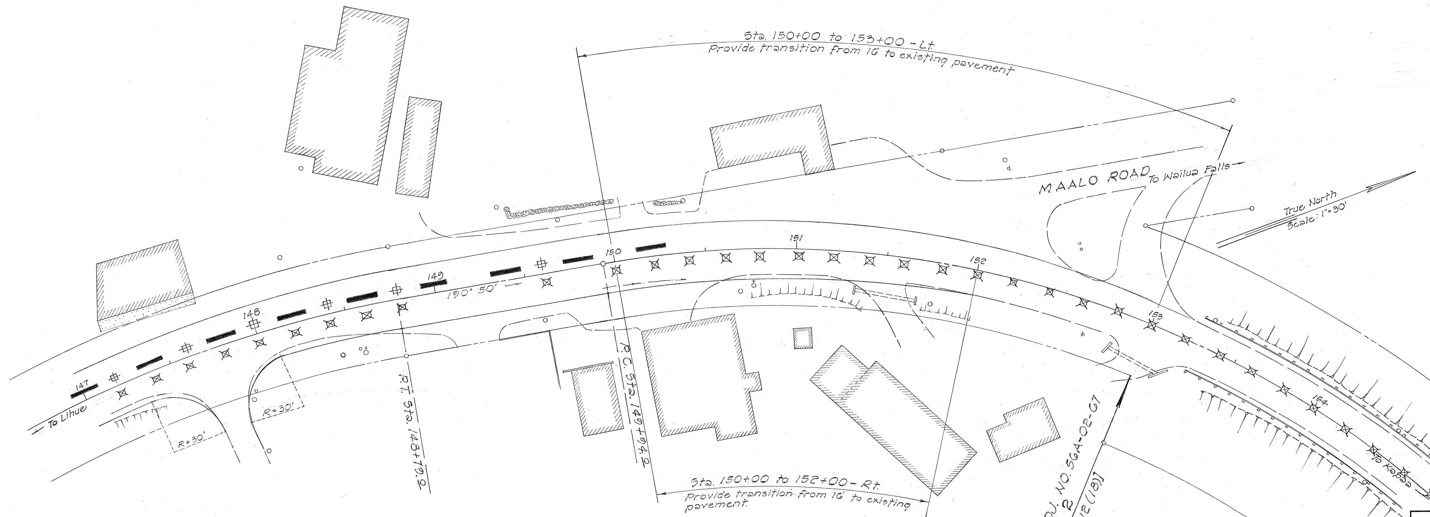
PLAN SHOWING PAVEMENT MARKERS STA. 147+00 TO END OF PROJ. SCALE: 1" = 30'
