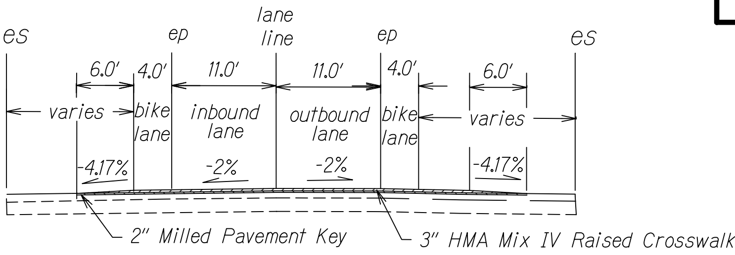
SECTION "A-A" HMA RAISED CROSSWALK Scale: 1"=10'
