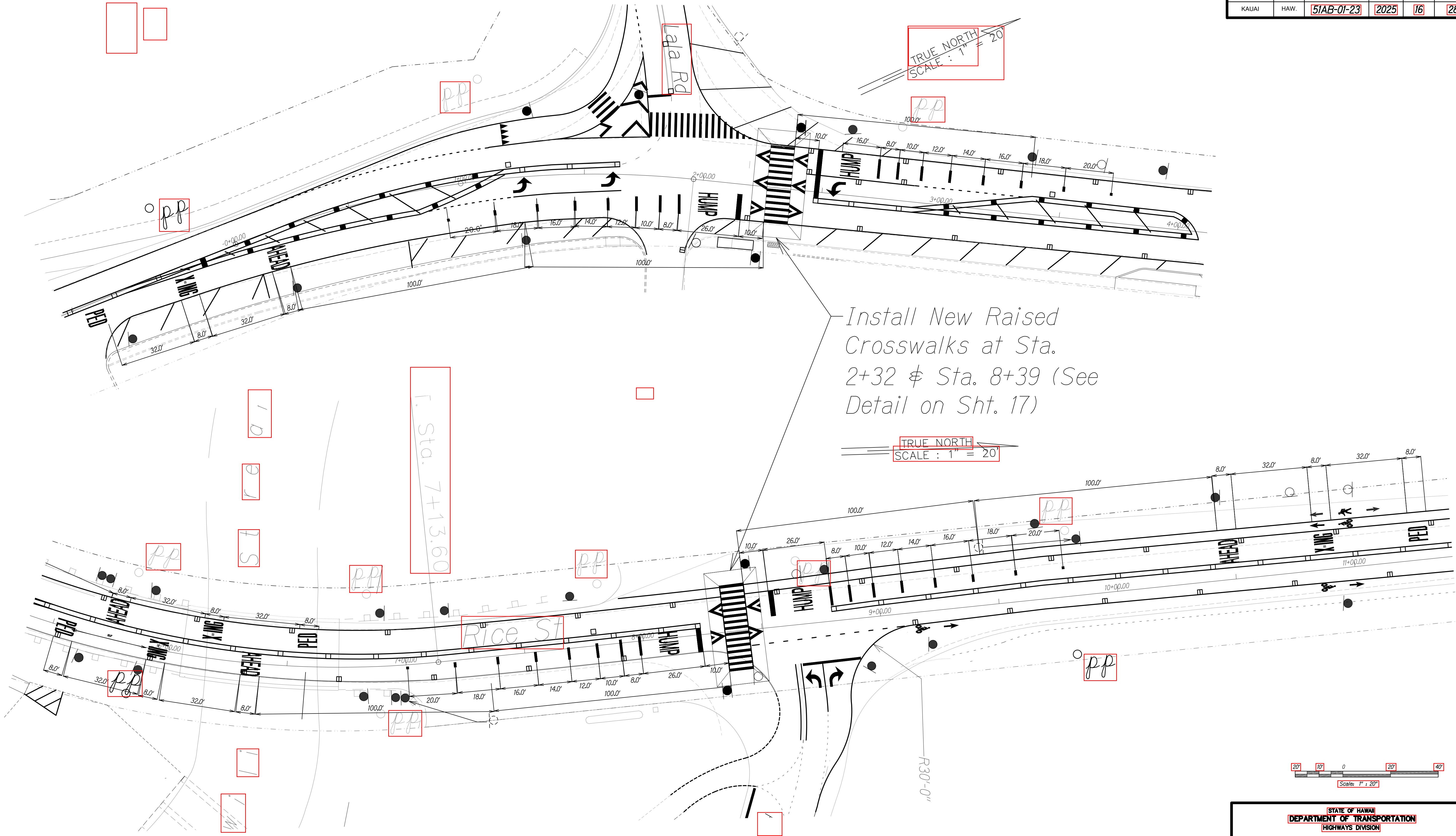
RAISED CROSSWALK ENLARGE PLANS Scale: 1" : 20'
