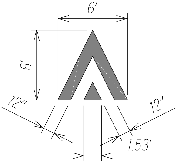
RAISED CROSSWALK MARKINGS Scale: 1"=5'
