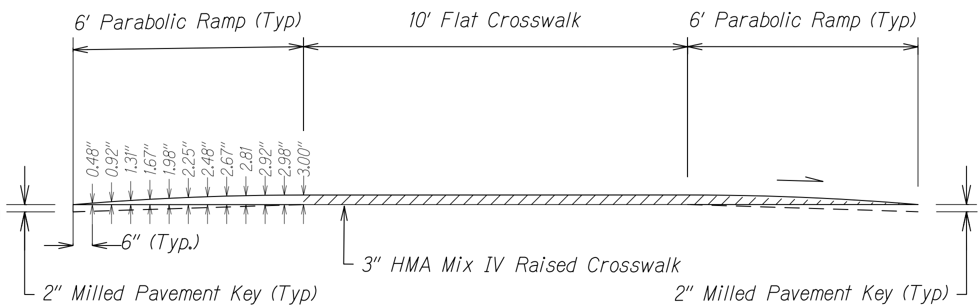
SECTION "B-B" HMA RAISED CROSSWALK Scale: 1"=2.5'
