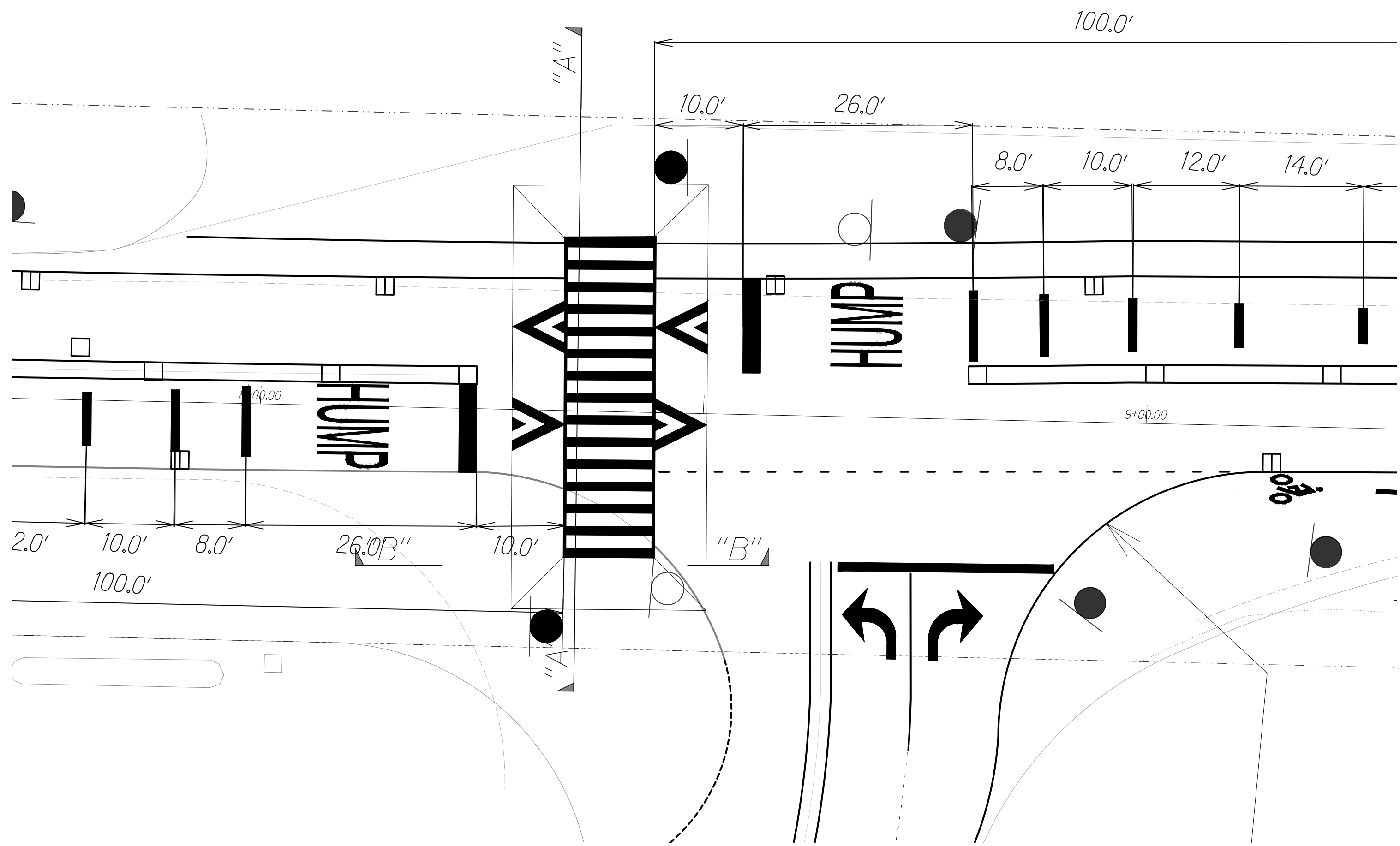
HMA RAISED CROSSWALK Scale: 1" = 10'
