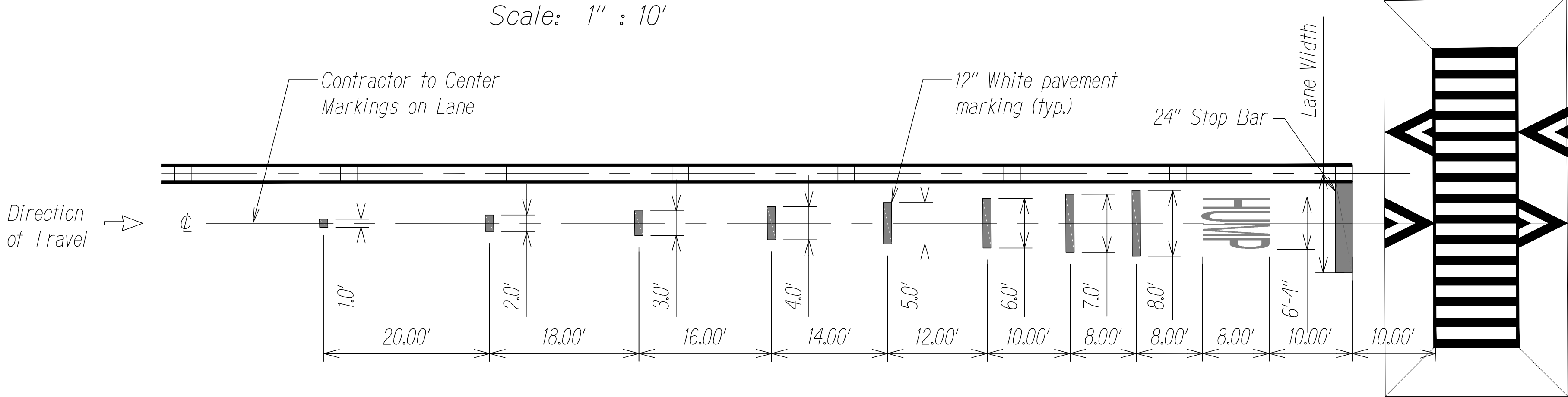
SPEED HUMP ADVANCE WARNING MARKINGS DETAIL Scale: 1"=10'
