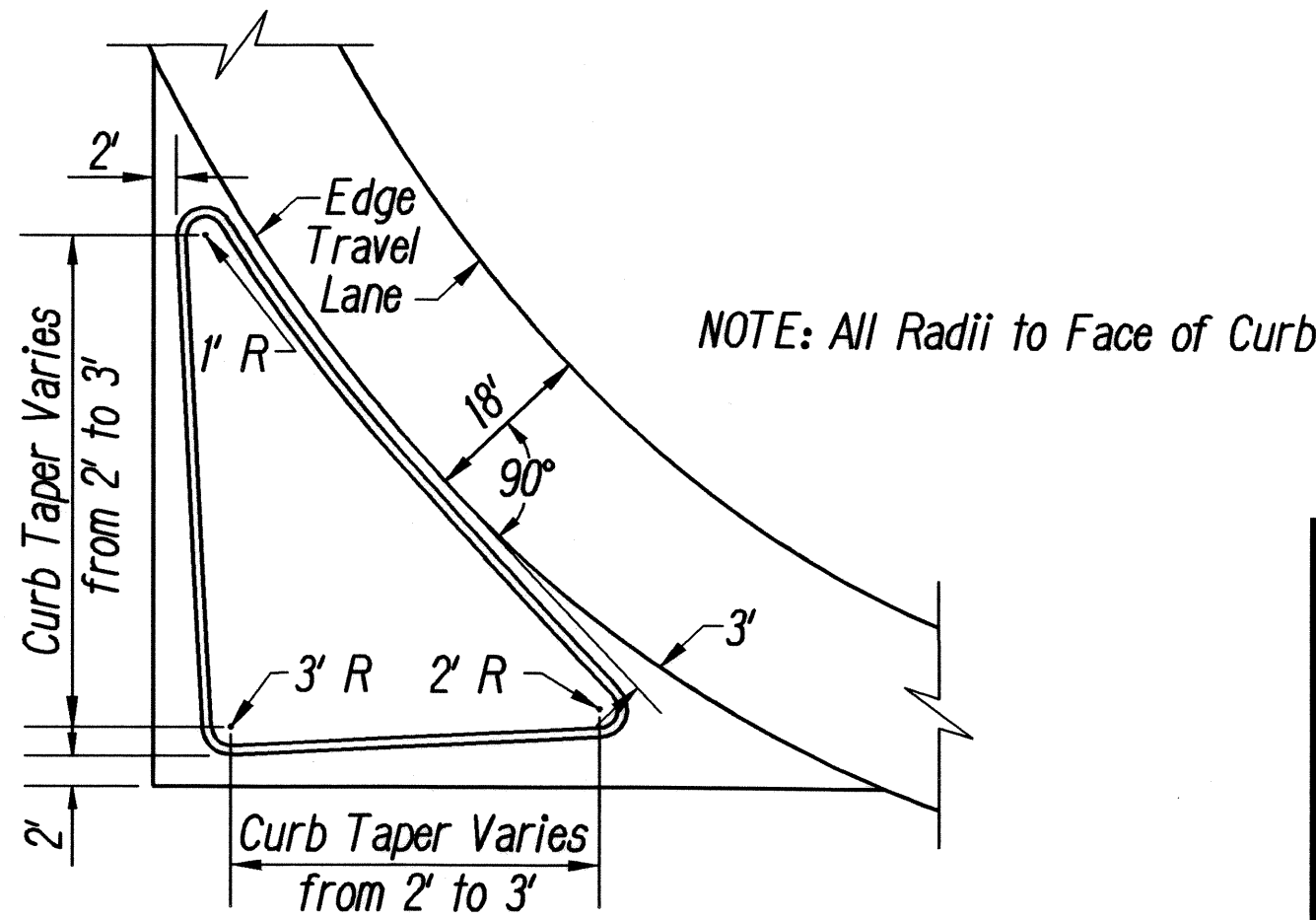
TYPICAL A.C. CURBED ISLAND LAYOUT Not to Scale
