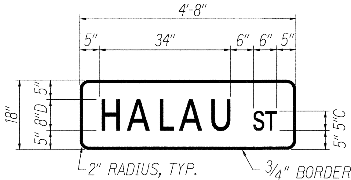
STREET NAME SIGN DETAIL
