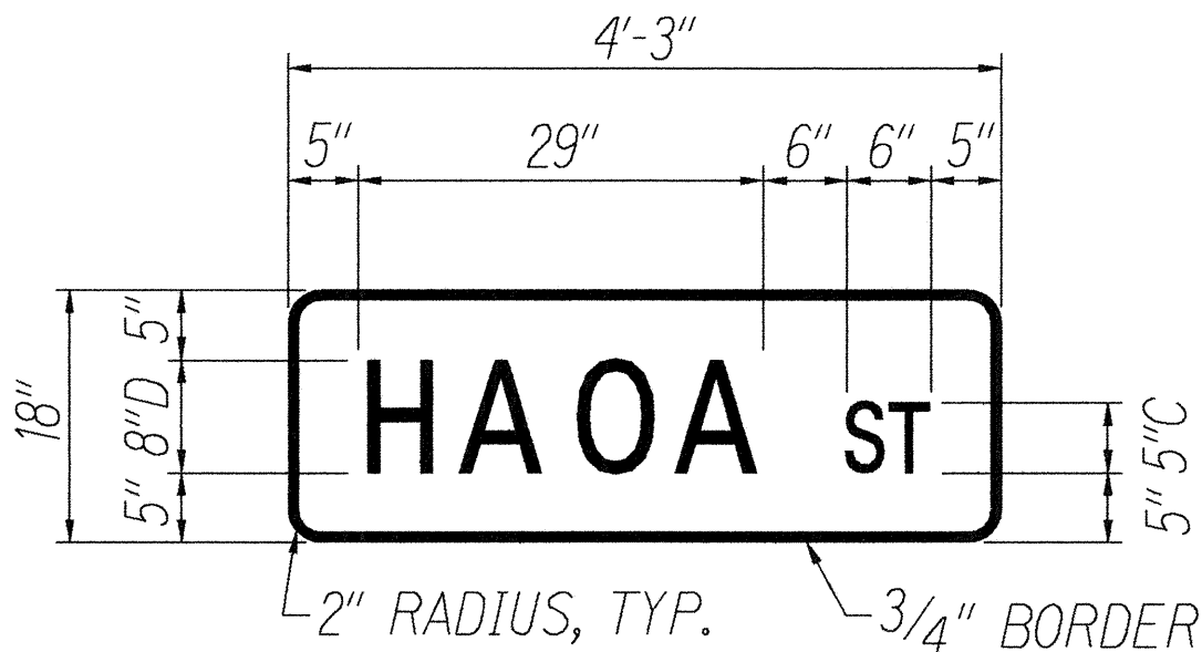
STREET NAME SIGN DETAIL
