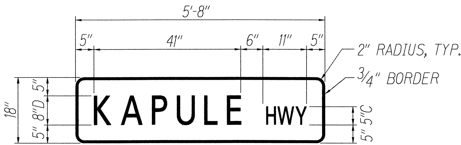
STREET NAME SIGN DETAIL
