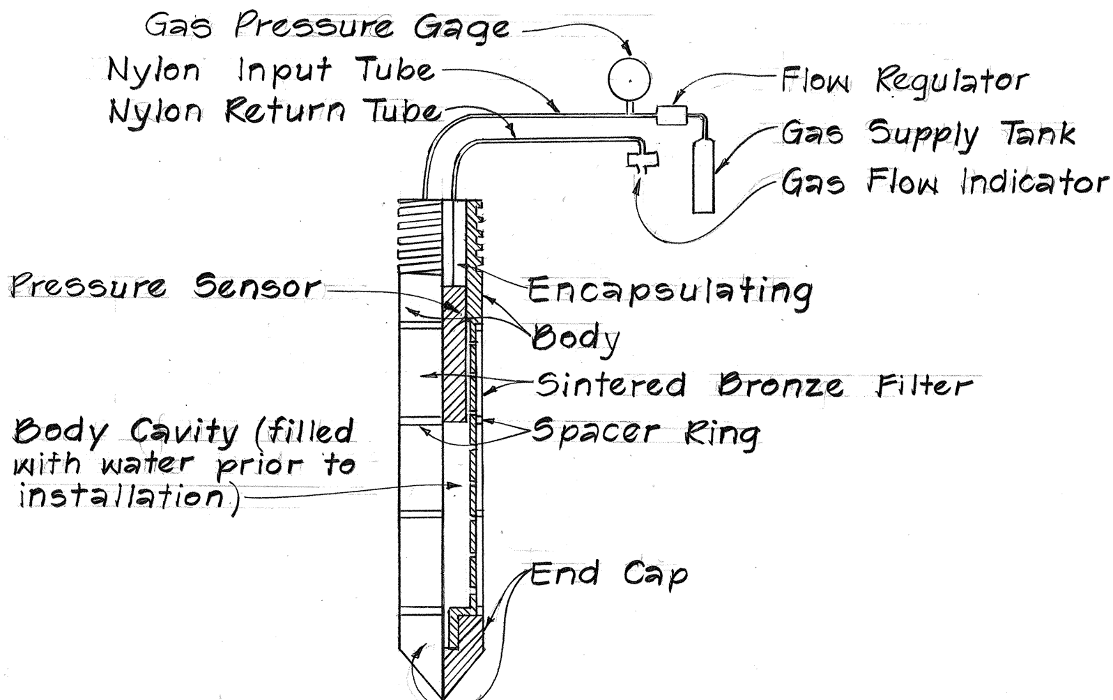
CROSS SECTION OF COMPLETE PIEZOMETER SCALE: Not to Scale
