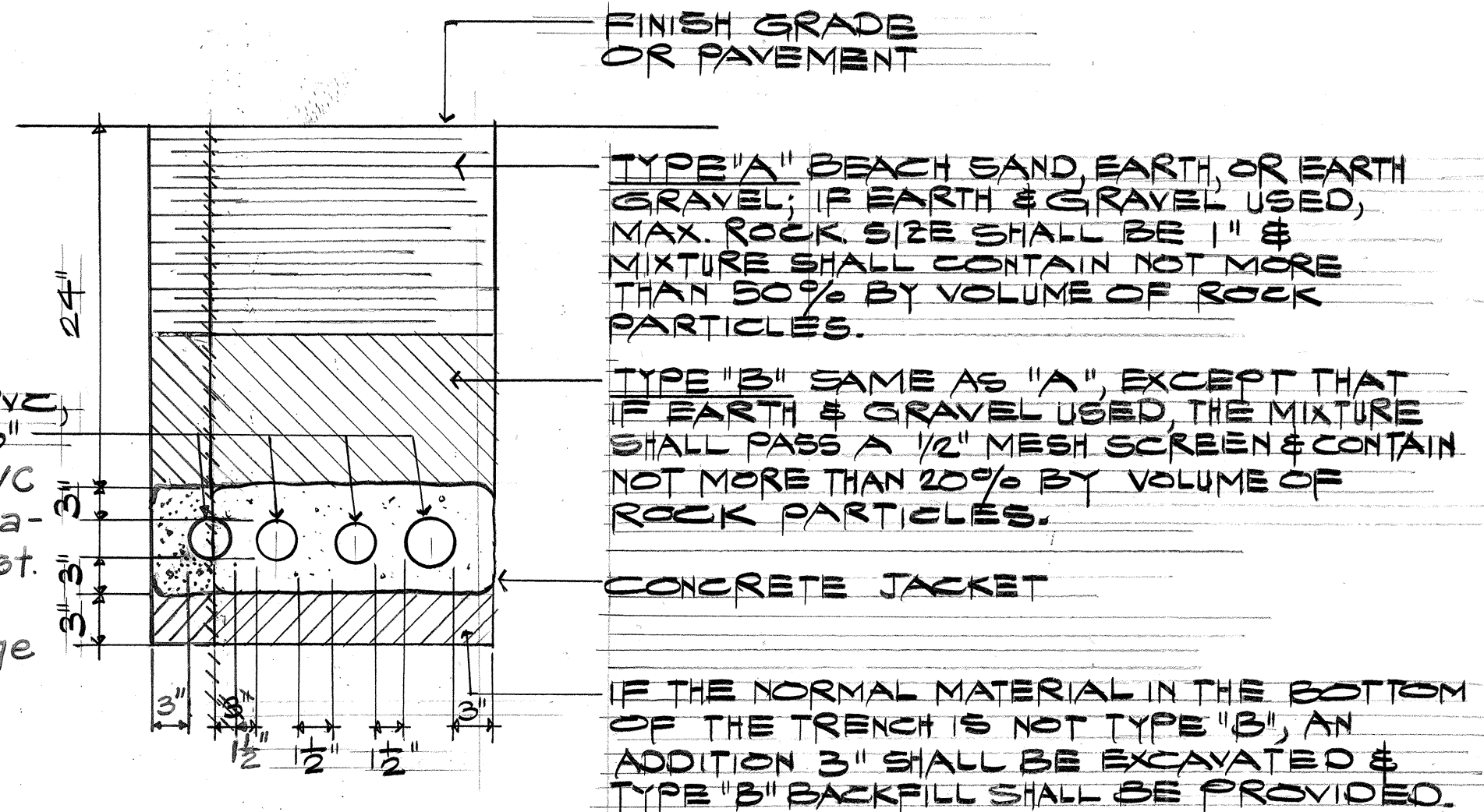
TYP. DUCT SECTION NTS
