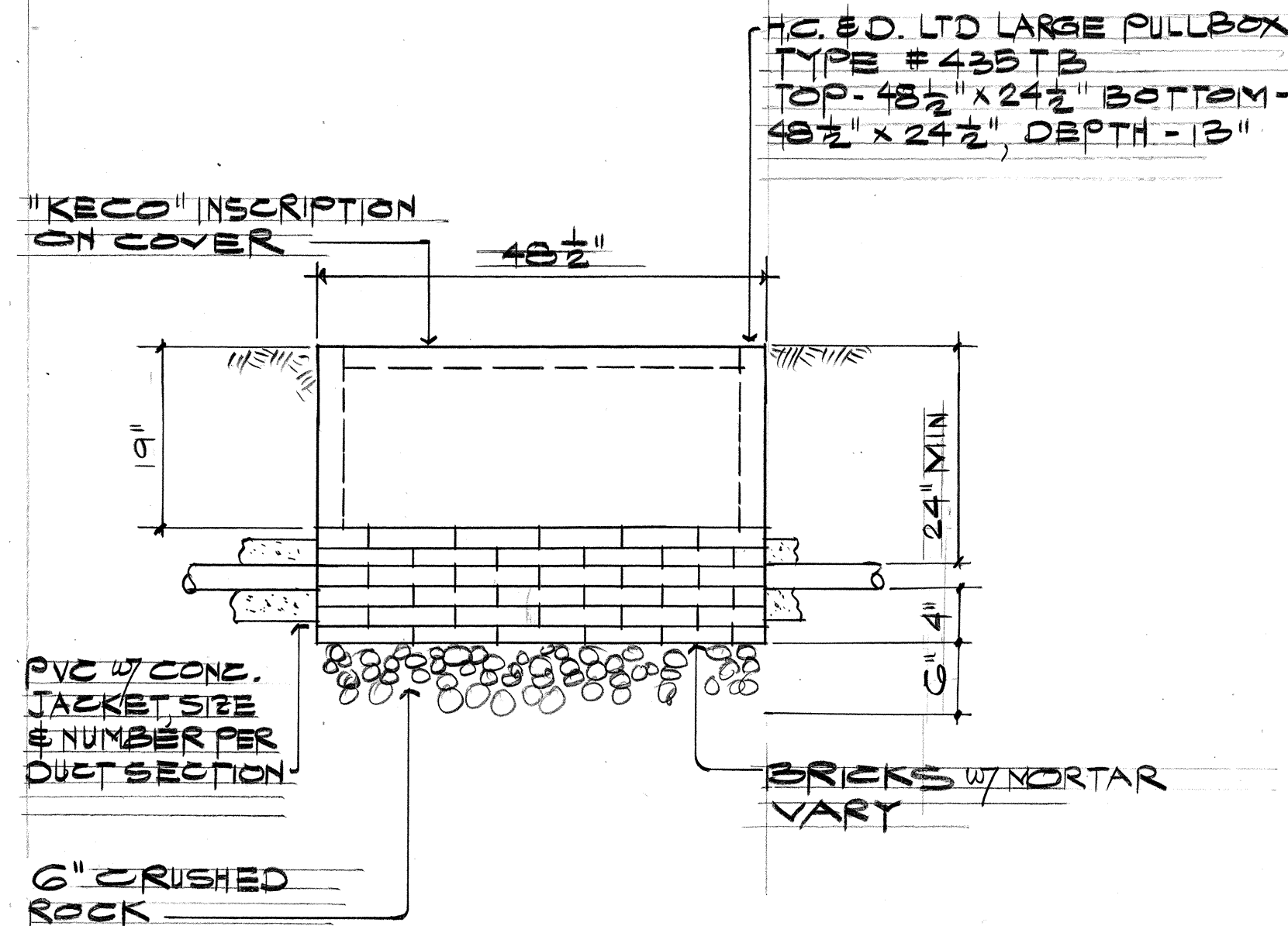
PULL BOX DETAIL NTS
