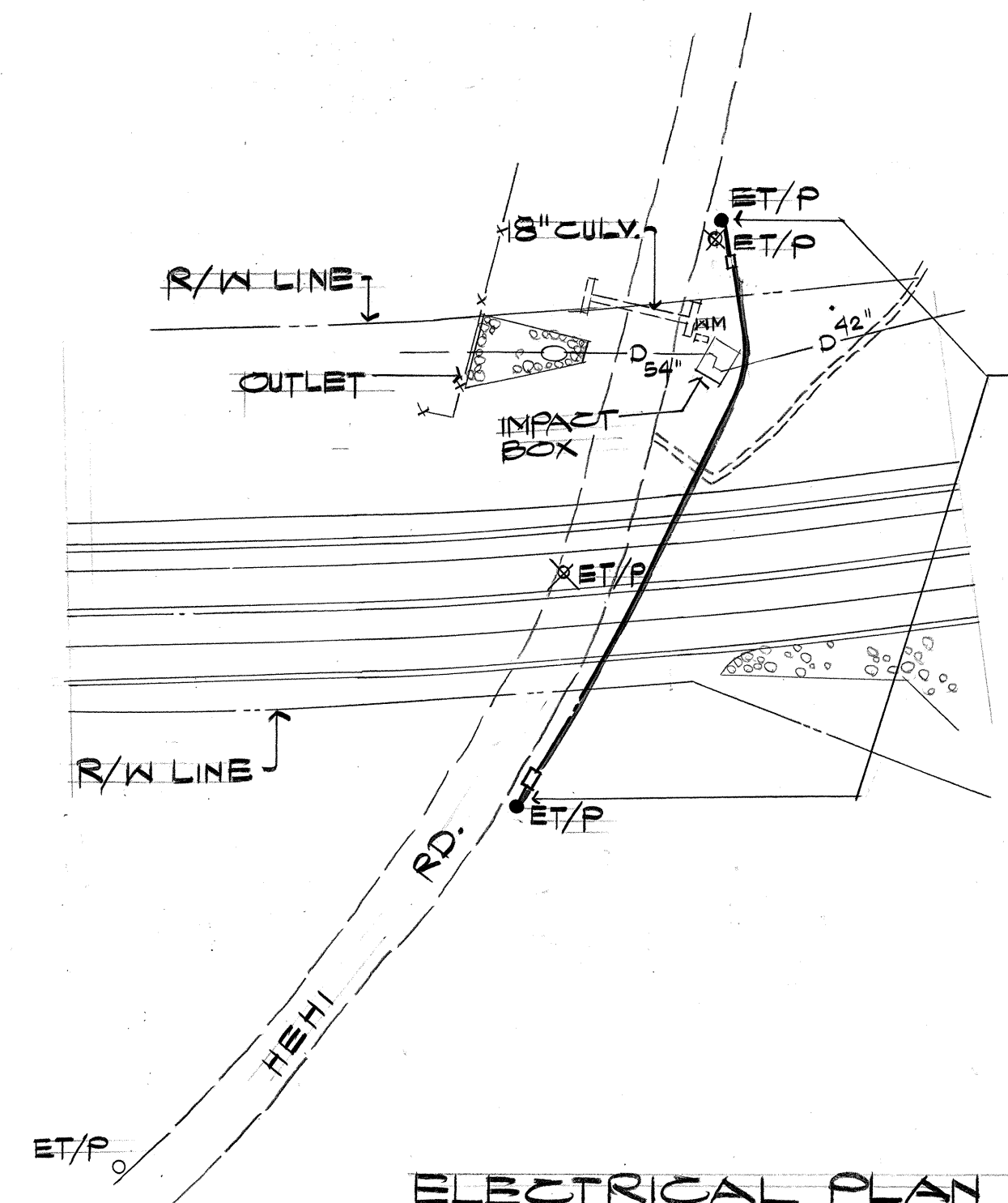
ELECTRICAL PLAN SCALE: 1" = 50'
