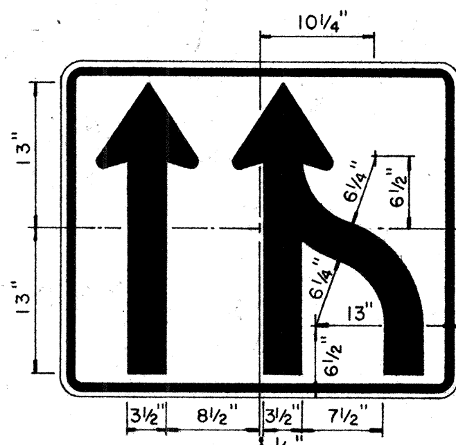
R3-10 36" x 30"
