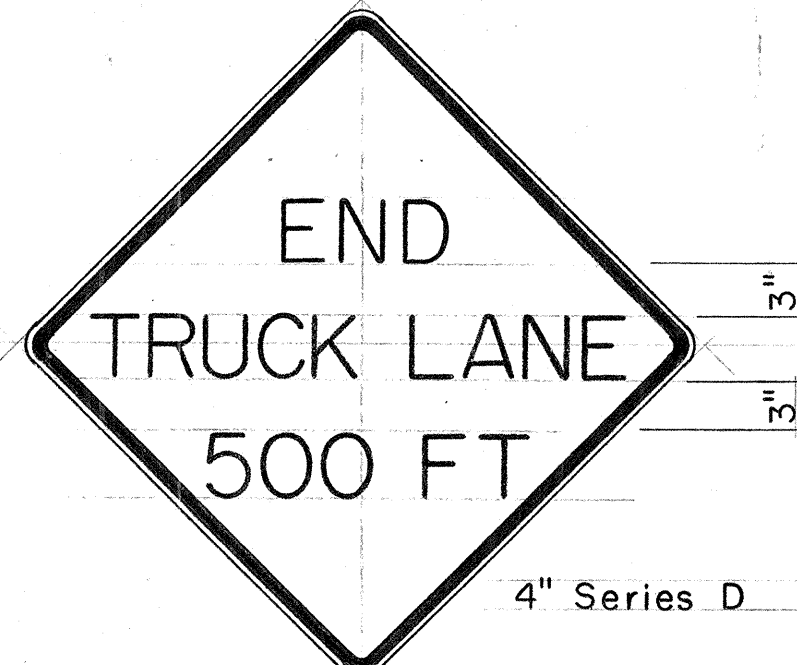
W6-3 30" x 30"
