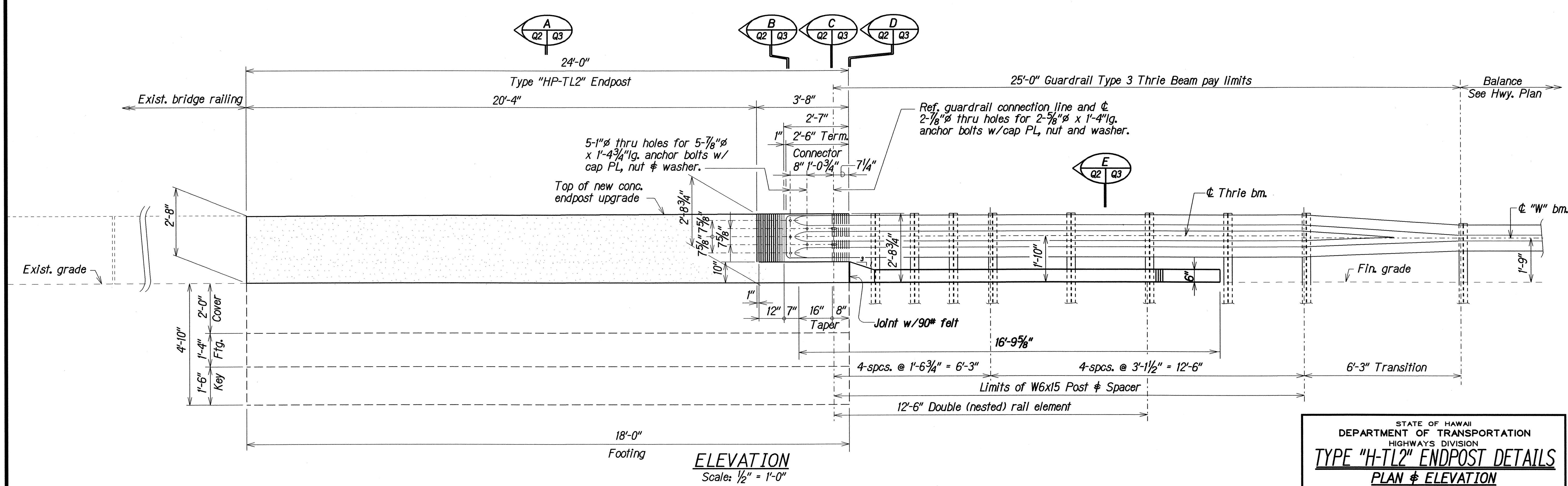
TYPE "HP-TL2" ENDPOST PLAN AND ELEVATION
