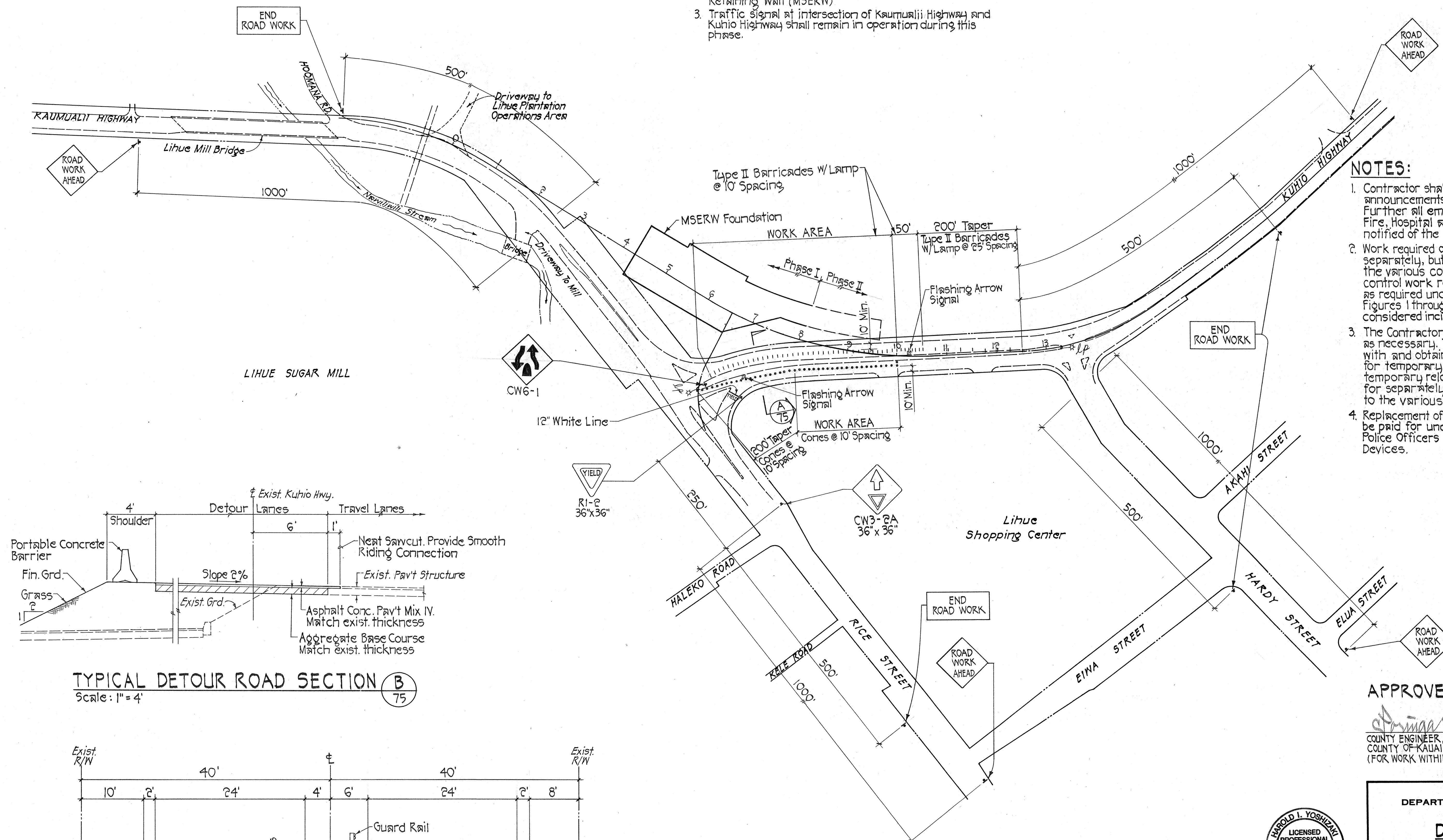
DETOUR PLAN~PHASE I Scale: 1" = 100'
