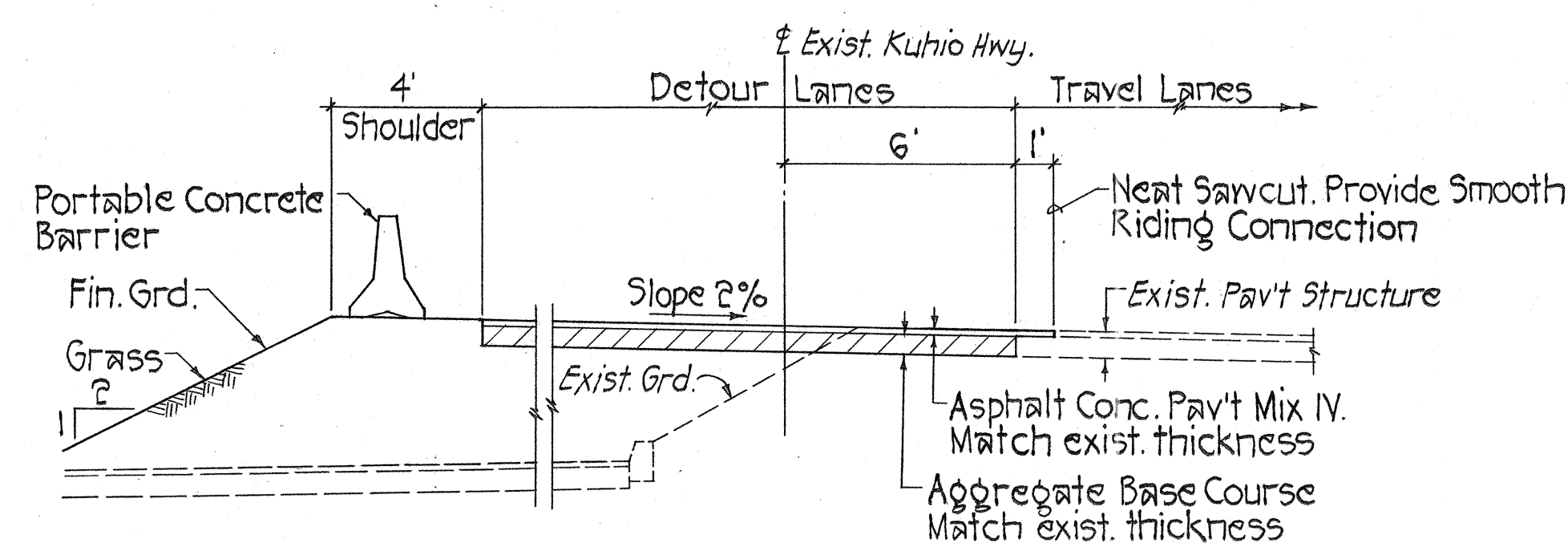
TYPICAL DETOUR ROAD SECTION B Scale: 1" = 4'
