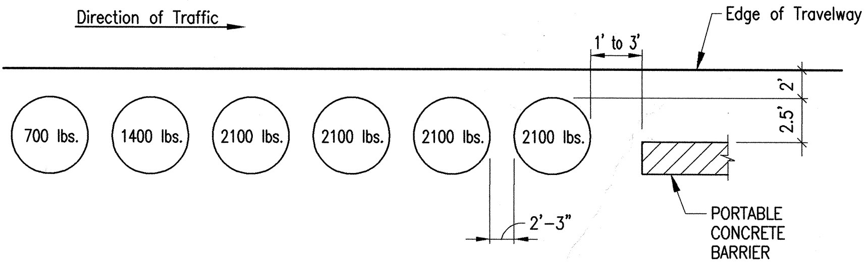
INERTIAL BARRIER DETAIL A NOT TO SCALE 79
