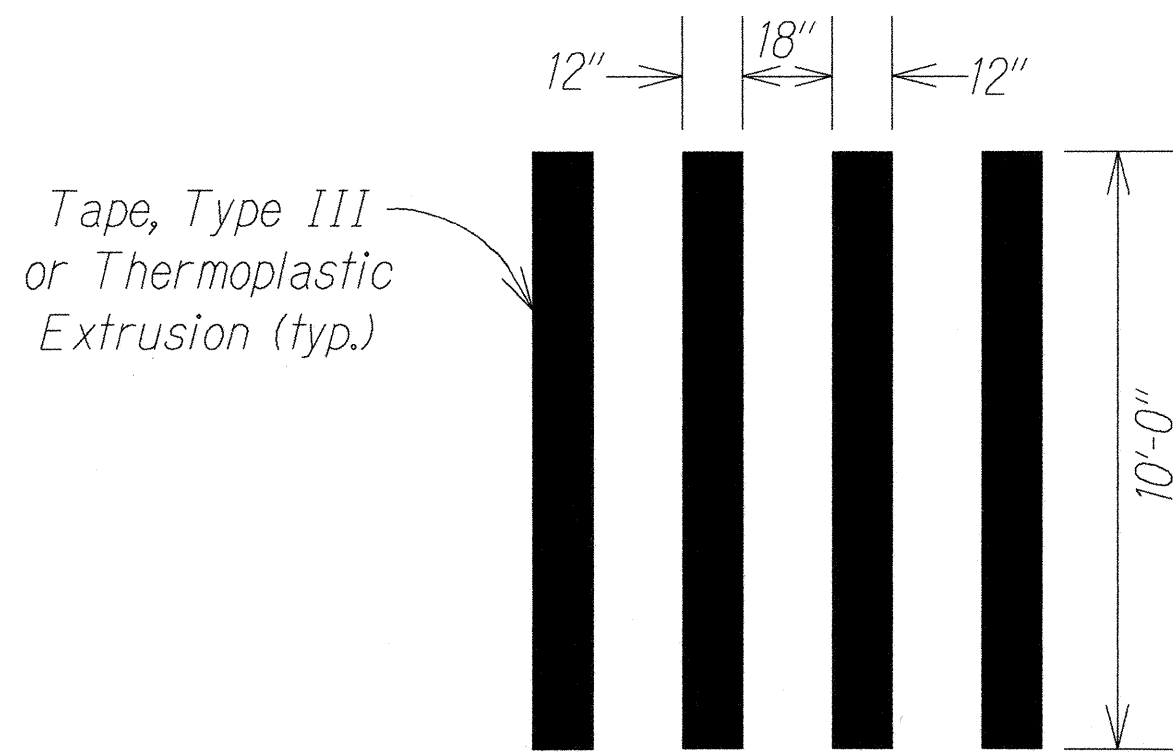
TYPICAL CROSSWALK DETAIL Not to Scale
